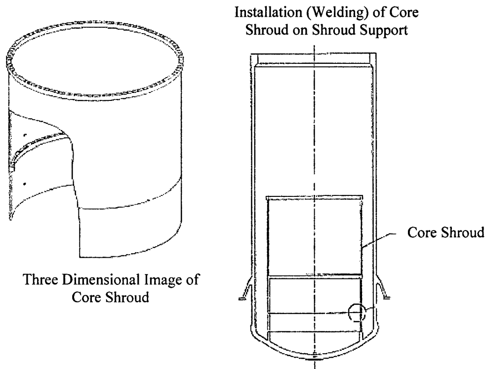
Figure 3.1.1-1 RPV and Core Shroud Assembly (Taken from Reference 3-2)
