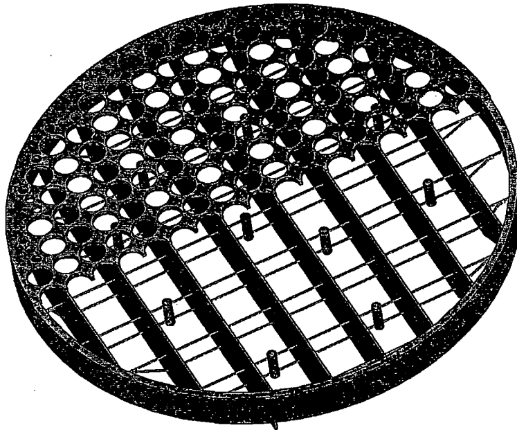
Figure 3.1.4-1 Core Plate
