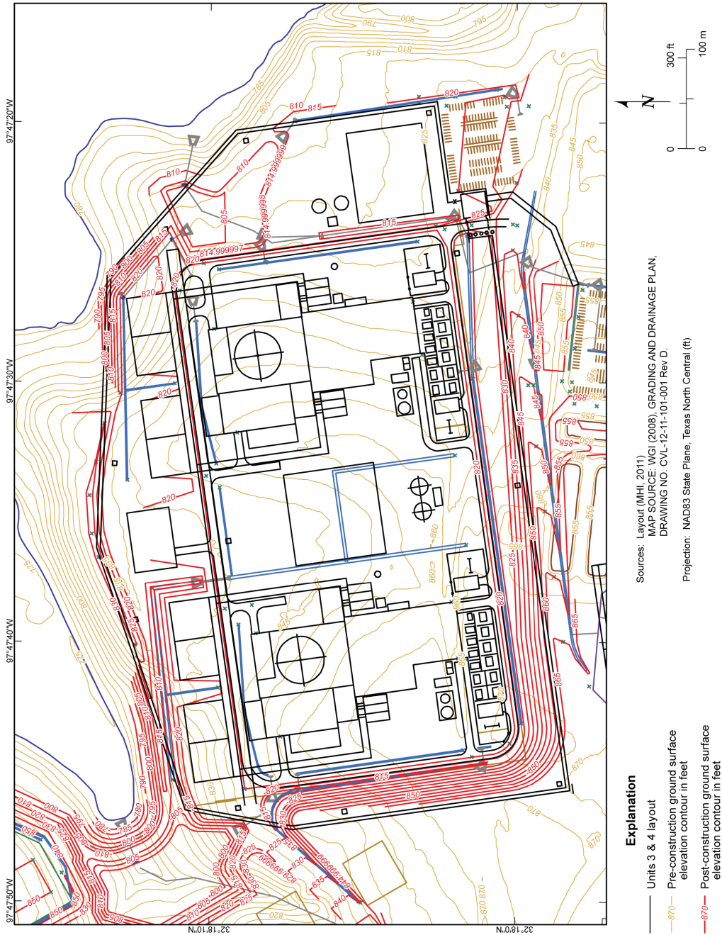
Figure 2.5.5-204 Site Grading Map
