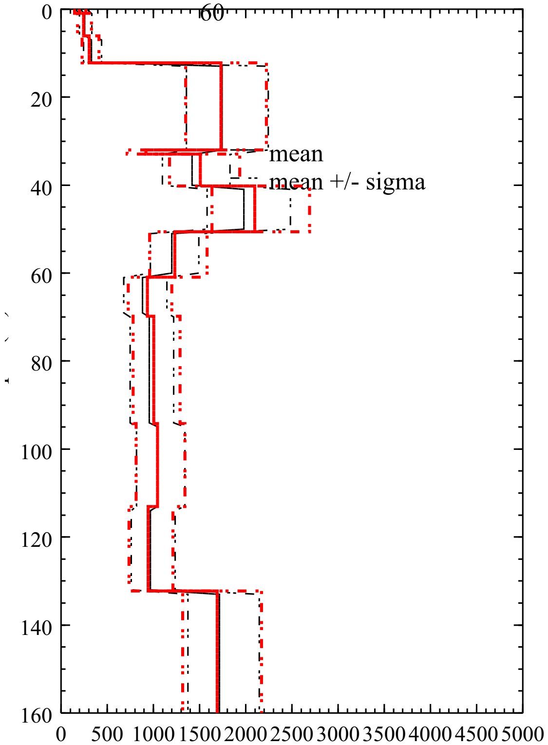
Figure 2.5.2-243 Summary Statistics from Synthetic Profiles for the Top Portion of the FIRS4 Site Column Compared to Values in Table 2.5.2-227
