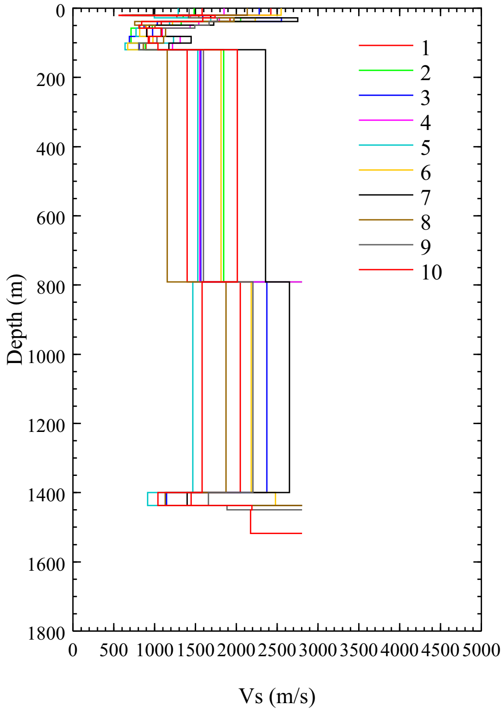
Figure 2.5.2-240 Graph of Velocity vs. Depth for the First 10 Synthetic Profiles Generated for the GMRS/FIRS1 Site Column
