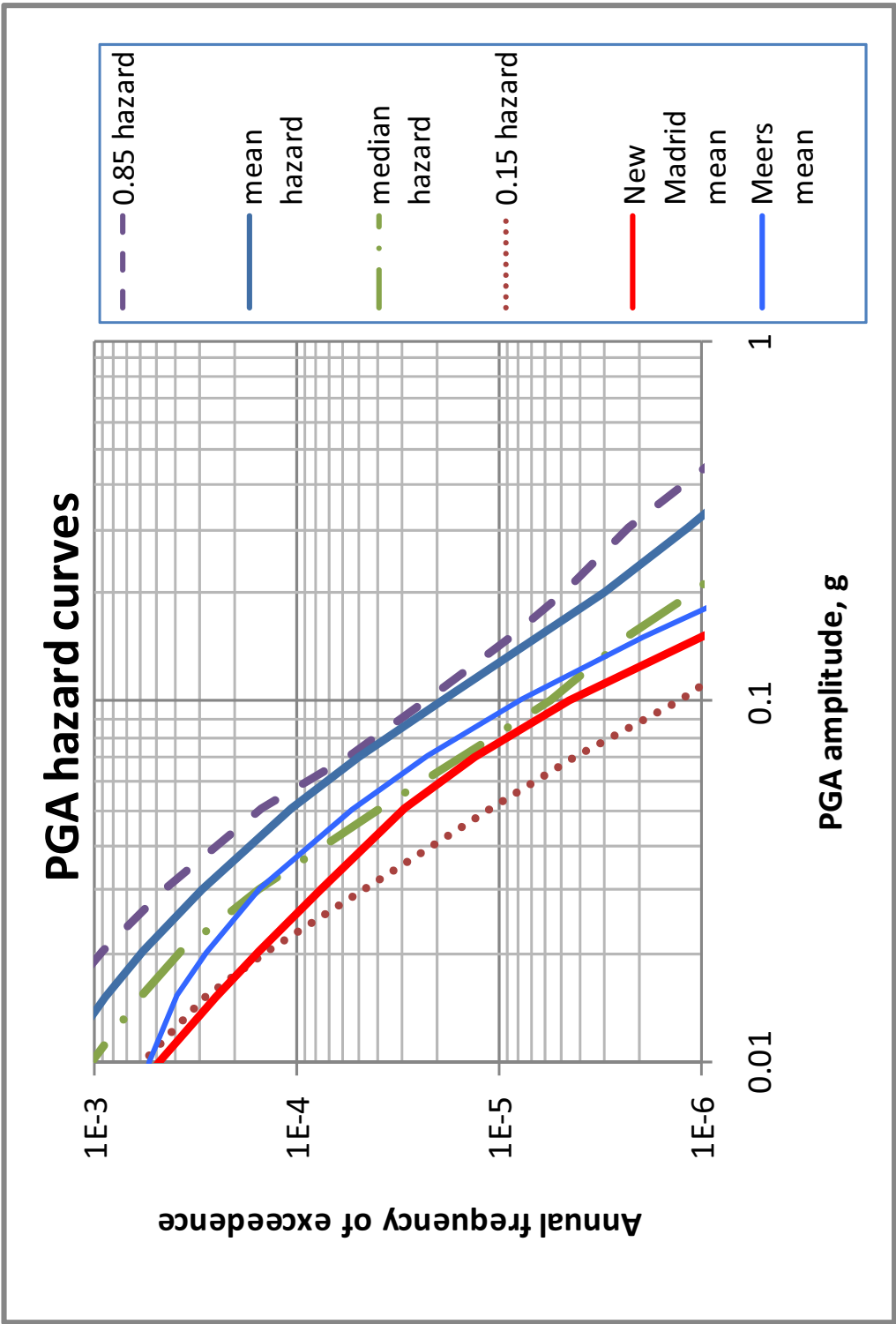
Figure 2.5.2-215 PGA Rock Seismic Hazard Curves for all Sources and for New Madrid Faults Alone
