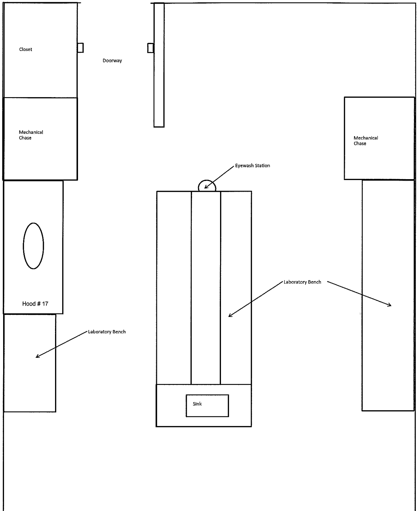
Floor Plan Room 1221
