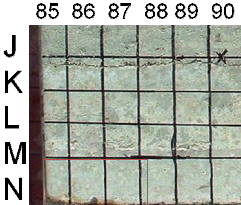
Figure 2-16. Photograph of Section Three Grout, Which Was Predicted by Ultrasonics To Have Air Gaps. Lift 1 Is Smoother Than Lifts 2 and 3, and Ultrasonics Indicated That the Outlined Area, Which Is Smooth, Was Free From Air Gaps. Evidence of Preexisting Grout Spatters From Prior Pours Is Observed Above This Level.
