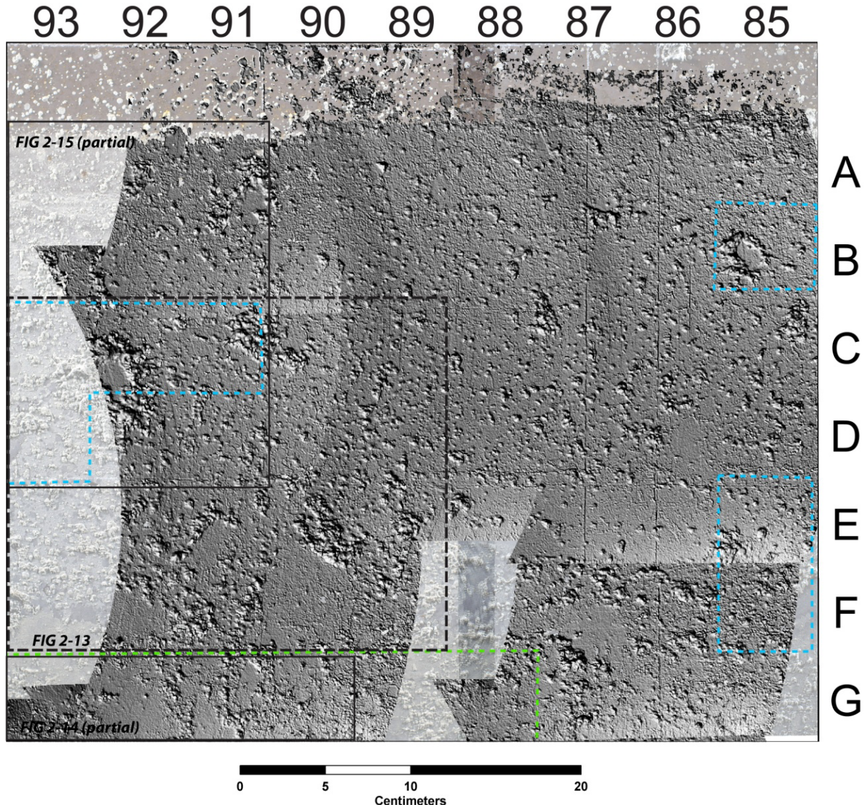
Figure 2-18(a). DSR Mosaic of a Portion of the Interior Surface of the Section Three Wall. Areas of no Data Show a Semi-Transparent Version of the Photomosaic Shown in Figure 2-18(b). Figure 2-18(a) Incorporates the Area of Figure 2-13 (Dashed Black Line), and Portions of Figures 2-14 and 2-15 (Black Lines as Labeled). Dashed Blue Lines Encompass Areas Predicted by Ultrasonic Testing To Have Air Gaps. Dashed Green Lines Show Areas Predicted by Coin-Tap Testing To Have Air Gaps. The DSR Shows This Portion of the Tank Wall To Be Generally Rough, With Little or no Difference in Appearance Relative to Ultrasonic Testing Results. Smooth Areas Exist as Isolated Patches. Smooth Areas Appear To Be Most Common in the Lower Portion of the DSR (Rows E, F, And G). Rows A–F Show Lift 3, and Row G Shows the Uppermost Portion of Lift 2. Row G Also Contains the Only Area Predicted by the Coin-Tap Method To Have an Air Gap. The Uppermost Portion of the Image, Above Row A, Shows a Portion of the Spattered Tank Wall That Is Located Above the Surface of the Monolith [See Figure 2-18(b)].
