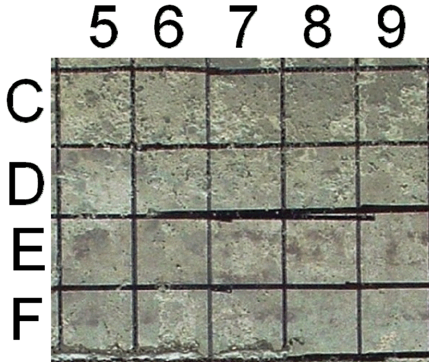
Figure 2-11. Photograph of Section One Grout Near the Base of Lift 3, Which Was Predicted by Ultrasonics To Be Free From Air Gaps. Much of the Lift 3 Surface in the Lower Half of the Photo Is Smooth. Near the Top, There Is More Pitting. Evidence of Preexisting Grout Splatters From Prior Pours Is Observed.
