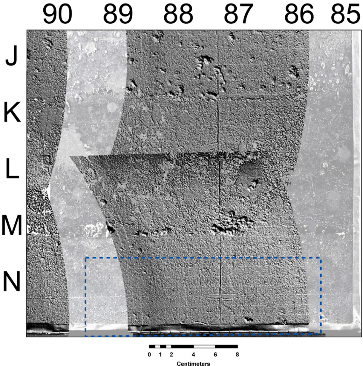
Figure 2-19(a). DSR Mosaic of a Portion of the Interior Surface of the Section Three Steel Tank Wall, Including Portions of the Area Shown In Figure 2-16. Areas of no Data Show a Semi-Transparent Version of the Photomosaic Shown in Figure 2-19(b). The Area Within the Dashed Blue Line Is Predicted by Ultrasonic Testing To Have an Air Gap; the Remaining Area Was Predicted To Be Free From Air Gaps. The Area Is Commonly Smooth, With Rough Areas in Rows J And M. The DSR Shows the Area Predicted To Be Not Bonded (Dashed Blue Rectangle) Is Relatively Smooth, With Very Small Topographic Relief. Soapstone-Inscribed Guidelines, As Described in Figure 2-17 Are Clearly Visible.
