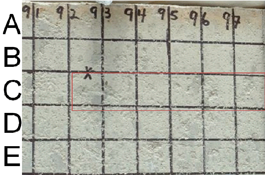
Figure 2-15. Photograph of Section Three Grout, Which Was Predicted by Ultrasonics To Have Air-Gaps. Much of the Lift 3 Area Is Rough. However, Ultrasonics Indicated That the Outlined Area Was Free From Air Gaps, Even Though it too Is Rough. Evidence of Preexisting Grout Spatters From Prior Pours Is Observed.
