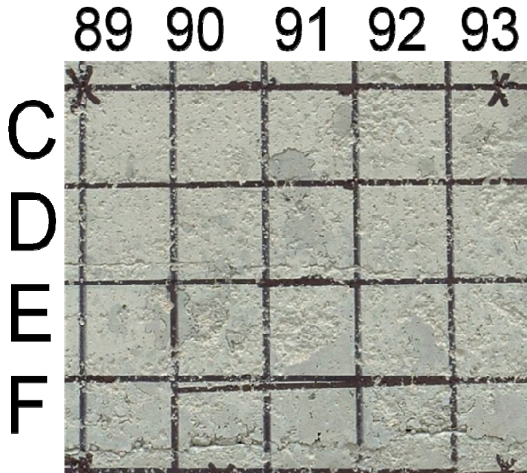
Figure 2-13. Photograph of Section Three Grout, Which Was Predicted by Ultrasonics To Have Air Gaps. Much of the Surface Is Pitted and Rough. Evidence of Preexisting Grout Spatters From Prior Pours Is Observed.
