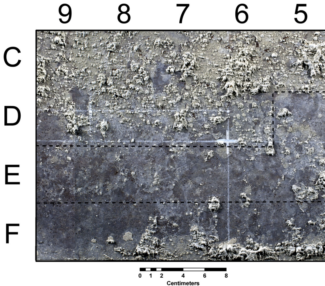
Figure 2-17(b). Digital Photograph of the Mirror Image Area Shown in Figure 2-11 and the Area Shown in Figure 2-17(a). Area Bounded by Dashed Lines Is as In Figure 2-17a. Surface Roughness Illustrated in Figure 2-17(a) Appears as Thin Coatings of Grout \sim \leq 2 mm [0.078 in] Thick That Remain Bonded to the Steel Tank Wall. Smooth Areas Appear as Grey Mottling With a Dark Red Undertone. The Grey Mottling Is Interpreted To Be a Thin Film of Grout Particles; the Dark Red Undertone Is Interpreted as the Original Antirust Red Coating of the Tank Wall and as Oxidation of the Tank Wall. Maximum Relief of the Mottled Areas Is Approximately 0.1 mm [0.039 in] Relative to the Surface of the Steel Plate.
