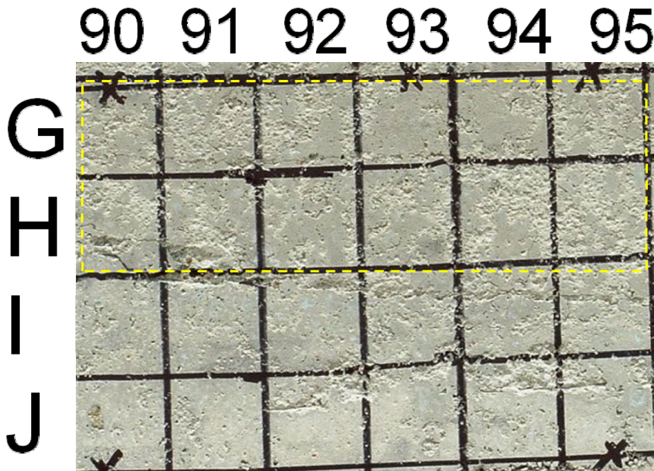
Figure 2-14. Photograph of Section Three Grout, Which Was Predicted by Ultrasonics To Have Air Gaps. Most of the Surface Is Pitted and Rough and Cracks Are Present. The Dashed Outline Encloses an Area Where the Coin-Tap Test Indicated Air Gaps Were Present.
