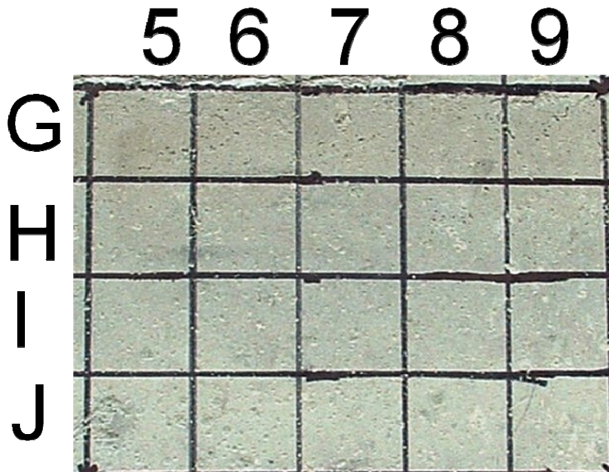
Figure 2-12. Photograph of Section One Grout at the Top of Lift 2, Which Was Predicted by Ultrasonics To Be Free From Air Gaps. Most of the Lift 2 Surface Is Smooth. Few Grout Splatters Are Observed.
