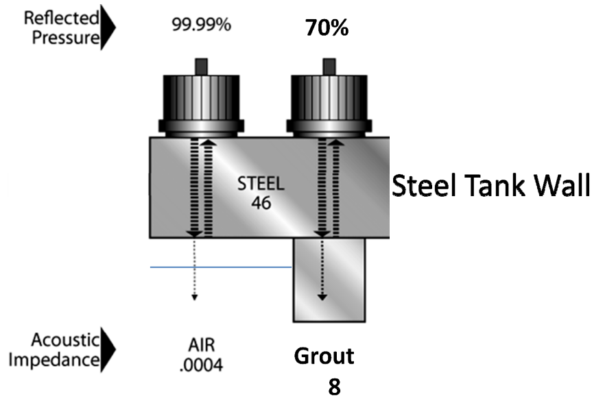
Figure 2-1. Illustration of the Reflection of Ultrasonic Waves From a Steel–Air Interface and a Steel–Grout Interface
