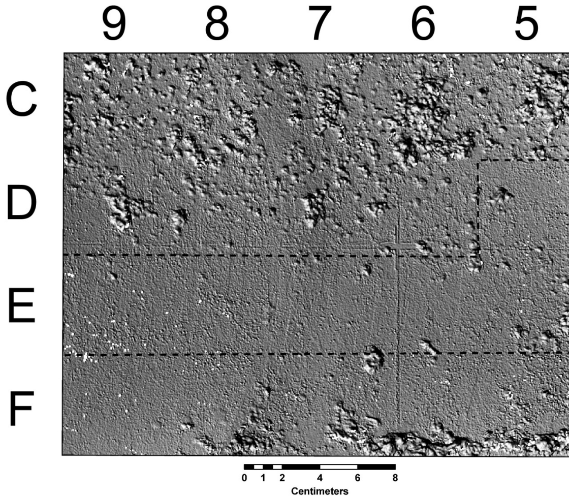
Figure 2-17(a). Dynamic Structured Light Data, Presented as DSR of a Portion of the Upper Lift (Lift 3) Exposed on the Interior Surface of the Section One Steel Tank Wall (See Figure 2-11). Ultrasonic Testing Predicted the Relatively Smooth Area Bounded by the Dashed Lines To Have Air Gaps; Relatively Rough Areas Above and Below Were Predicted To Be Free From Air Gaps. Rough Areas Correlate to the Pitting Described in Figure 2-11. Maximum Vertical Relief of Grout Remnants Is Approximately 2 mm [0.078 in] Relative to the Surface of the Steel Plate. Observe That Column Order Is Reversed Compared With Figure 2-11; the Inner Surface of the Tank Wall Presents a Mirror Image of the Exposed Grout Wall. The Faint Horizontal (Middle of Image) and Vertical (Center Right) Linear Features Were Guidelines Lightly Drawn on the Tank Wall With Soapstone; the Intersection Is Highlighted With a Paint Marker [See Figure 2-17(b)]. The Lines Do Not Correspond to Nondestructive Evaluation Sampling Grids. Drawn Prior to Collecting DSL Data, the Marks Visible in the DSR Attest to the Method's Sensitivity.
