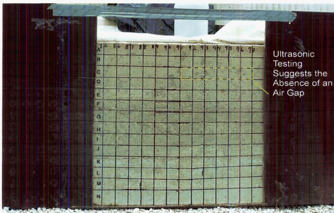
Figure 2-10. Photograph of the Grout Surface Adjacent to the Removed Tank Wall Within the Section Three Grid (cf. Figure 2-7)
