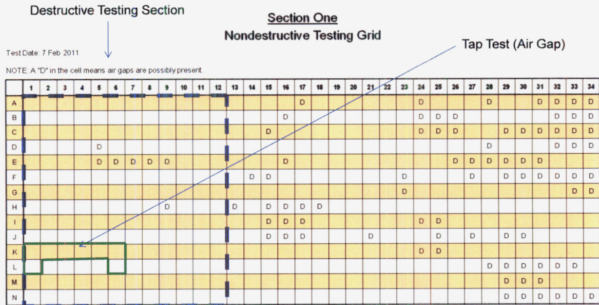
Figure 2-5. Illustration of the Section One Grid on the Tank Wall Shows Cells Where an Air Gap Was Detected (D) Between the Tank Wall and the Grout Using Ultrasound, Regions Where the Coin-Tap Test Indicated Possible Air Gaps, and a Representative Region Free From Air Gaps That Could Be Destructively Removed for Additional Analysis. Grid Cells Are 5 × 5 cm 2 [2 × 2 in 2 ].
