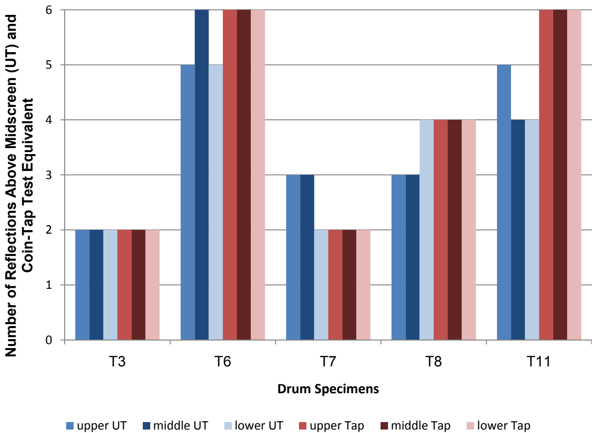
Figure 2-3. Ultrasonic and Coin-Tap Test Results for Each Lift Within Five Drum Grout Specimens. High Values Suggest Air Gaps and Low Values Suggest the Absence of Air Gaps.
