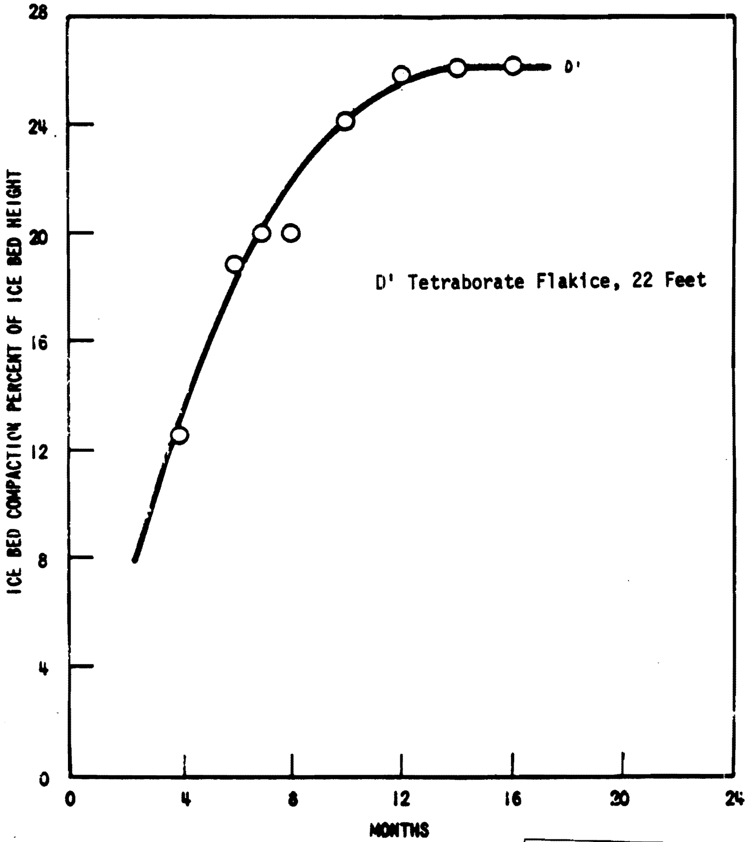
WATTS BAR NUCLEAR PLANT FINAL SAFETY ANALYSIS REPORT ICE BED COMPACTION VERSUS TIME Figure 6.7-35
