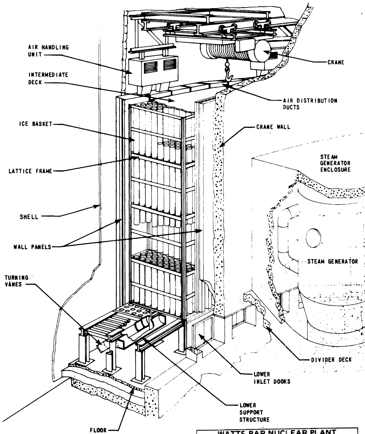
WATTS BAR NUCLEAR PLANT FINAL SAFETY ANALYSIS REPORT ISOMETRIC OF ICE CONDENSER Figure 6.7-1
