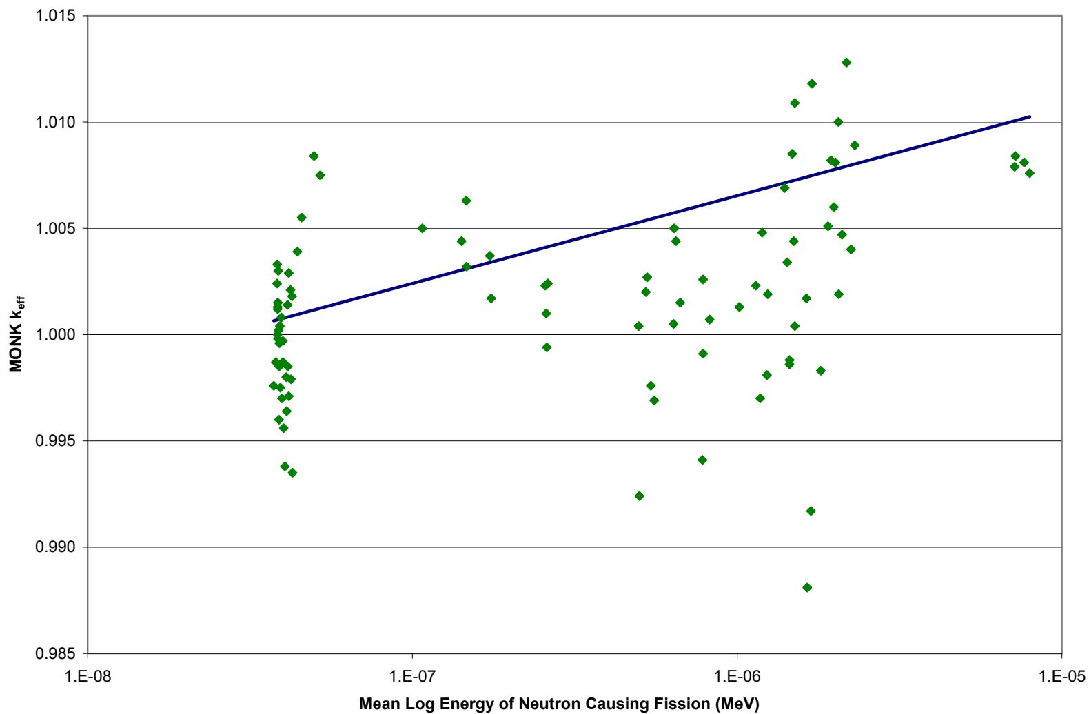
Figure 6-6: Plot of MONK8A k_{eff} vs. Mean Log Energy of Neutron Causing Fission (MLENCF)
