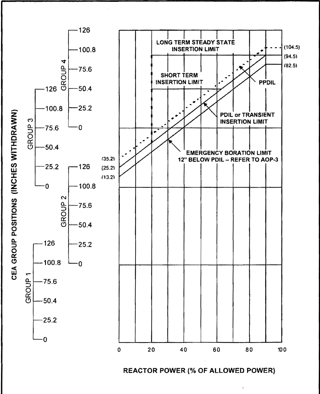
COLR POWER DEPENDENT INSERTION LIMIT FIGURE 2
