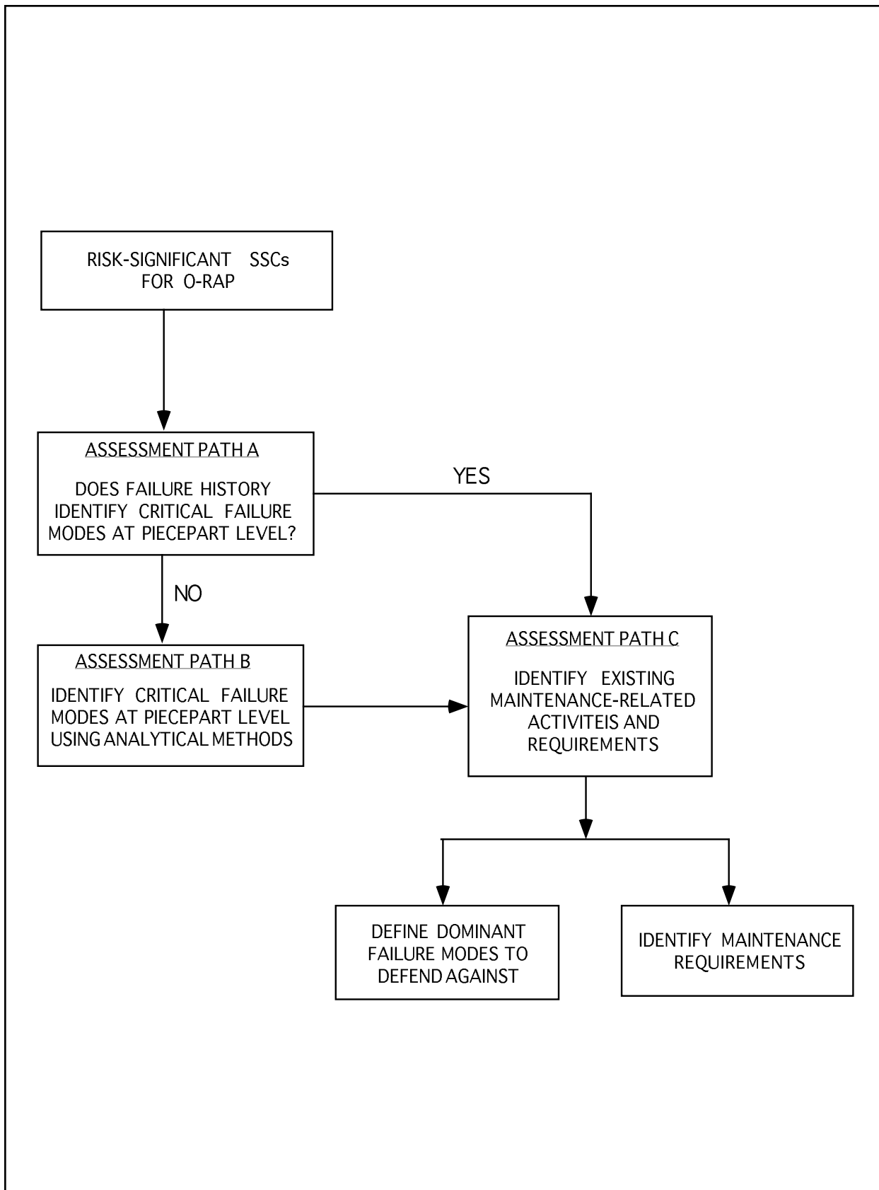
Figure 17.3-2 Process for Determining Dominant Failure Modes of Risk-Significant SSCs
