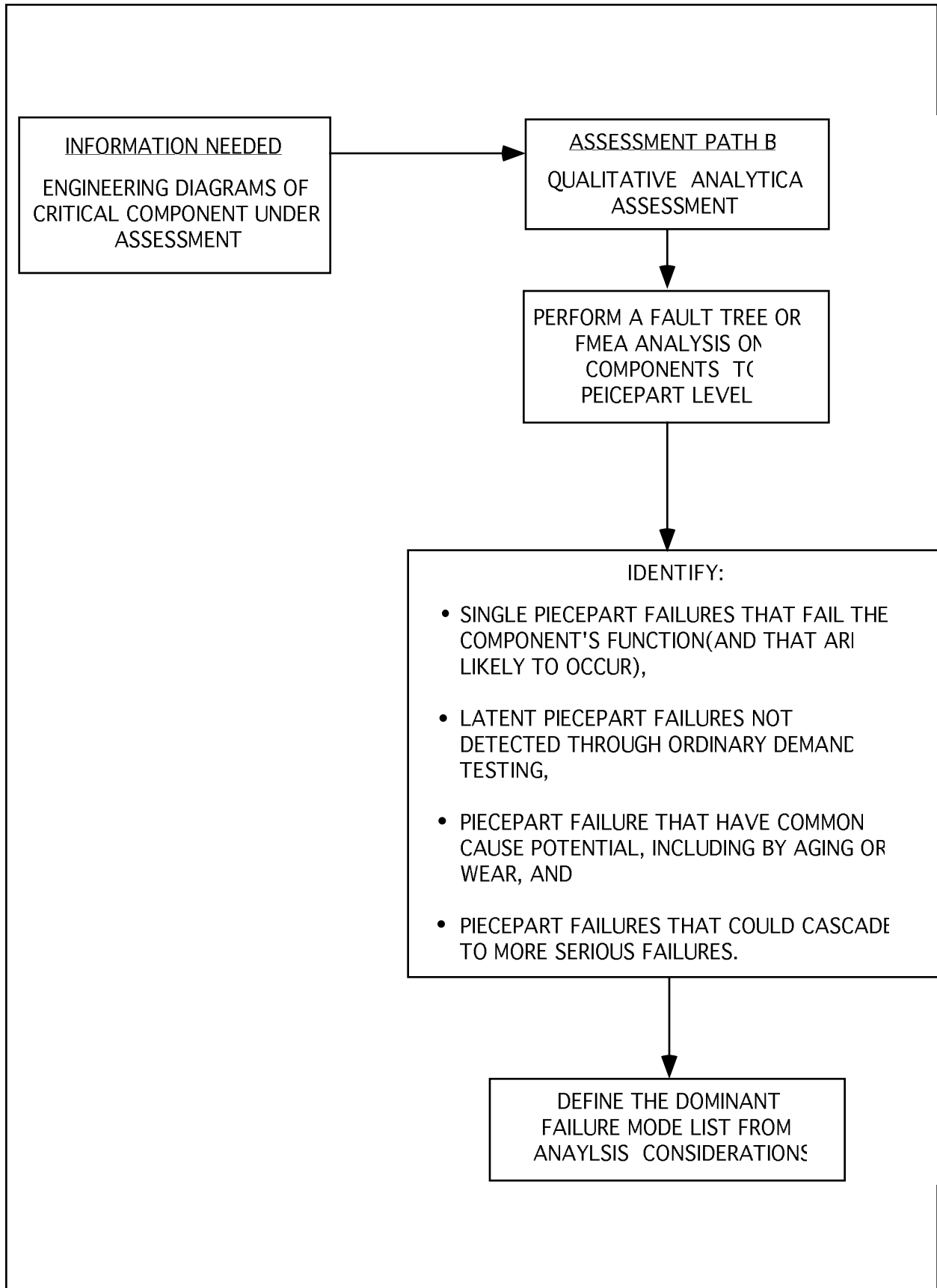
Figure 17.3-4 Analytical Assessment to Define Failure Modes
