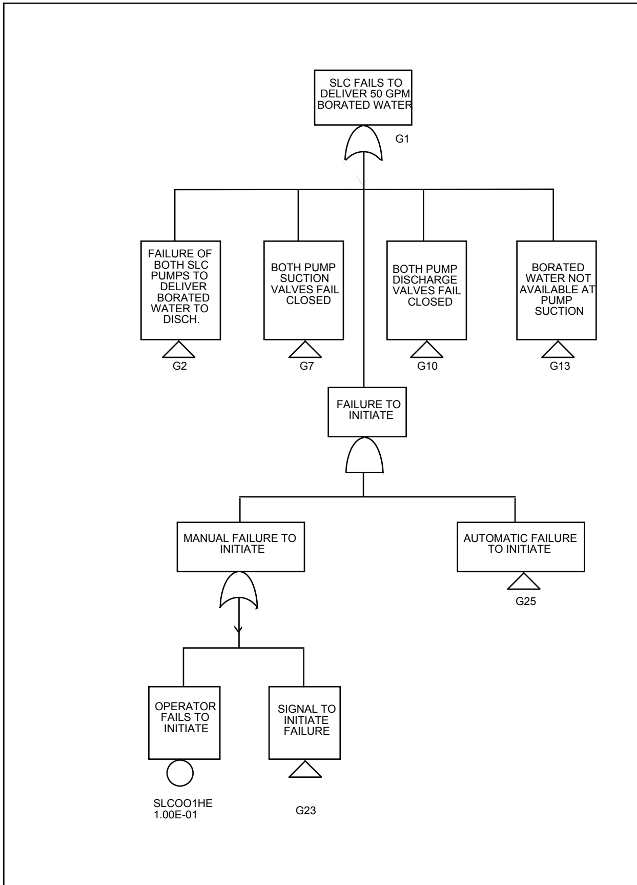
Figure 17.3-8 Standby Liquid Control System Top Level Fault Tree
