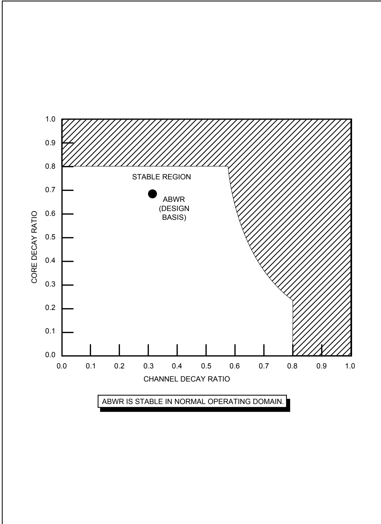
Figure 4.4-3 ABWR Stability
