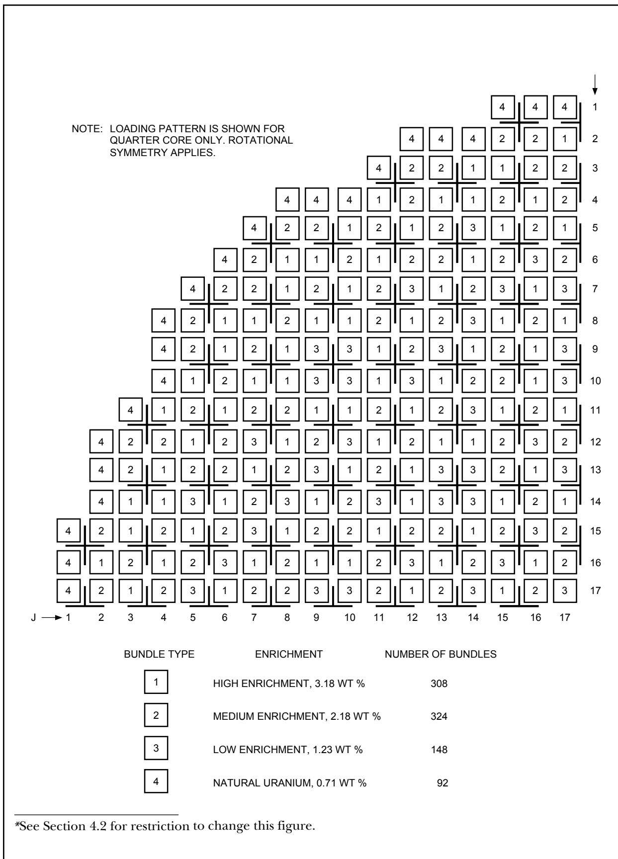
[Figure 4.3-1 Core Loading Map Used for Response Analyses]*
