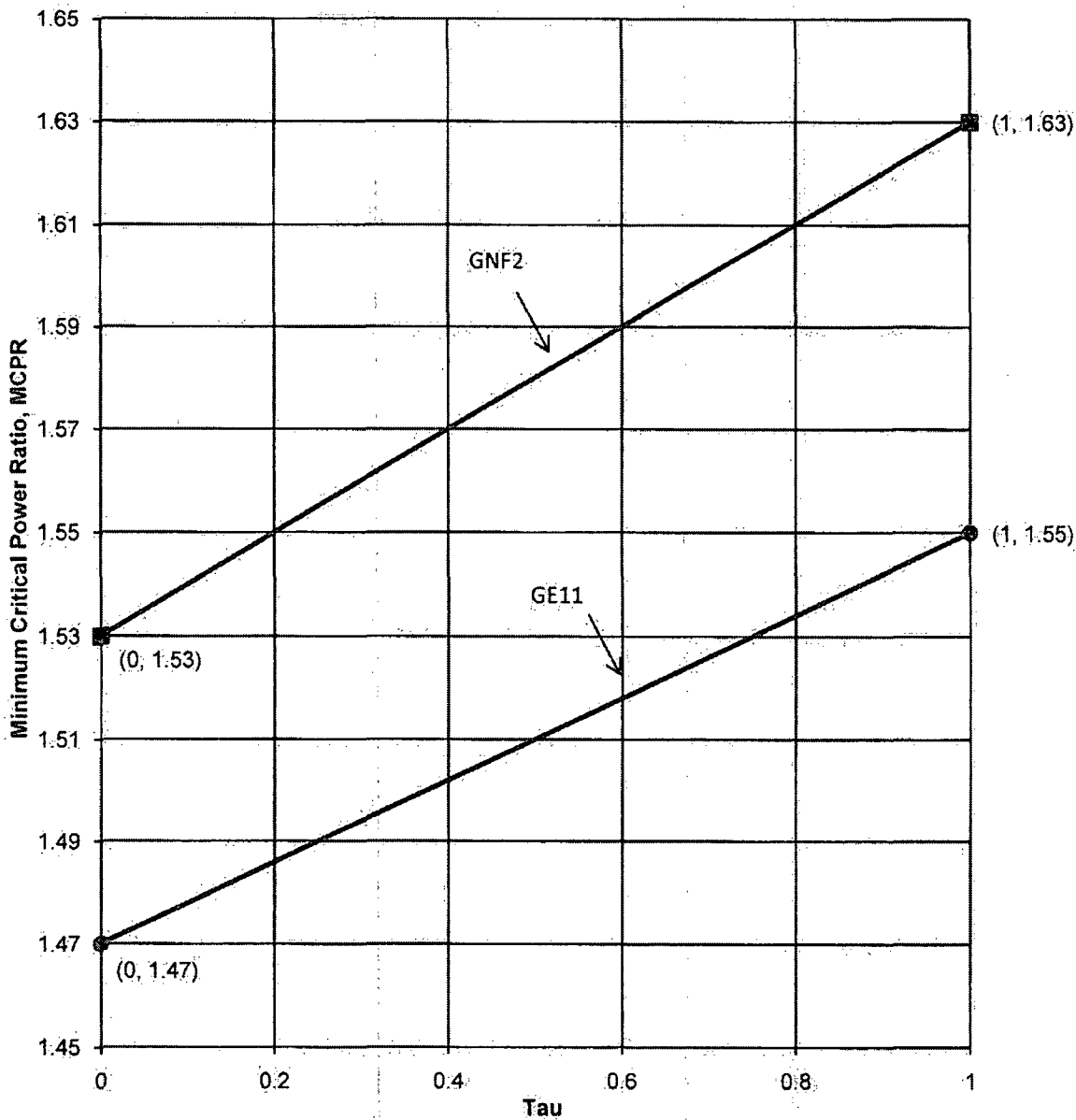
Figure 2c M CPR Operating Limits for Feedwater Pump Combination 2 maximum flows Beginning of Cycle to EOR*-1448 MWd/ST (Bounds TDFWP+ two MDFWPs)
