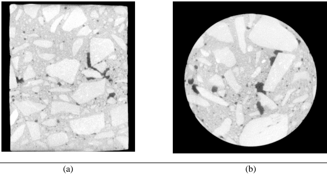
Figure 29. Longitudinal (a) and transverse (b) slice of three inch diameter base mat surrogate core sample TNK009B. Macro-porosity is represented by black features ( K_s = 1.6 \times 10^{-8} cm/sec).
