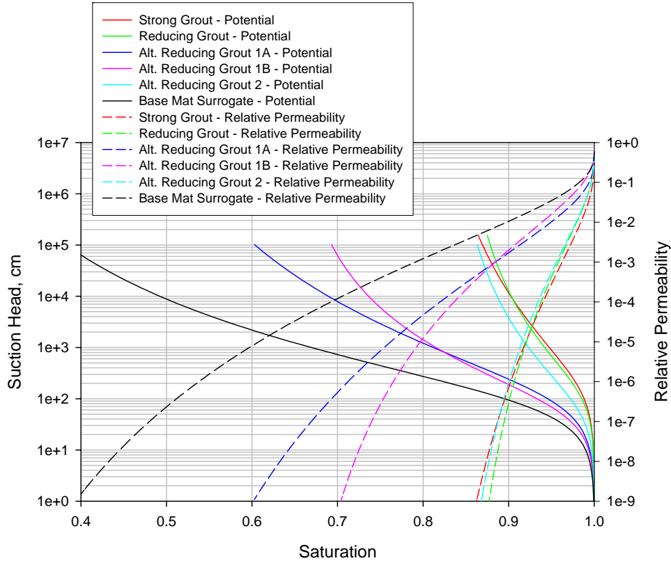
Figure 22. Recommended characteristic curves for FTF tank grouts and base mat surrogate.
