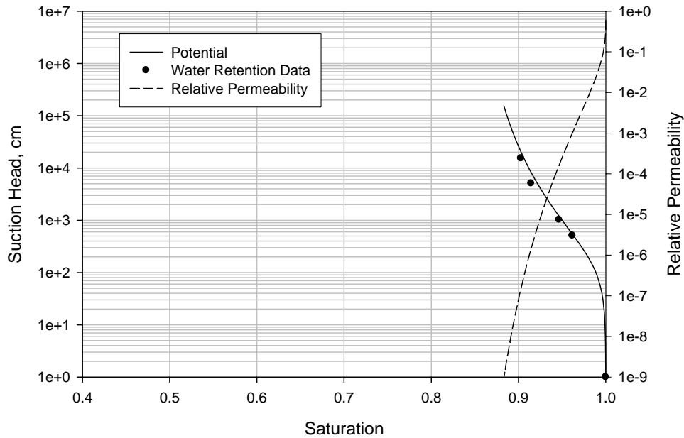
Figure 11. Characteristic curves for the reducing fill grout (OPDEXE-X-P-0-BS) as determined from MCT data.
