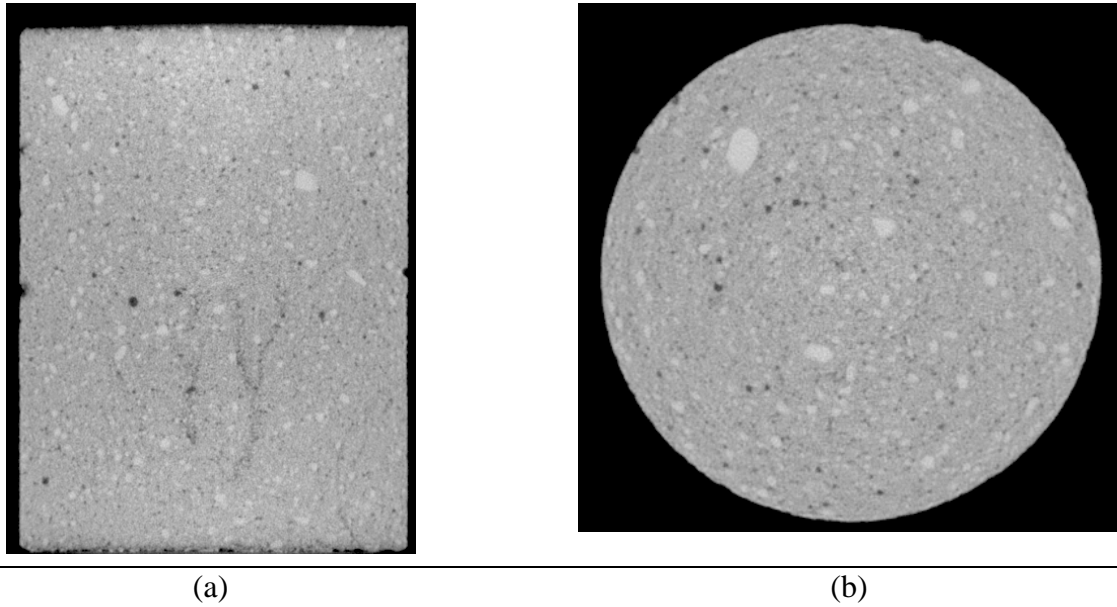
Figure 24. Longitudinal (a) and transverse (b) slice of three inch diameter strong grout mold sample TNK001S. Macro-porosity is represented by black features ( K_s = 2.8 \times 10^{-8} cm/sec).
