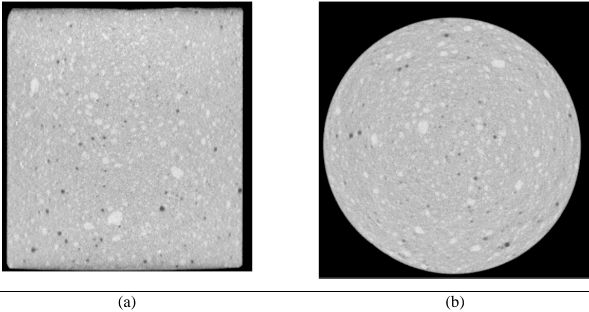
Figure 30. Longitudinal (a) and transverse (b) slice of three inch diameter alternative reducing fill grout 1A mold sample TNK027A1. Macro-porosity is represented by black features ( K_s = 8.2 \times 10^{-9} cm/sec).
