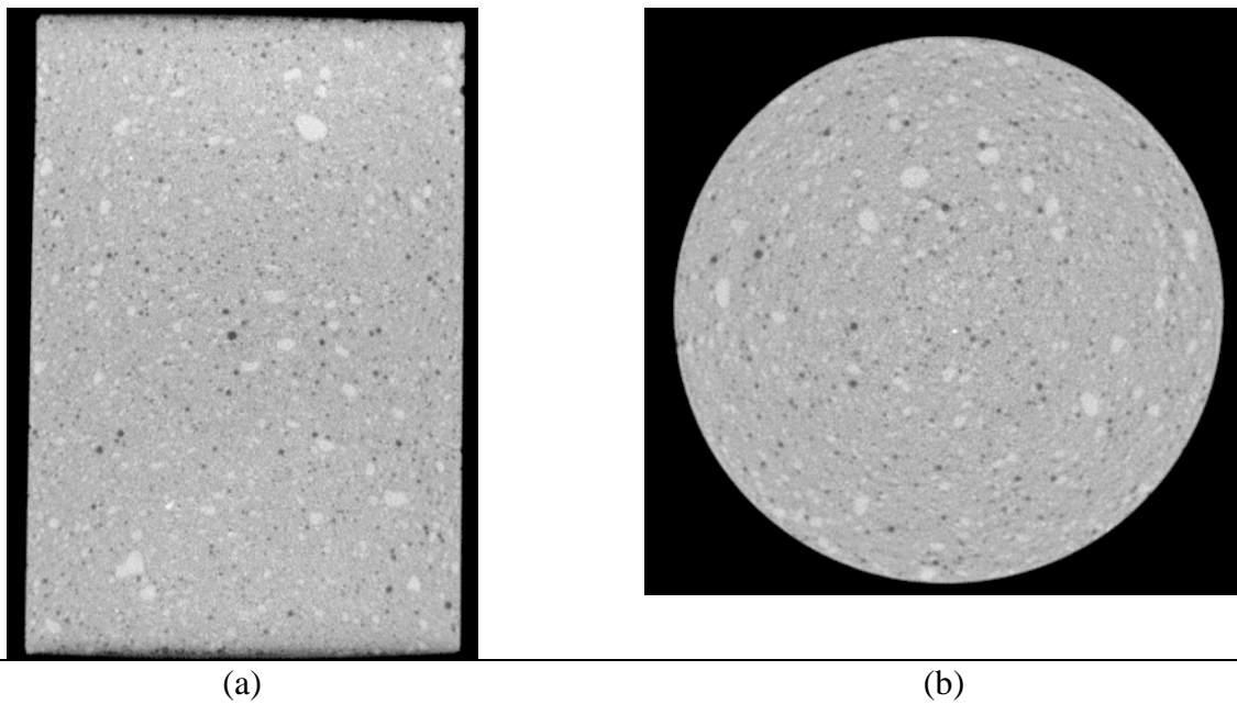
Figure 25. Longitudinal (a) and transverse (b) slice of three inch diameter strong grout mold sample TNK023S. Macro-porosity is represented by black features ( K_s = 6.8 \times 10^{-9} cm/sec).
