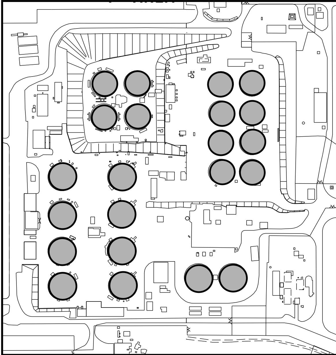
Figure 1. General Layout of the FTF.
