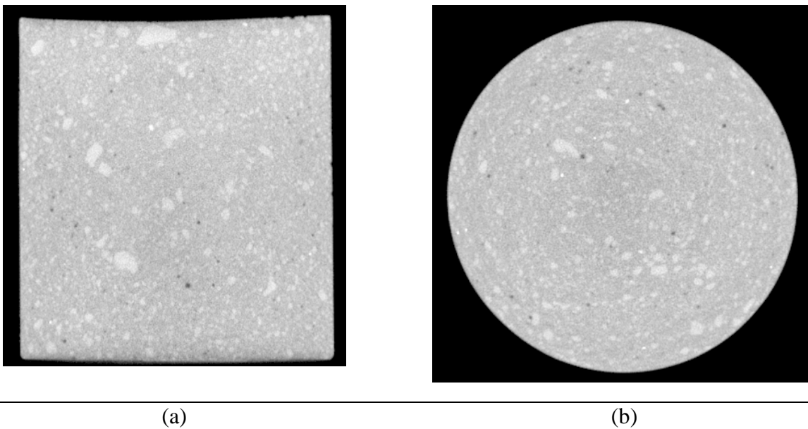
Figure 31. Longitudinal (a) and transverse (b) slice of three inch diameter alternative reducing fill grout 1B mold sample TNK029A2. Macro-porosity is represented by black features ( K_s = 1.0 \times 10^{-8} cm/sec).
