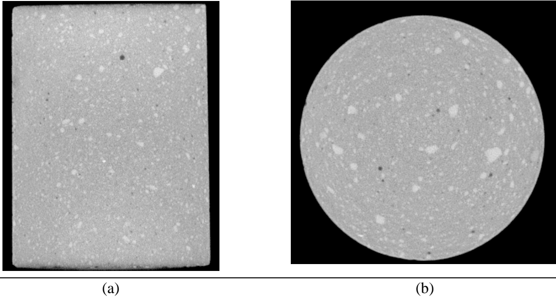
Figure 28. Longitudinal (a) and transverse (b) slice of three inch diameter reducing fill grout mold sample TNK025R. Macro-porosity is represented by black features ( K_s = 4.3 \times 10^{-8} cm/sec).
