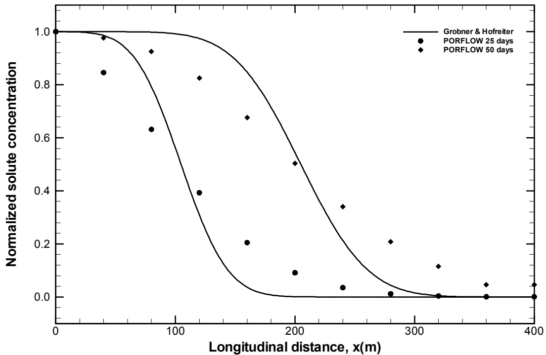
Figure 5.1.8 Concentration Profiles for the 1D Transport Showing Effect of Grid Size, \Delta x = 40 m (Case E).
