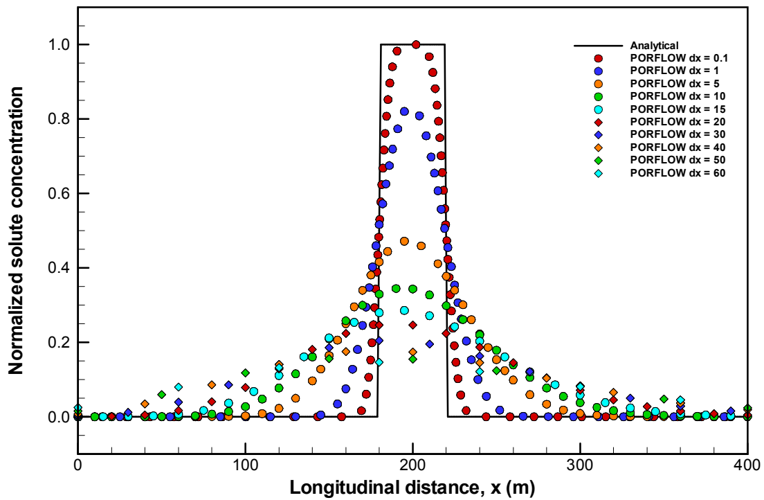
Figure 6.1.1. Normalized Solute Concentration Profiles at 5.5 Years for Variable Mesh Spacing in PORFLOW with Numerical Dispersion.
