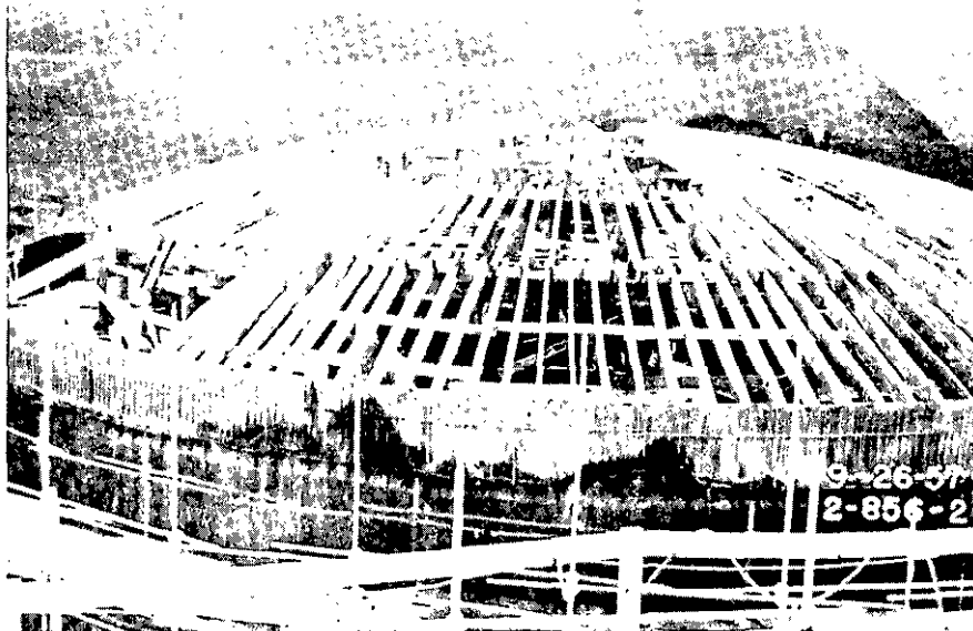
EXHIBIT VIII-B DOME FORMWORK
