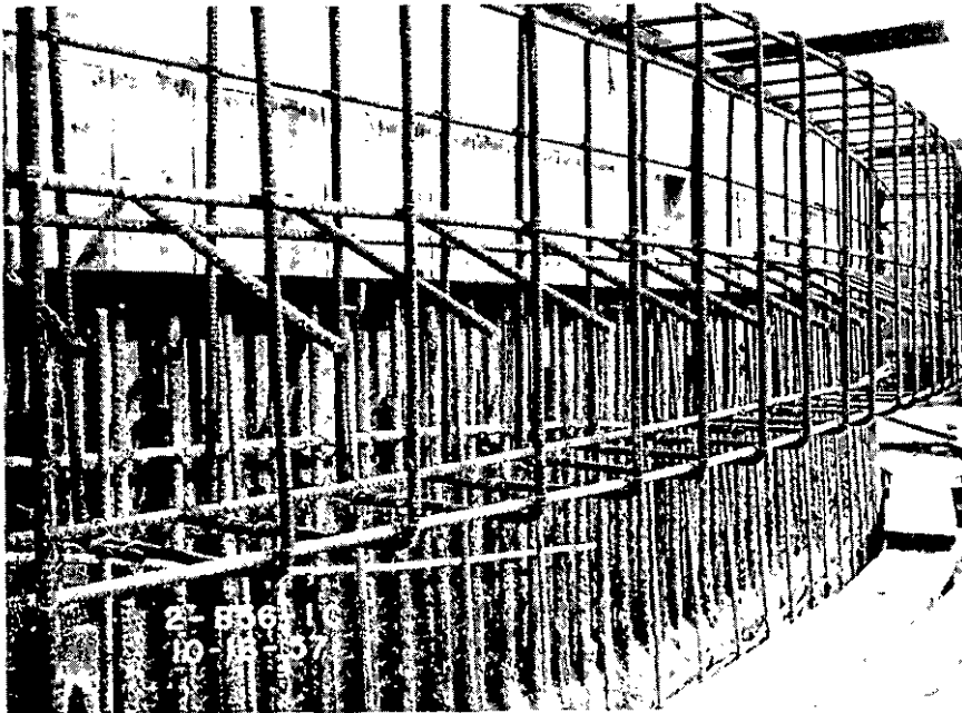
EXHIBIT IX-B DOME RING REINFORCING
