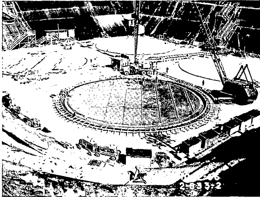
EXHIBIT VI-A FLOOR SLABS AND FOUNDATIONS SHOWING FORMWORK FOR DRAINAGE CHANNELS
