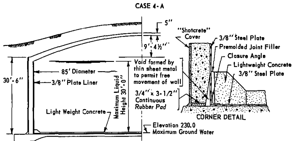
Prestressed 85-Ft-Diameter Poured Concrete Construction Modified Hanford Type
