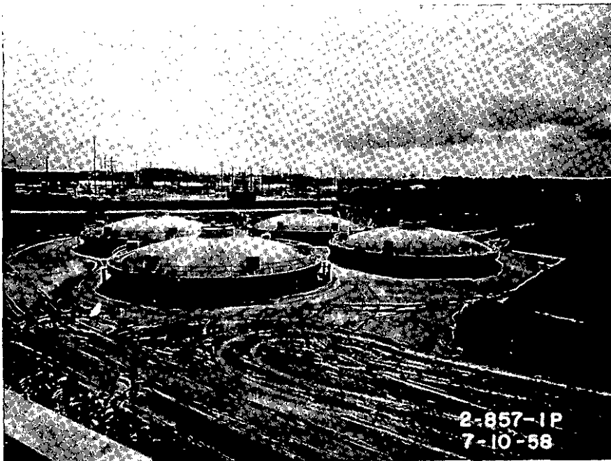
EXHIBIT XIII-B BACKFILL NEARING TOP OF WALL
