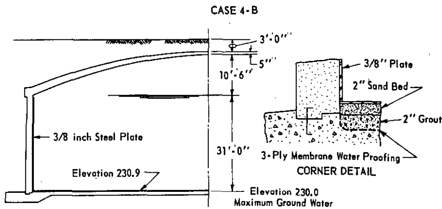
Prestressed 85-Foot-Diameter "Shotcrete" Construction
