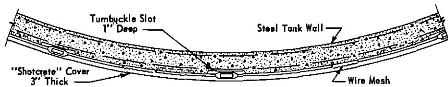
SECTIONAL PLAN
