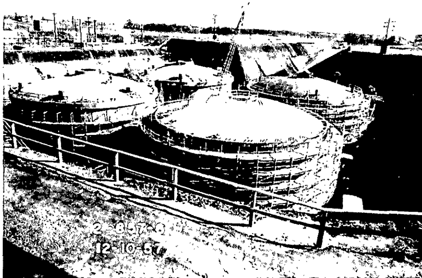
EXHIBIT XII-A COMPLETED DOME FORM DECK IN FOREGROUND
