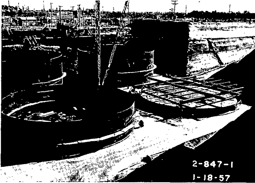
EXHIBIT VII-A ERECTION OF STEEL LINERS SHOWING ASSEMBLY OF WALL PLATES
