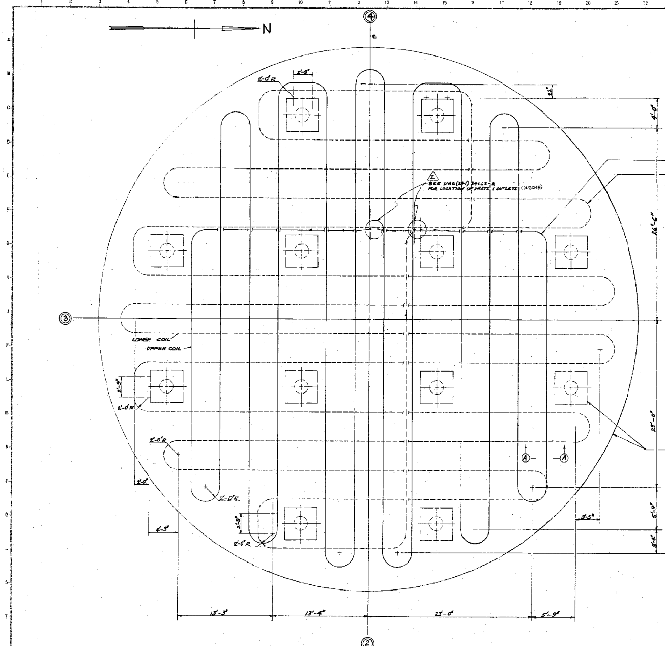
ALL PIPE SHOWN IN THIS PLAN TO BE SCH. 40. RANDOM LENGTHS PERMISSIBLE PLAN SCALE - 1/4" = 1'-0" BOTTOM COOLING COILS FOR WASTE STORAGE TANKS MATERIAL AS NOTED 116001 A & B AS SHOWN 116001 C & D OPPOSITE HAND ABOUT N-S
