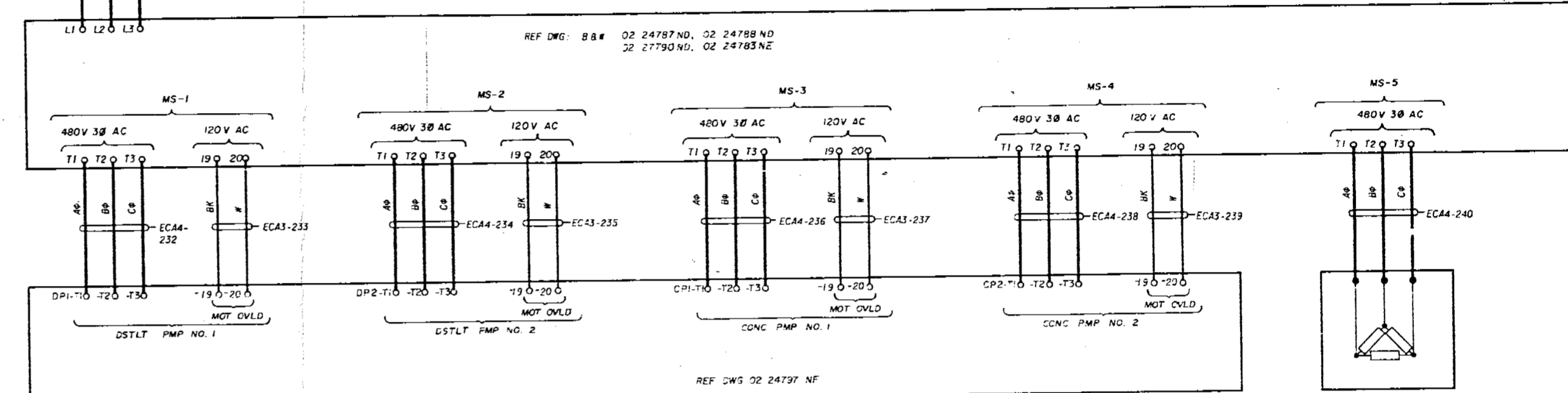
WASTE EVAP PACKAGE, MEVP-038 (FOR REST OF PACKAGE SEE BELOW AND SHEET 21)
