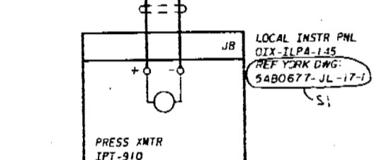
WASTE EVAP DSTLT TRANS PUMPS O18, O19 DISCH PRESS, IPT-910
