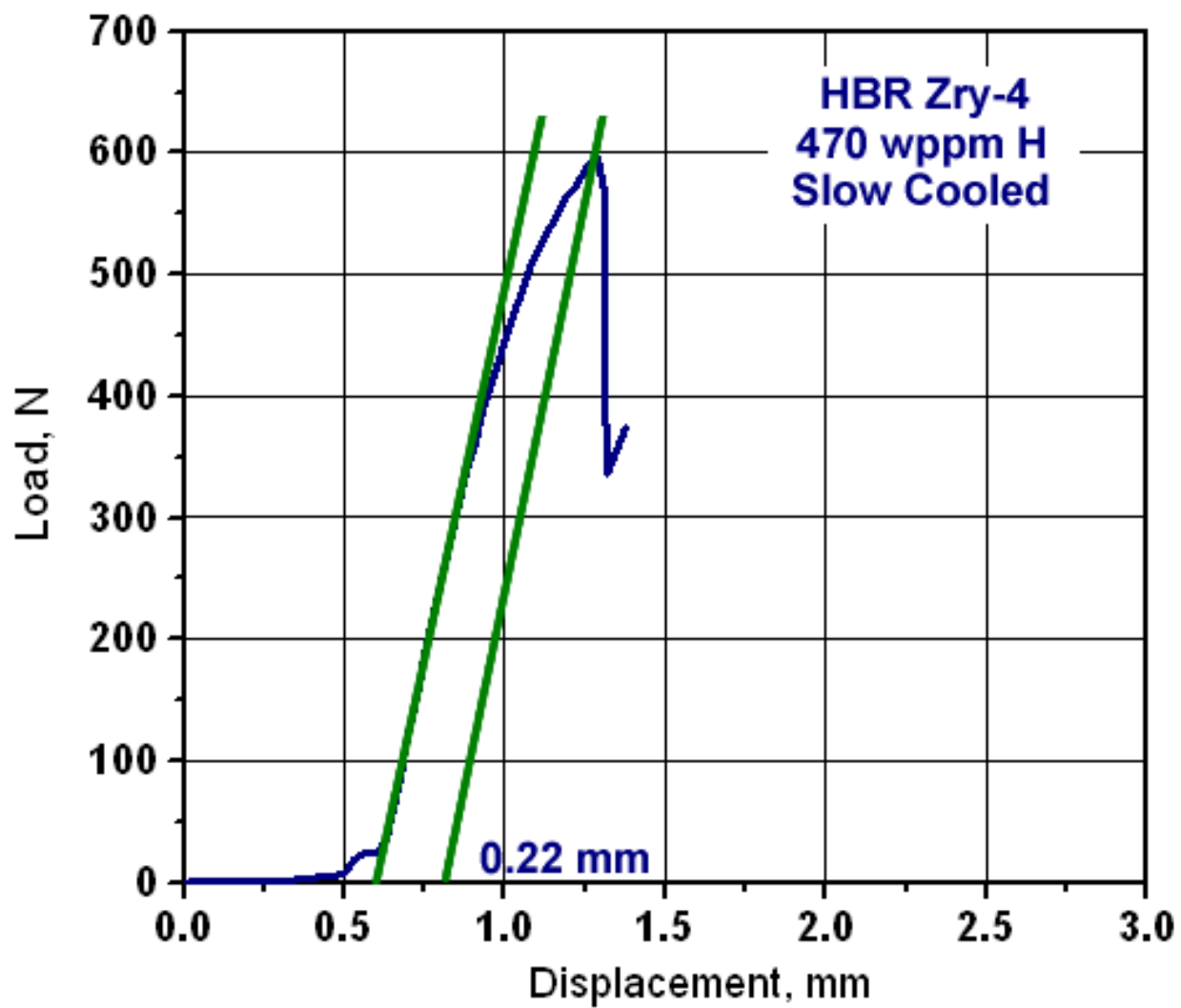
Figure B-7. Load-displacement results for ring #1 (8.04 mm long) of a prehydrided ( 470\pm 30 wppm) HBR 15×15 Zry-4 sample oxidized to 6% CP-ECR at a maximum oxidation temperature of 1,200 °C and cooled to room temperature without quench. The posttest sample had a tight through-wall crack at the support location. Offset and permanent displacements were 0.22 mm and 0.18 mm, respectively.
