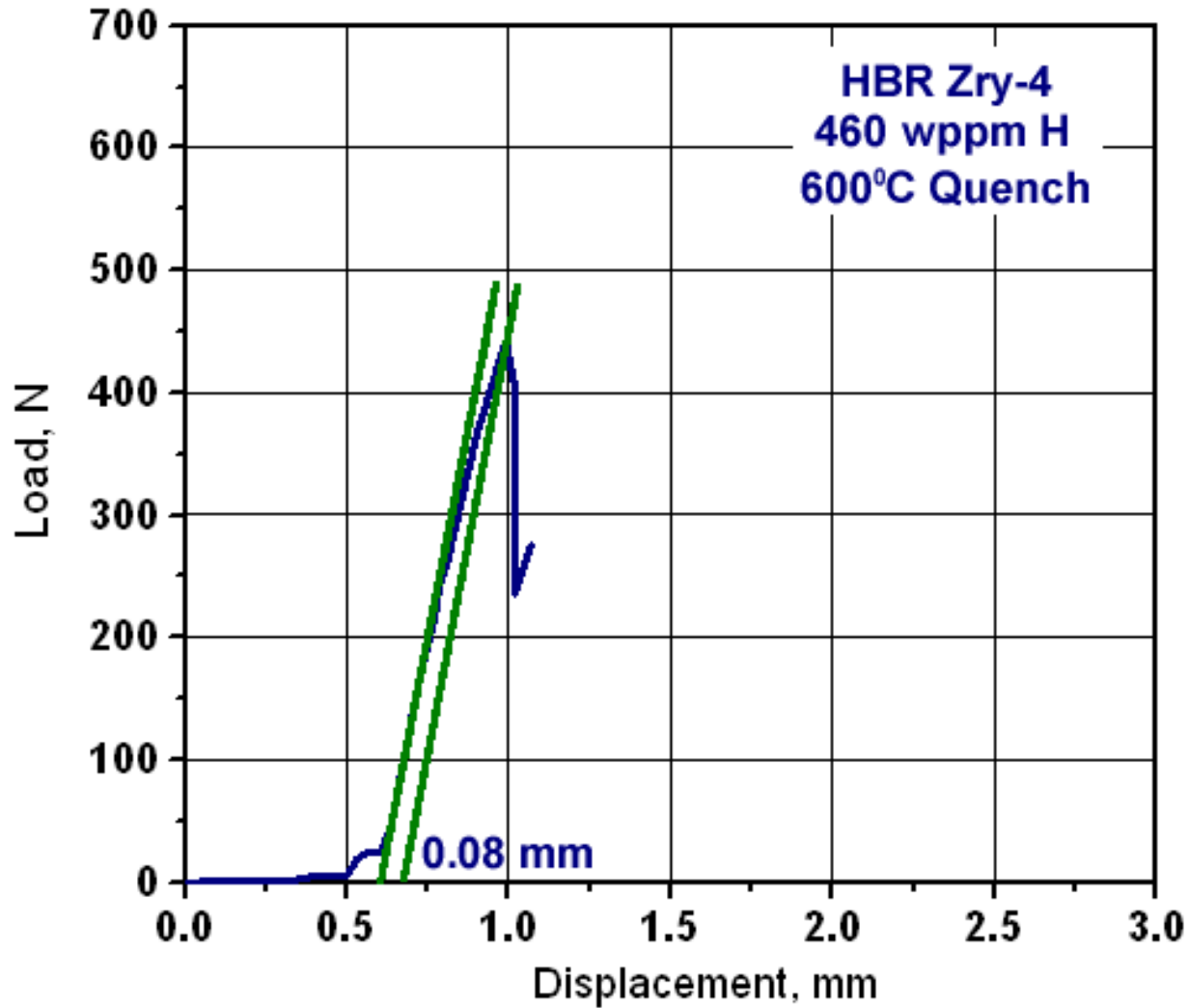
Figure B-5. Load-displacement results for ring #1 (7.93 mm long) of a prehydrided (460±30 wppm) HBR 15×15 Zry-4 sample oxidized to 6% CP-ECR at a maximum oxidation temperature of 1,200 °C and quenched at 600 °C. The posttest sample had a tight through-wall crack at the support location. Offset and permanent displacements were 0.08 mm and 0.05 mm, respectively.
