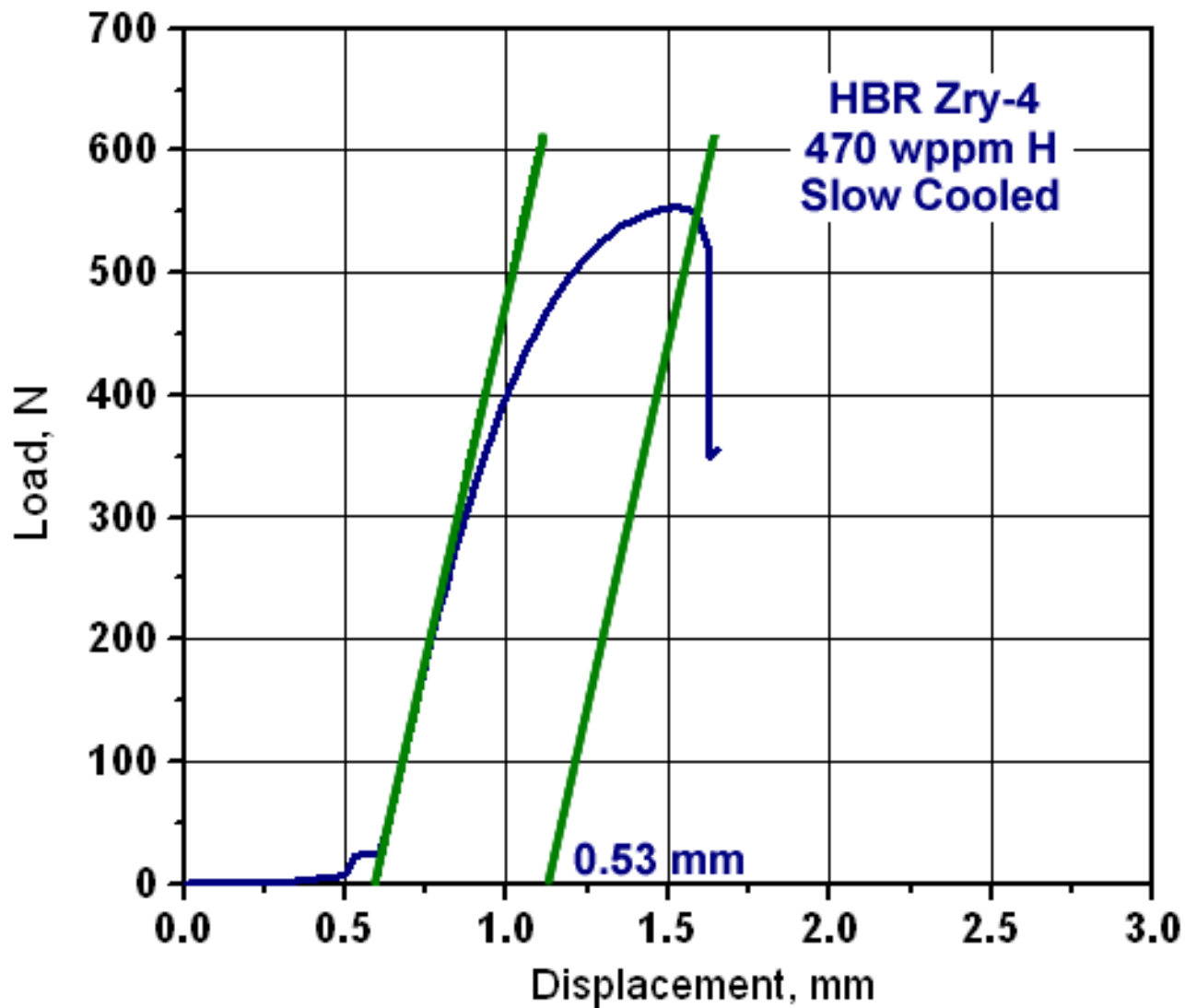
Figure B-8. Load-displacement results for ring #2 (7.05 mm long) of a prehydrided ( 470\pm 30 wppm) HBR 15×15 Zry-4 sample oxidized to 6% CP-ECR at a maximum oxidation temperature of 1,200 °C and cooled to room temperature without quench. The posttest sample had a tight through-wall crack at the loading location. Offset and permanent displacements were 0.53 mm and 0.39 mm, respectively.
