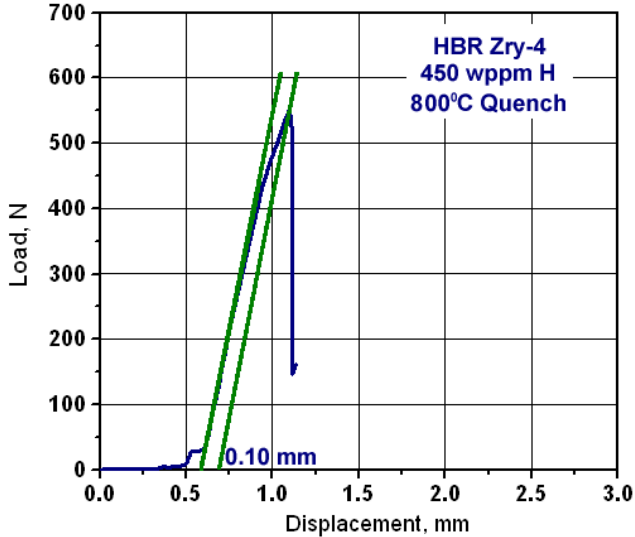
Figure B-1. Load-displacement results for ring #1 (8.12 mm long) of a prehydrided (450 wppm) HBR 15×15 Zry-4 sample oxidized to 6% CP-ECR at a maximum oxidation temperature of 1,200 °C and quenched at 800 °C. The posttest sample had tight through-wall cracks at load and support locations. Offset and permanent displacements were 0.10 mm and 0.08 mm, respectively.
