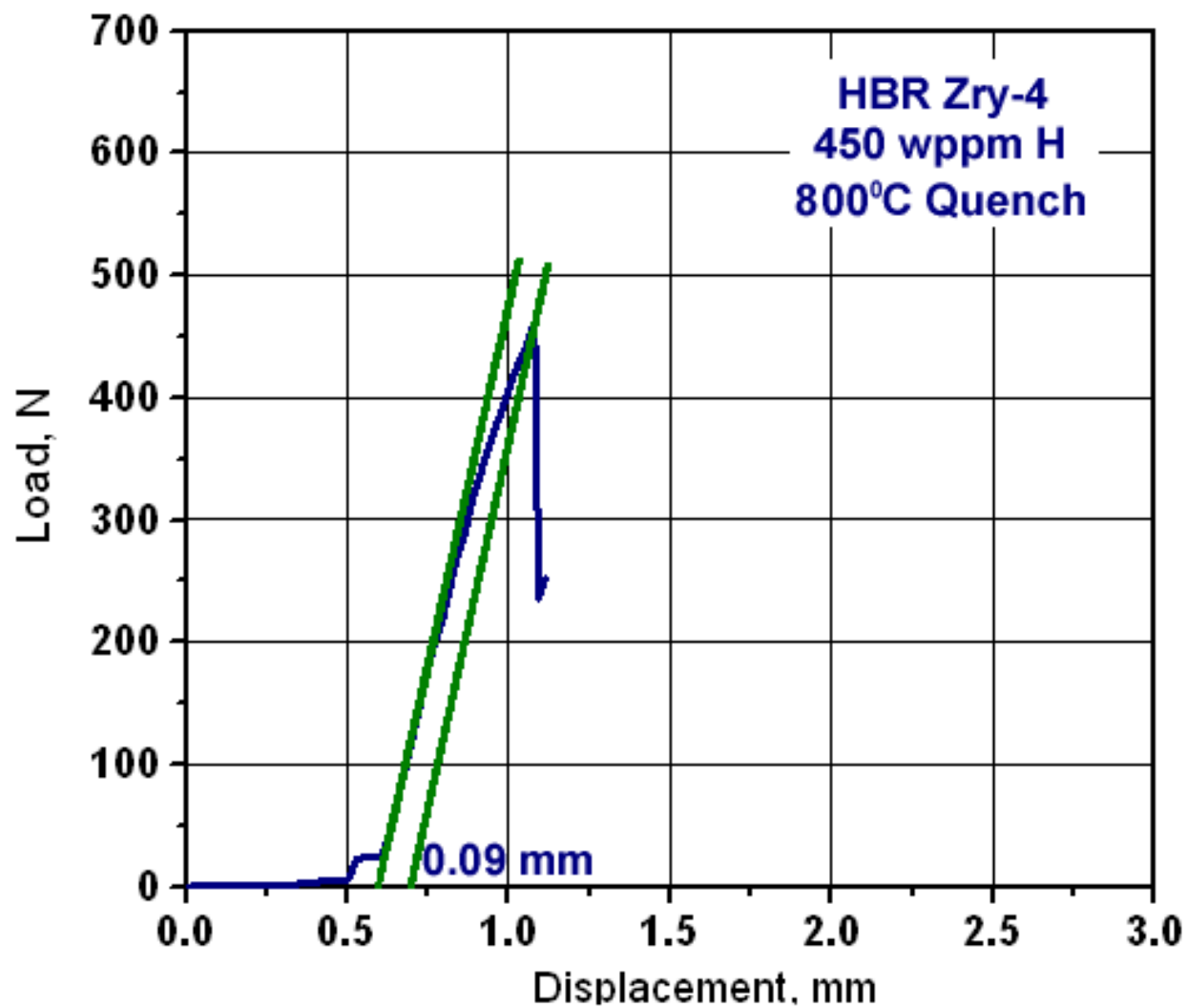
Figure B-2. Load-displacement results for ring #2 (6.84 mm long) of a prehydrided (450 wppm) HBR 15×15 Zry-4 sample oxidized to 6% CP-ECR at a maximum oxidation temperature of 1,200 °C and quenched at 800 °C. The posttest sample had a tight through-wall crack at the support locations. Offset and permanent displacements were 0.09 mm and 0.07 mm, respectively.
