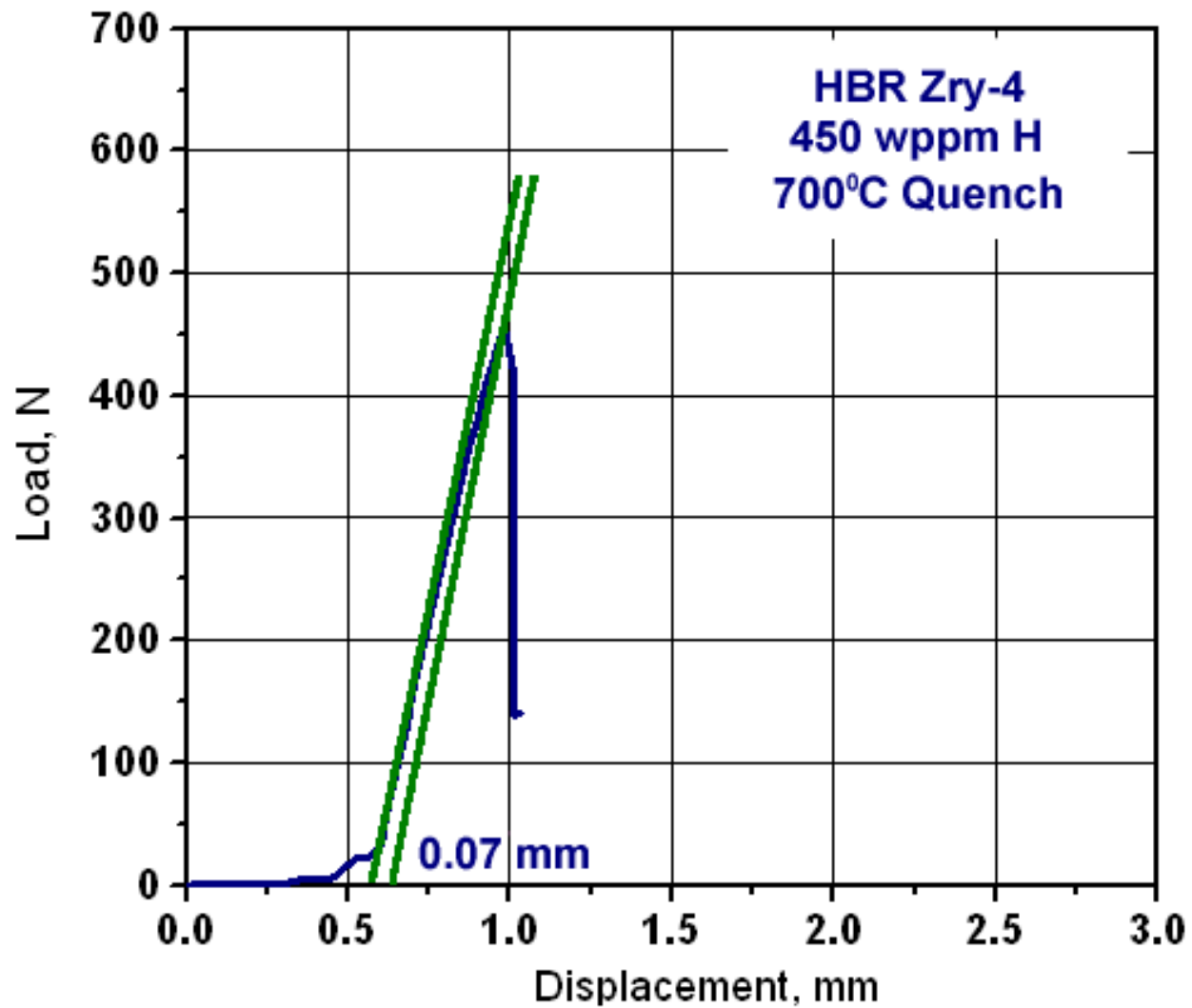
Figure B-3. Load-displacement results for ring #1 (8.08 mm long) of a prehydrided (450 wppm) HBR 15x15 Zry-4 sample oxidized to 6% CP-ECR at a maximum oxidation temperature of 1,200 °C and quenched at 700 °C. The posttest sample had through-wall cracks at load and support locations. Offset displacement was 0.07 mm.
