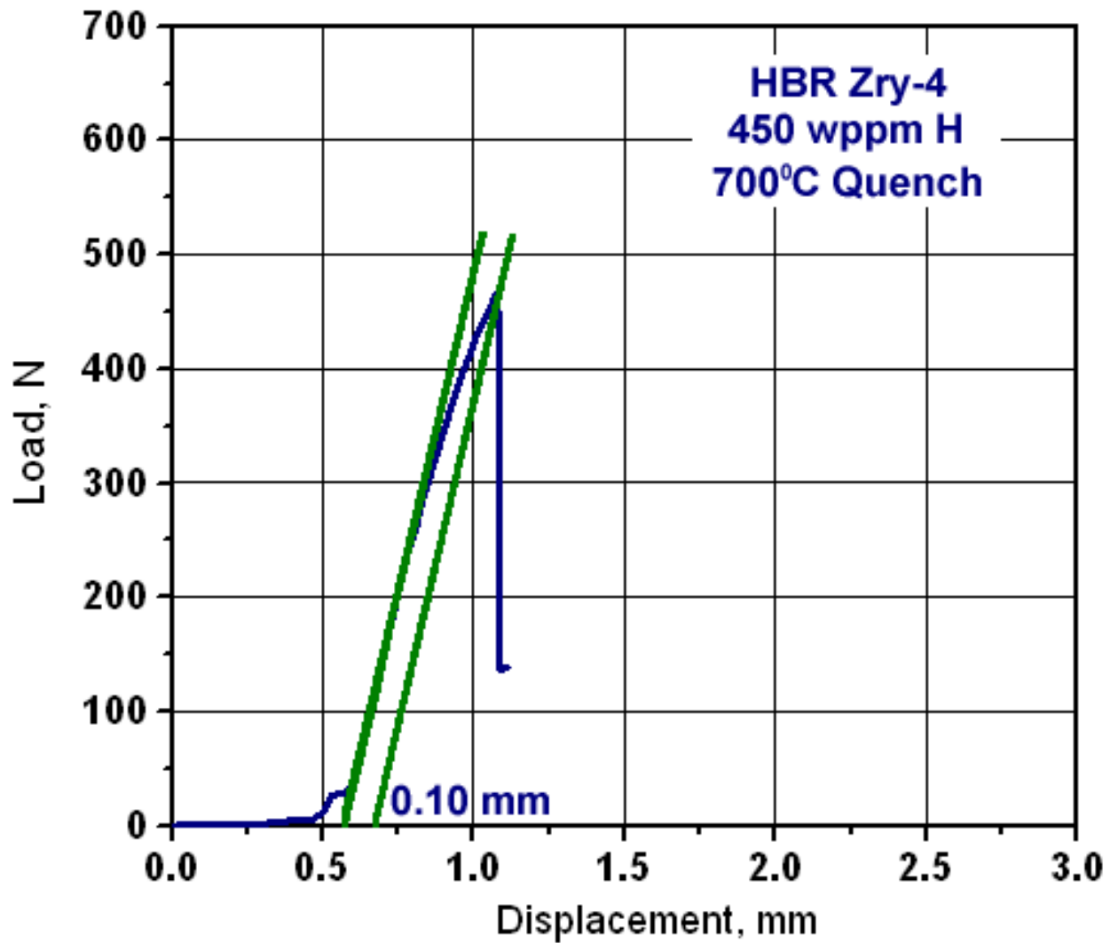
Figure B-4. Load-displacement results for ring #2 (7.30 mm long) of a prehydrided (450 wppm) HBR 15×15 Zry-4 sample oxidized to 6% CP-ECR at a maximum oxidation temperature of 1,200 °C and quenched at 700 °C. The posttest sample had tight through-wall cracks at load and support locations. Offset and permanent displacements were 0.10 mm and 0.05 mm, respectively.
