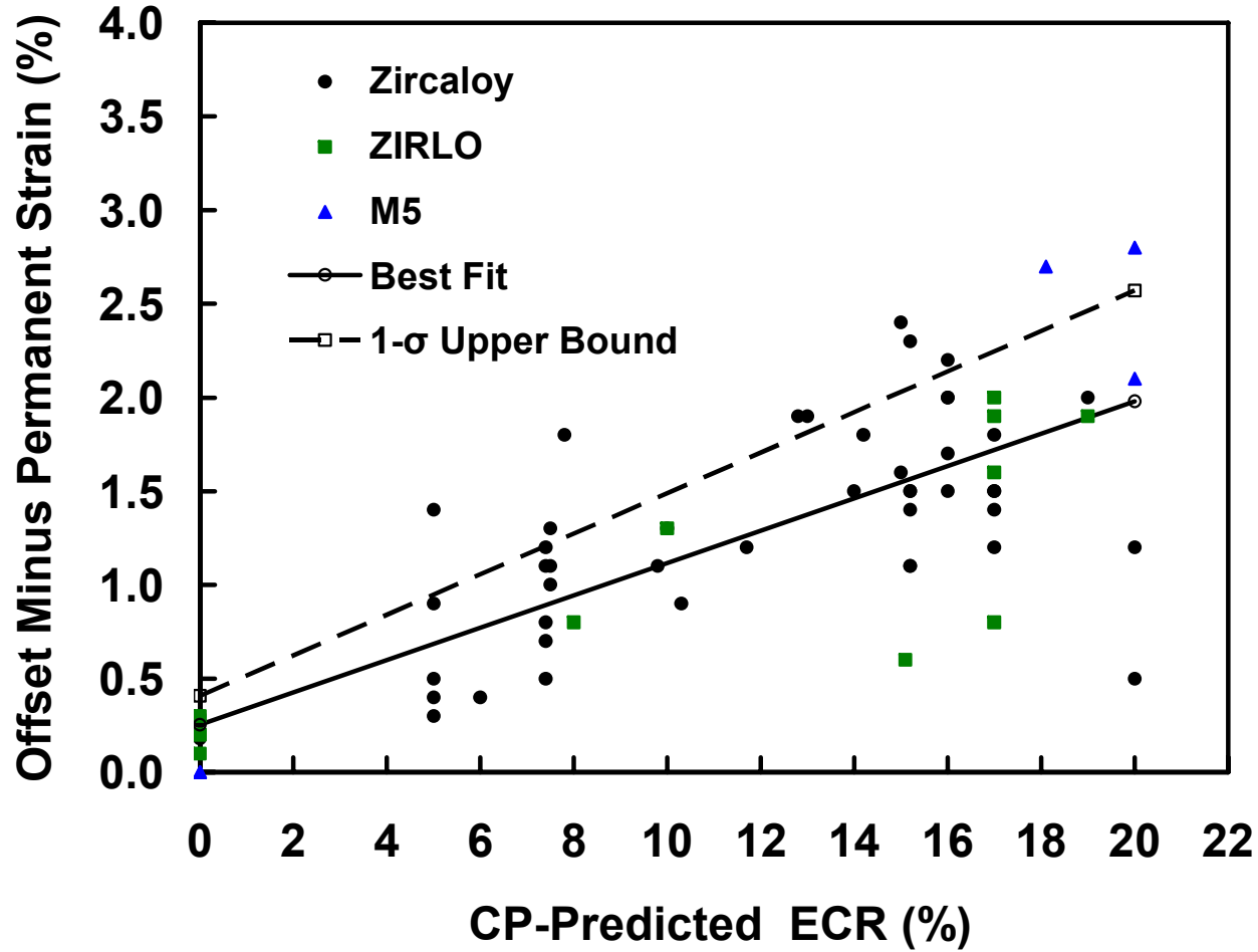
Figure C-1. Difference in offset strain and permanent strain as a function of calculated oxidation level (CP-ECR) for permanent strains near the embrittlement threshold (1.0 to 2.3%) for as-fabricated, prehydrided, and high-burnup cladding alloys oxidized at 1,200 °C and ring-compressed at room temperature and 135 °C and at 0.033 mm/s.
