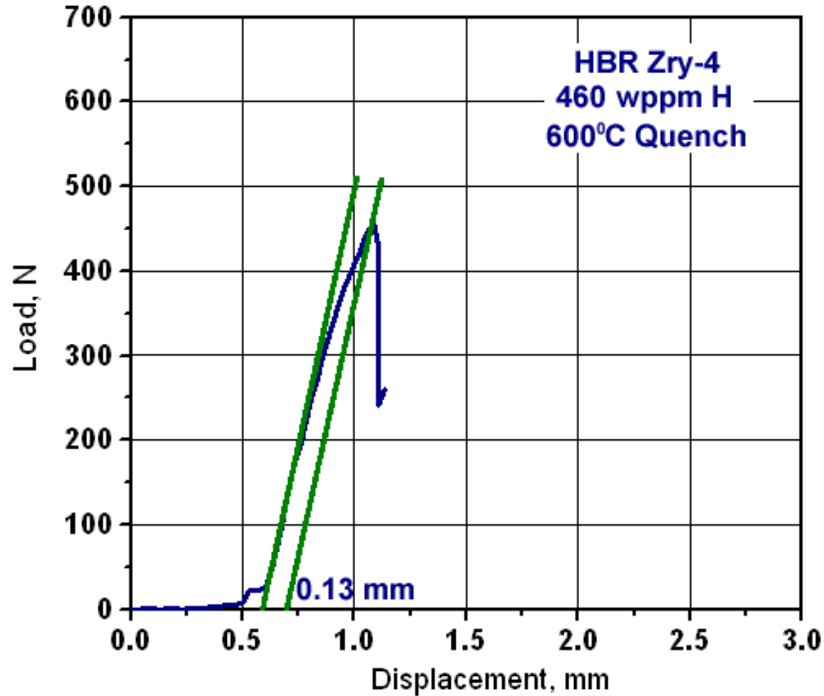
Figure B-6. Load-displacement results for ring #2 (7.05 mm long) of a prehydrided (460±30 wppm) HBR 15×15 Zry-4 sample oxidized to 6% CP-ECR at a maximum oxidation temperature of 1,200 °C and quenched at 600 °C. The posttest sample had a through-wall crack at the loading location. Offset and permanent displacements were 0.13 mm and 0.08 mm, respectively.
