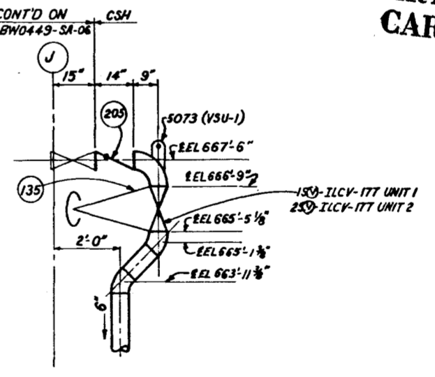
SECTION C9-C9 & D9-D9 UNITS 1 & 2, RESPECTIVELY SCALE: 1/2" = 1'-0" (SHEETS 05 & 06)
