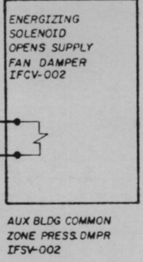
COMMON ZONE AREA SUPPLY FAN MFAN-002 SEE SIMPLIFIED CONTROL CIRCUIT DETAIL A
