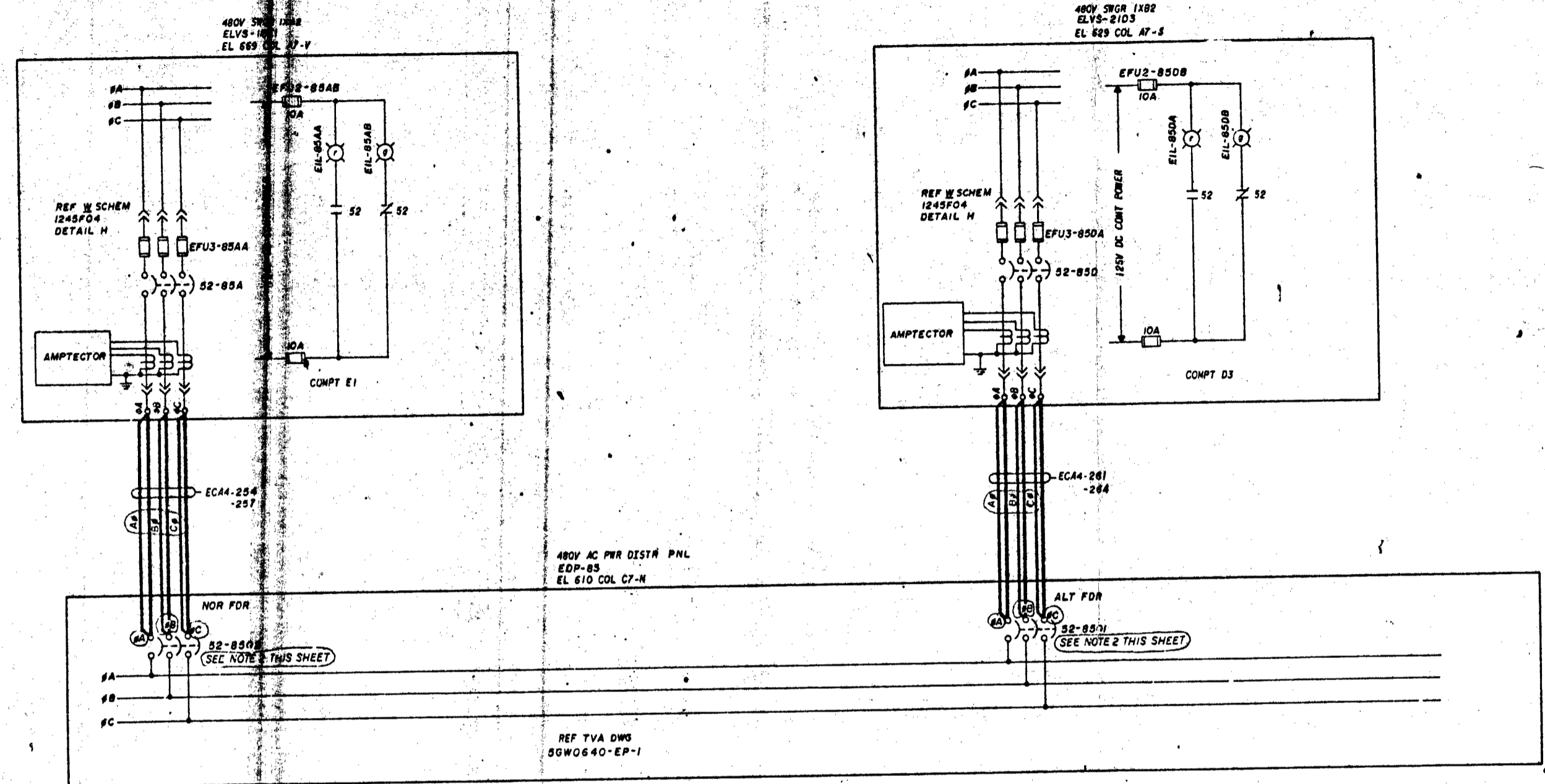
480V AC POWER DISTRIBUTION PANEL
