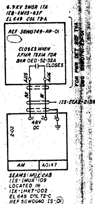
XFMR TSXIA FDR BKR SEAMS ALARM
