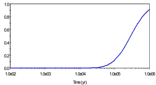
Fraction of waste packages failed by general corrosion
