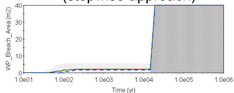
Waste package breached area (stepwise approach)
