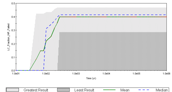
Fraction of waste packages failed by localized corrosion
