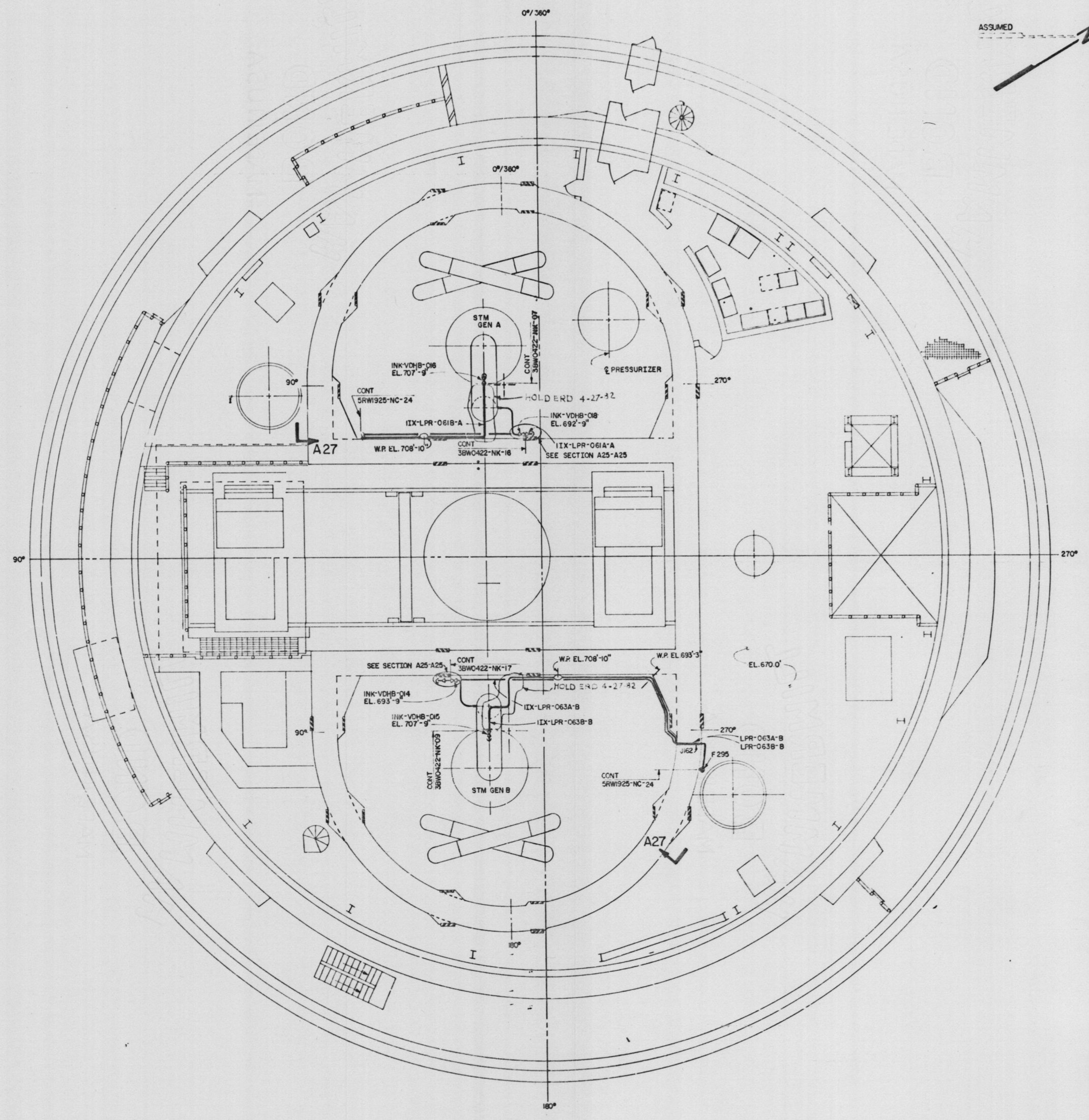
PLAN EL.670.0'
