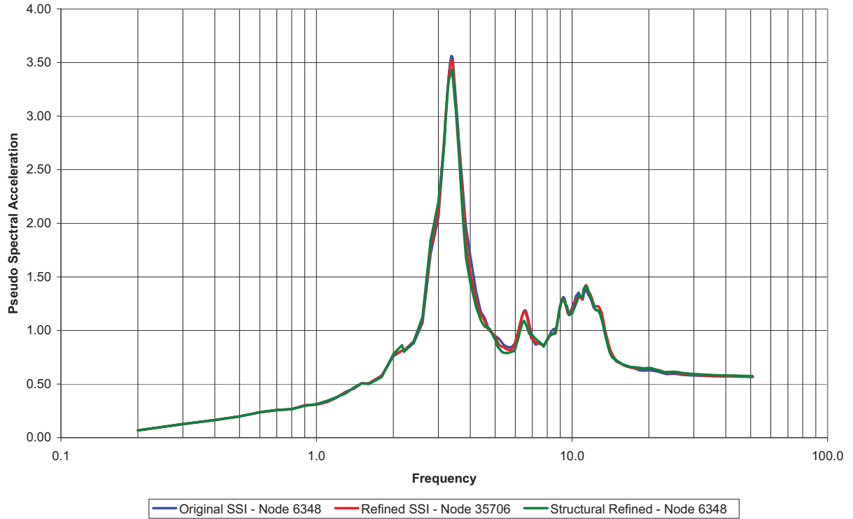
Figure 03.07.02-25.31: Bottom of Cooling Tower North Wall, Y-direction, 5% Damping
