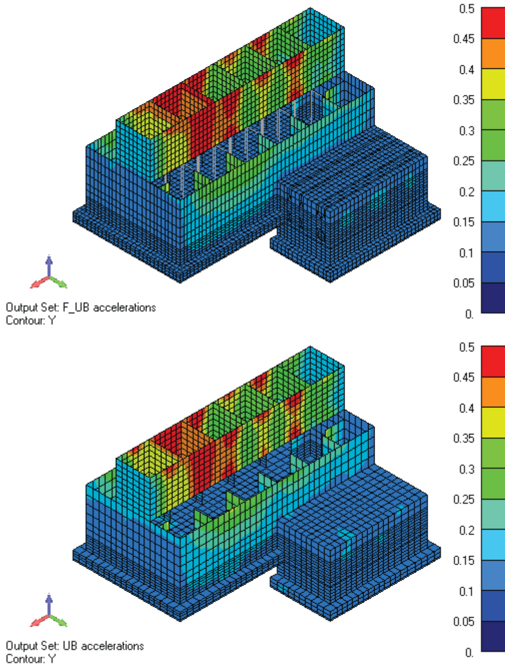
Figure 03.07.02-24.141: Acceleration contour plots of Refined Mesh Model (top) and Original Mesh Model (bottom) for Y-Direction accelerations from Full Basin Upper Bound Soil Case.
