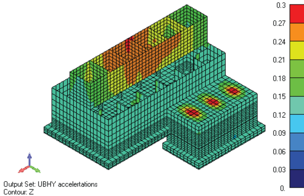
Figure 03.07.02-24.145: Acceleration contour plots of Refined Mesh Model (top) and Original Mesh Model (bottom) for Z-Direction accelerations from Empty Basin Upper Bound Soil Case.
