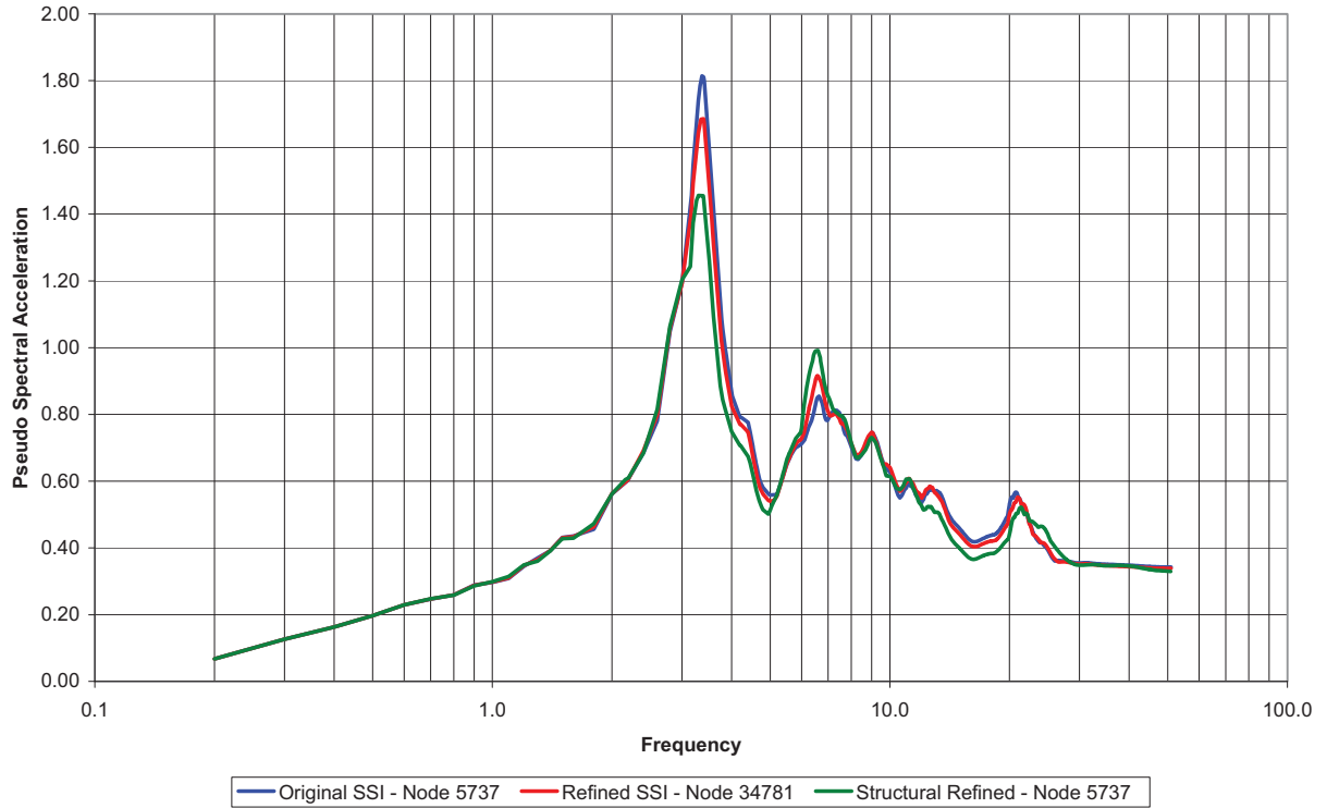
Figure 03.07.02-25.24: Basin South Wall, Y-direction, 5% Damping
