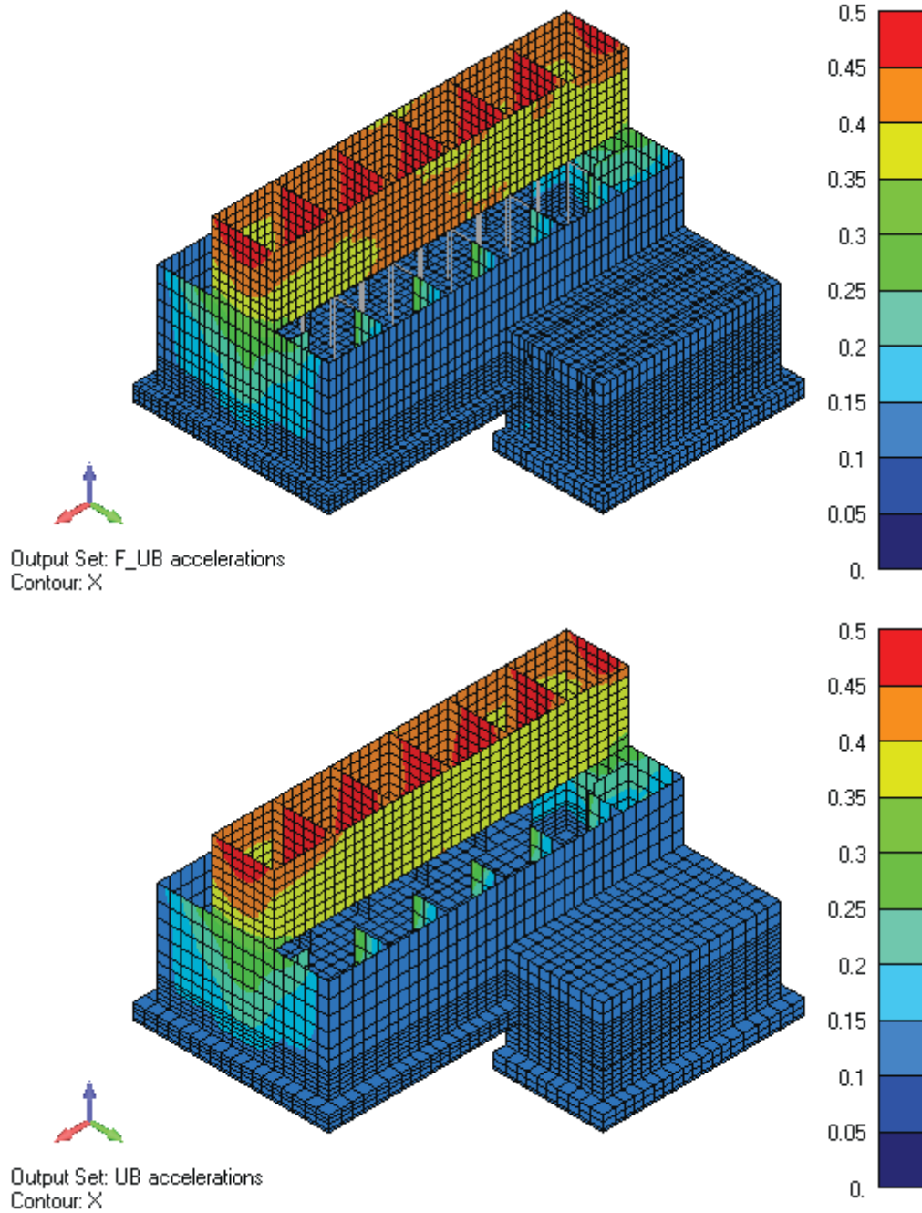
Figure 03.07.02-24.140: Acceleration contour plots of Refined Mesh Model (top) and Original Mesh Model (bottom) for X-Direction accelerations from Full Basin Upper Bound Soil Case.
