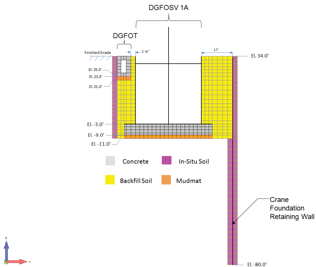
Figure 3H.6-225: 2D SSSI Model of DGFOT, DGFOV and Crane Foundation Retaining Wall
