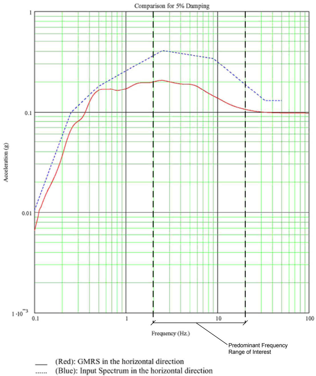
Comparison of GMRs with the Input Spectrum (Horizontal)
