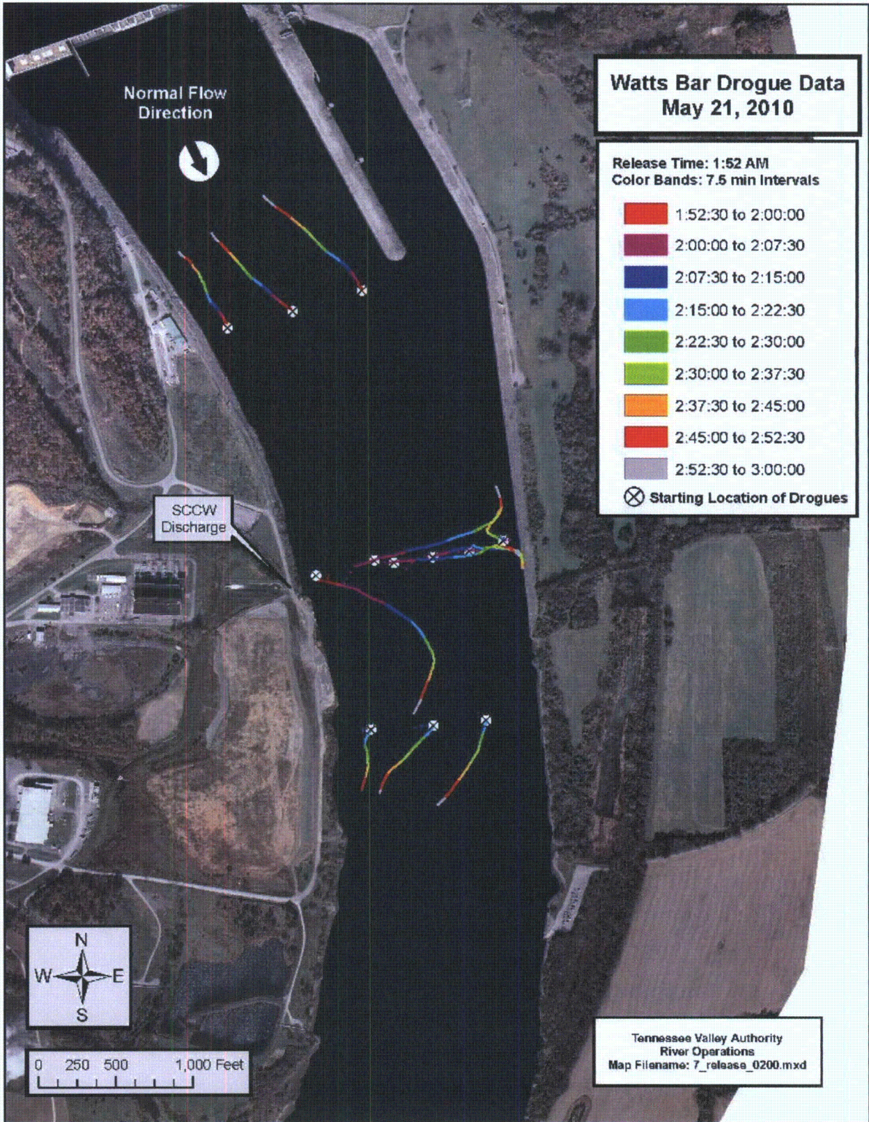
Figure 11. Drogue paths by time at WBN, 1:52 AM to 3:00 AM (third release of nighttime test) May 21, 2010.
