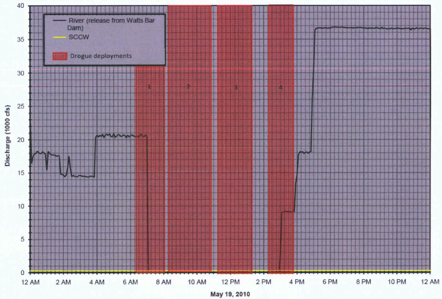
Figure 3. Drogue release times and flow at WBN for daytime test on May 19, 2010.
