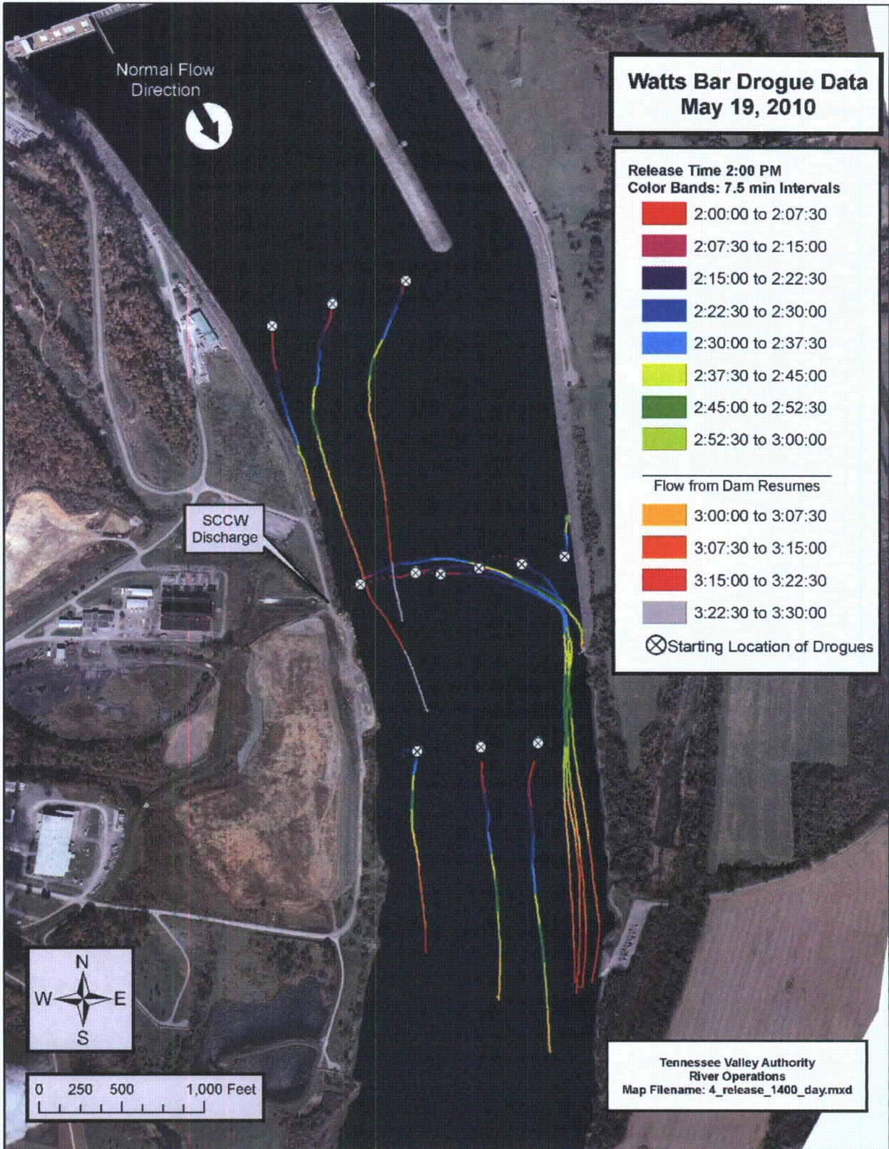
Figure 7. Drogue paths by time at WBN, 2:00 PM to 3:30 PM (fourth and final release of daytime test) May 19, 2010.
