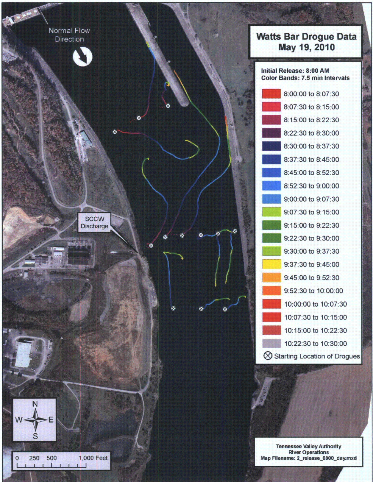
Figure 5. Drogue paths by time at WBN, 8:00 AM to 10:30 AM (second release of daytime test) May 19, 2010.
