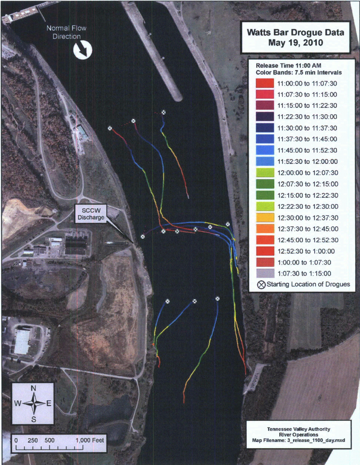
Figure 6. Drogue paths by time at WBN, 11:00 AM to 1:15 PM (third release of daytime test) May 19, 2010.
