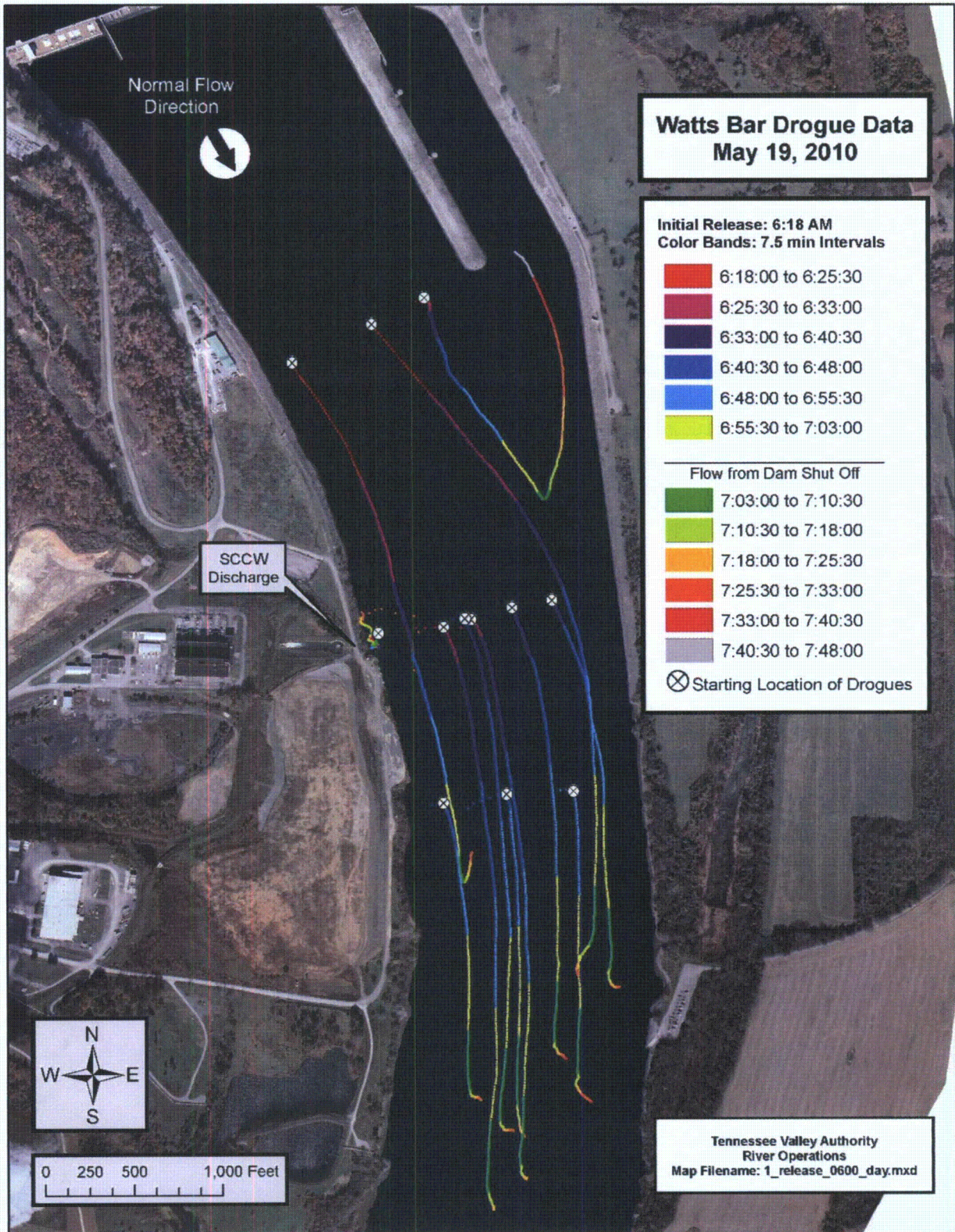
Figure 4. Droge paths by time at WBN, 6:00 AM to 7:48 AM (first release of daytime test) May 19, 2010.
