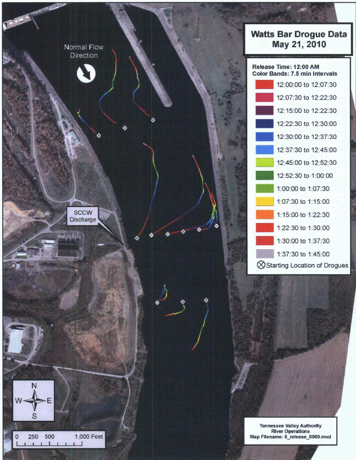
Figure 10. Drogue paths by time at WBN, midnight to 1:45 AM (second release of nighttime test) May 21, 2010.
