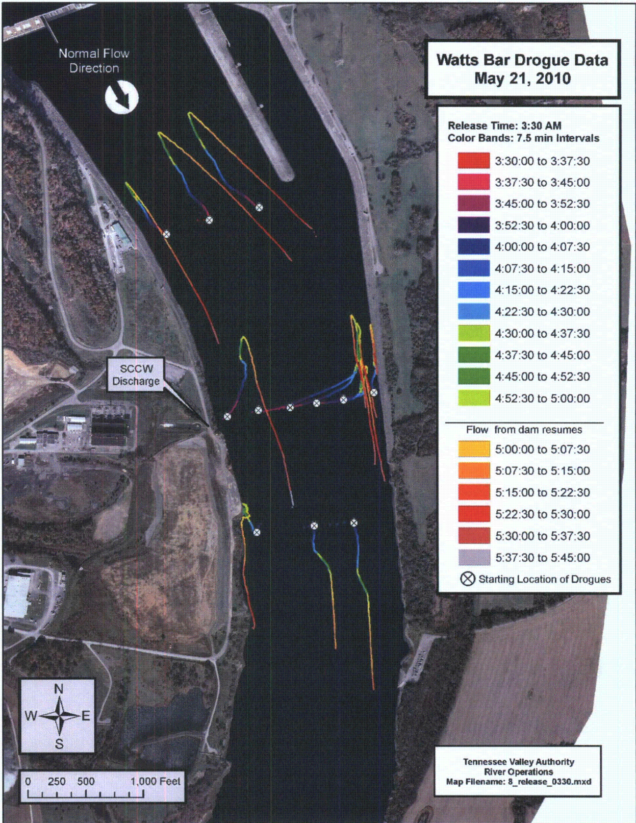
Figure 12. Drogue paths by time at WBN, 3:30 AM to 5:45 AM (fourth and final release of nighttime test) May 21, 2010.
