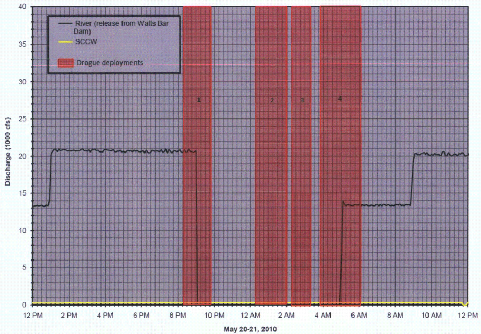
Figure 8. Drogue release times and flow for nighttime test, May 20-21 at WBN.
