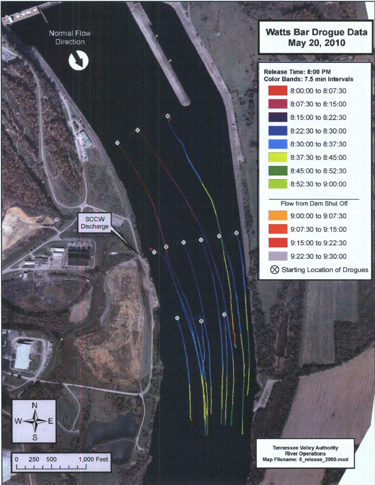
Figure 9. Drogue paths by time at WBN, 8:00 PM to 9:30 PM (first release of nighttime test) May 20, 2010.
