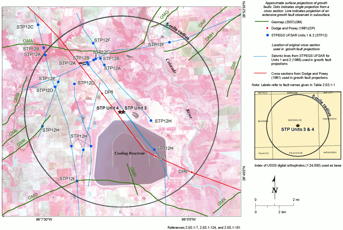
Figure 2.5S.1-43 Site Vicinity (5-mile radius) Growth Fault Surface Projections
