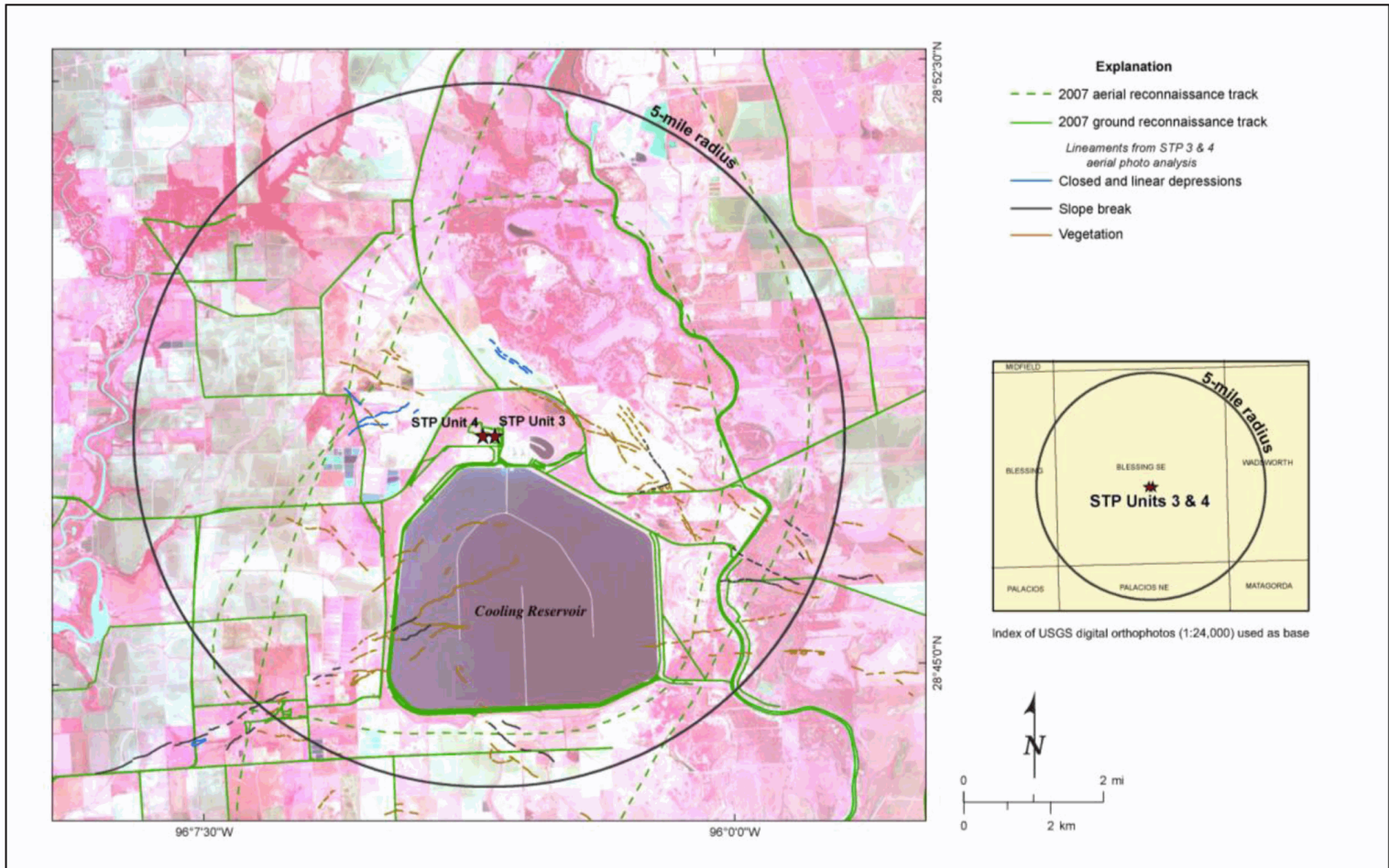
Figure 2.5S.1-44 Lineaments and Aerial Photographs
