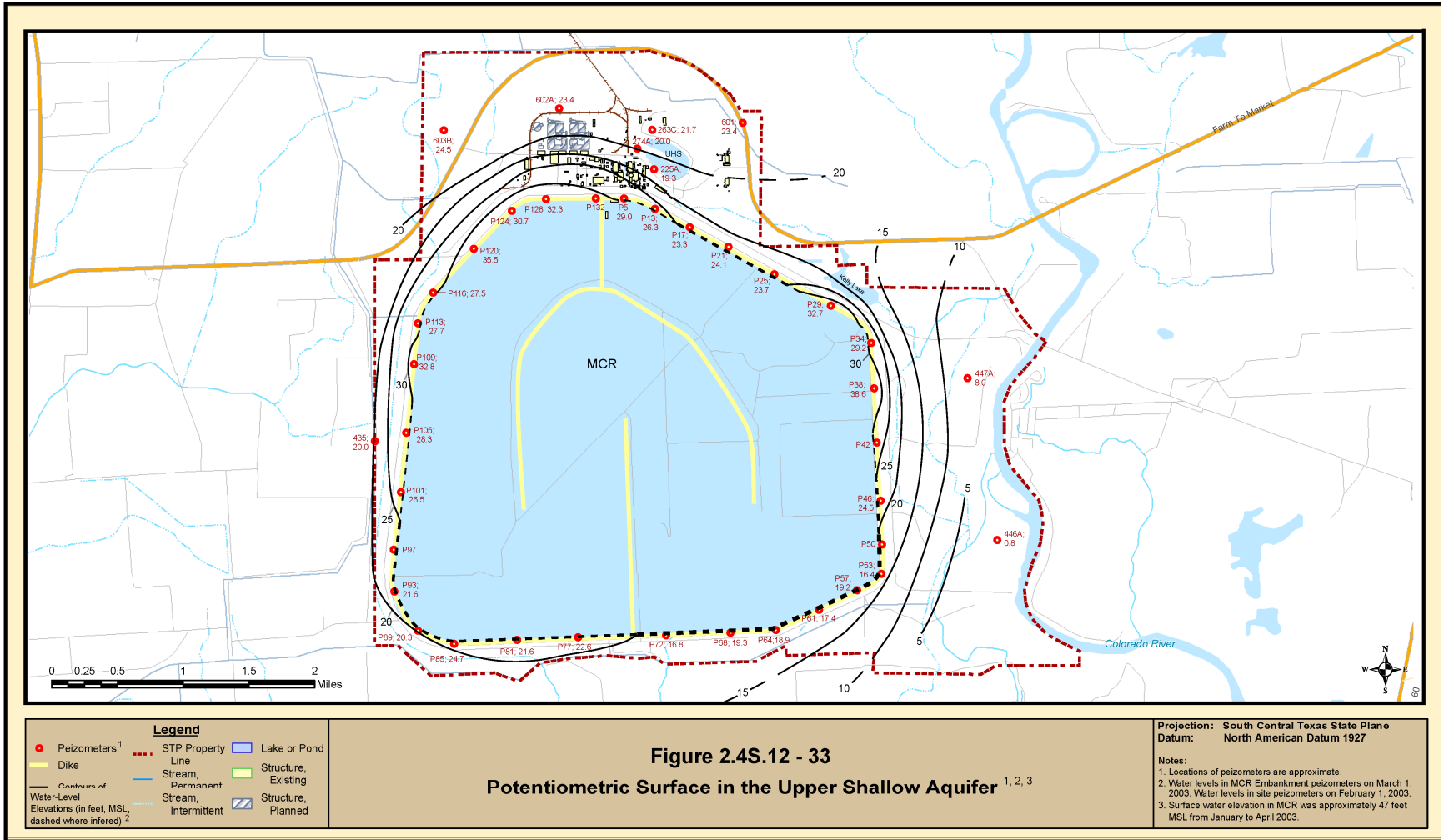
Figure 2.4S.12-33 Potentiometric Surface in the Upper Shallow Aquifer
