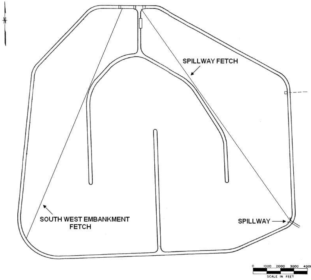
Figure 2.4S.8-4 Determination of Fetch at the Spillway and at the South West Embankment
