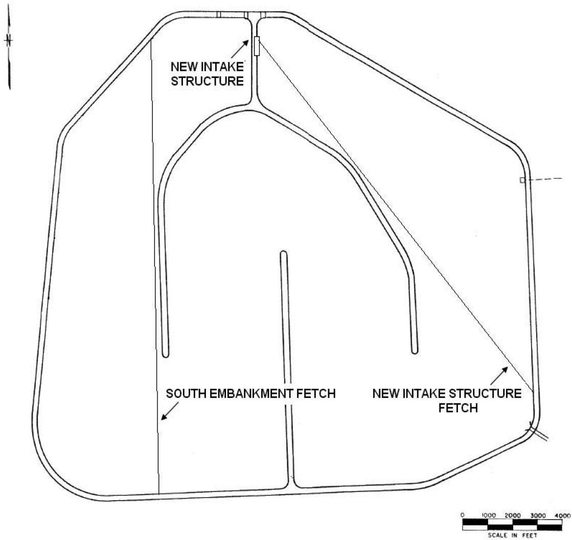
Figure 2.4S.8-2 Determination of Fetch at the New Intake Structure and at the South Embankment
