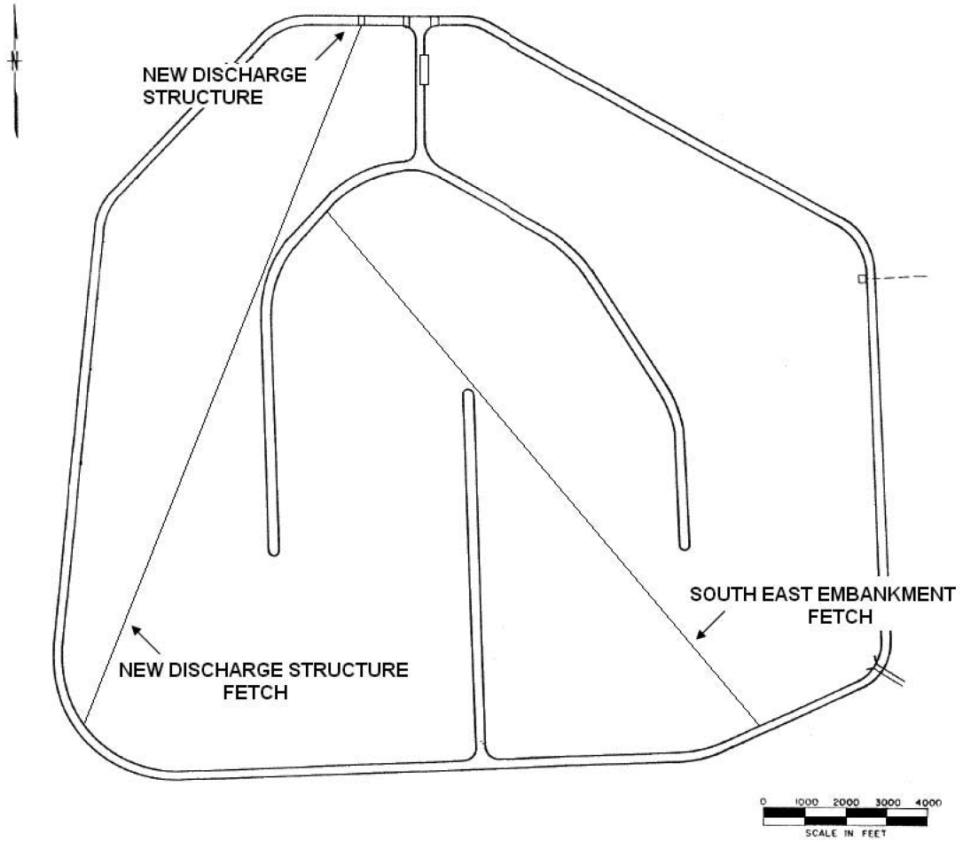
Figure 2.4S.8-5 Determination of Fetch at the Southeast Embankment and at the New Discharge Structure
