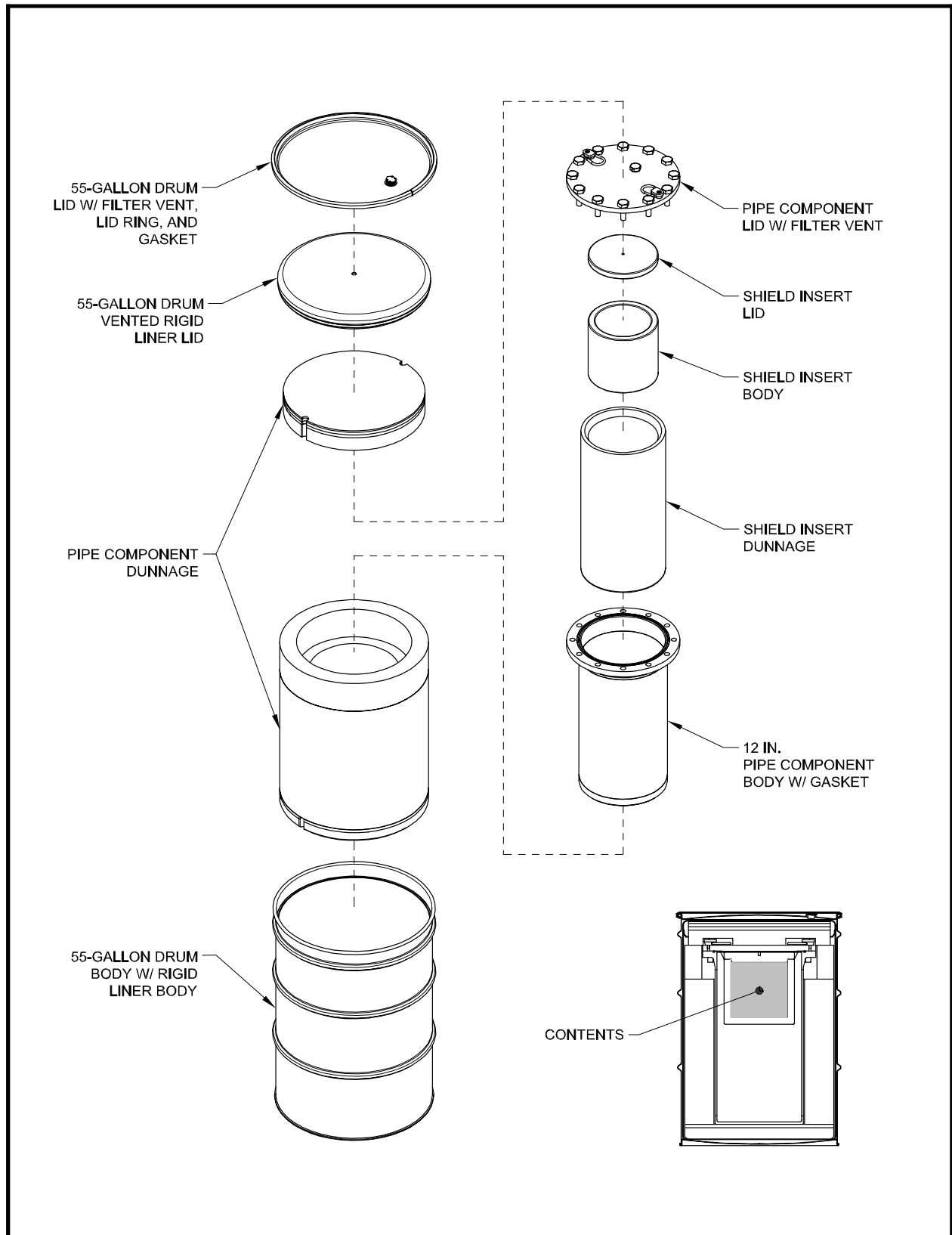
Figure 2.9-6 – S200 Pipe Overpack
