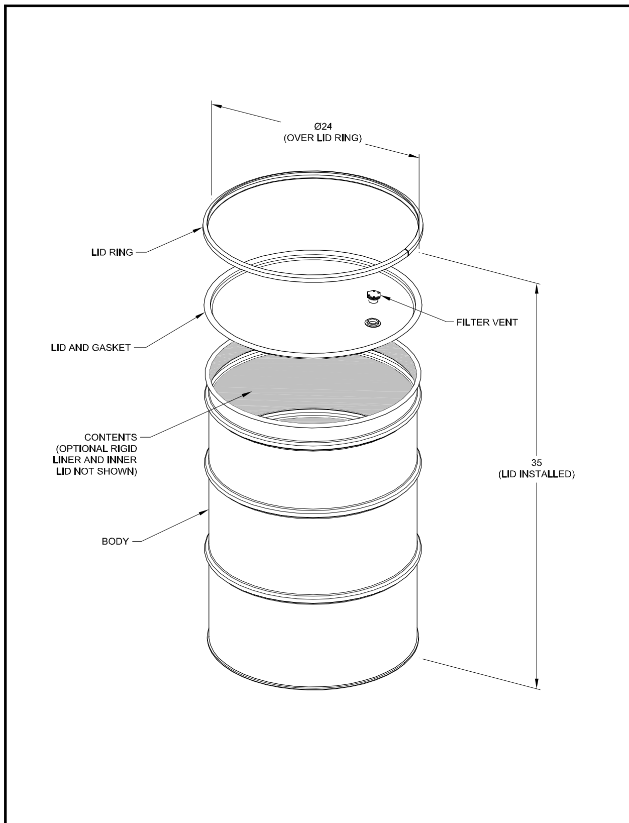
Figure 2.9-1 – 55-Gallon Drum
