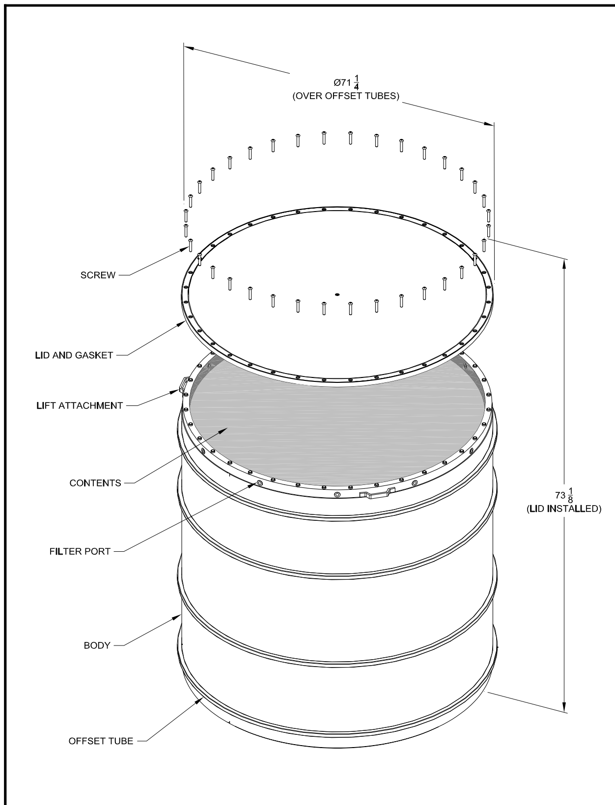
Figure 2.9-19 – Ten-Drum Overpack
