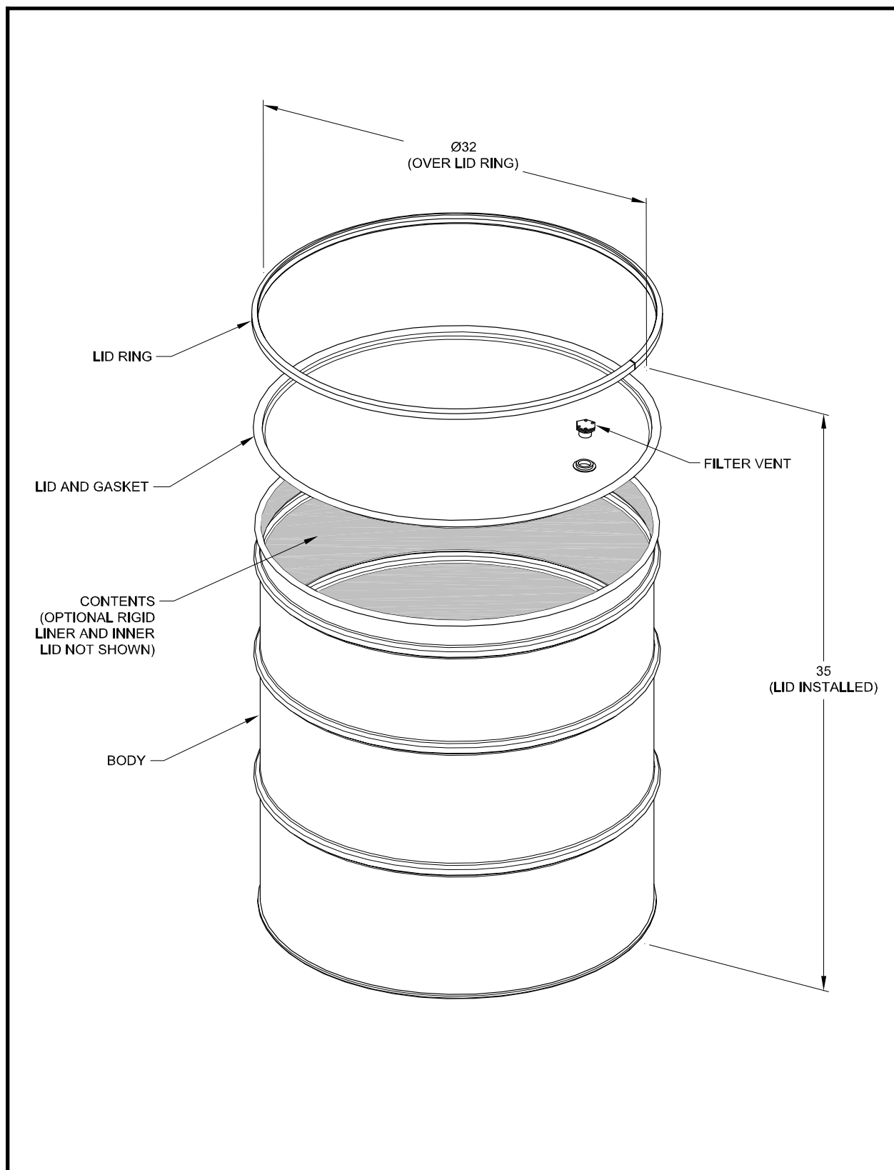
Figure 2.9-13 – 100-Gallon Drum
