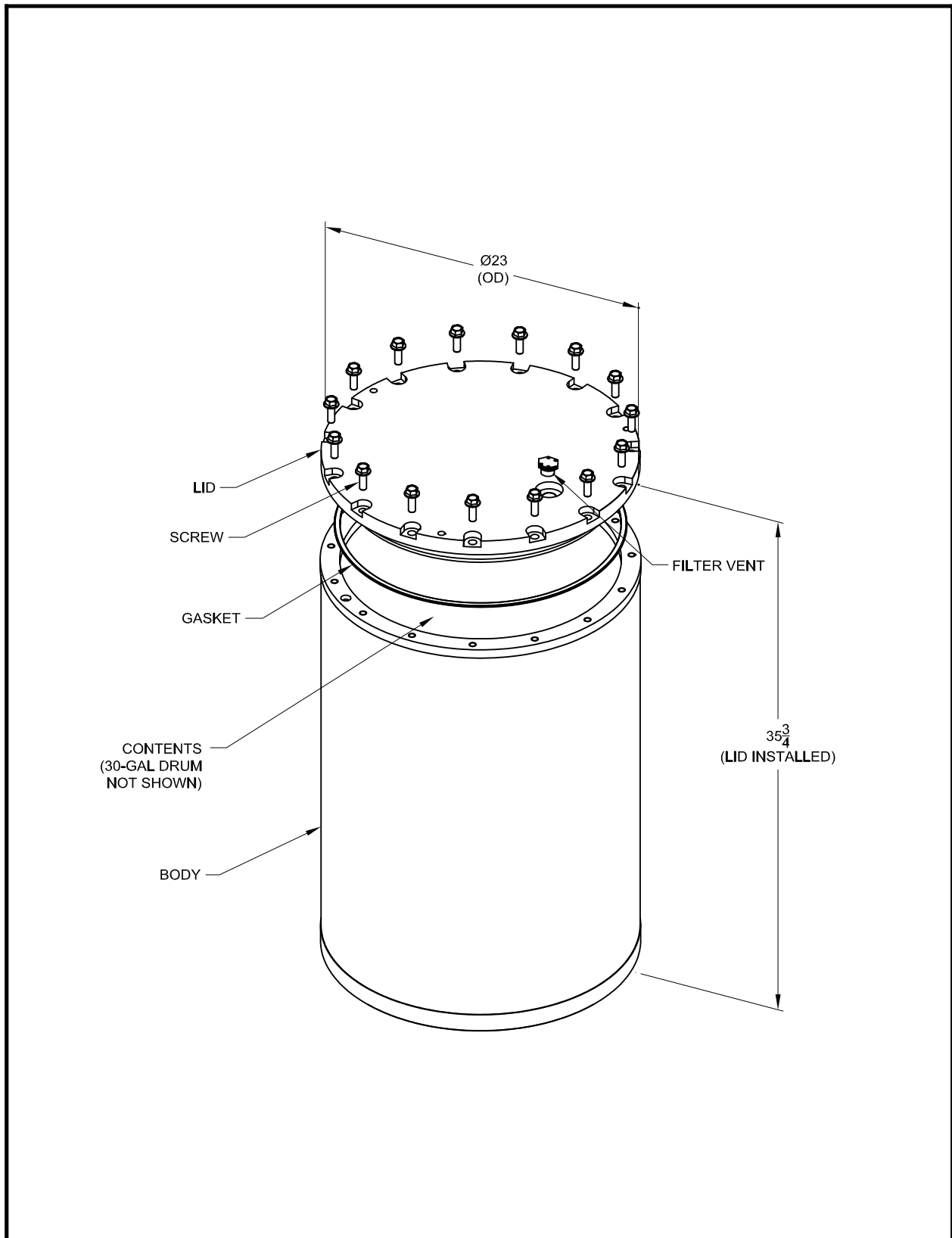
Figure 2.9-21 – Shielded Container
