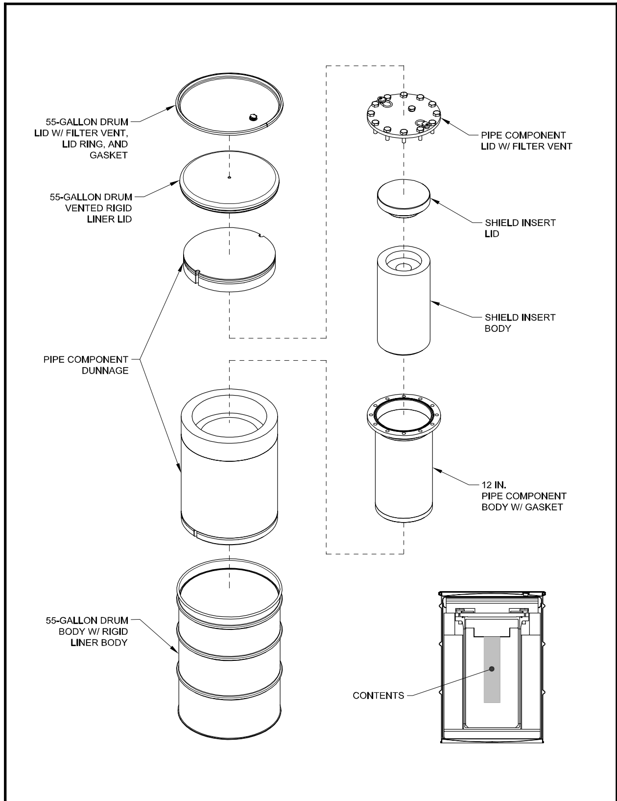
Figure 2.9-7 – S300 Pipe Overpack
