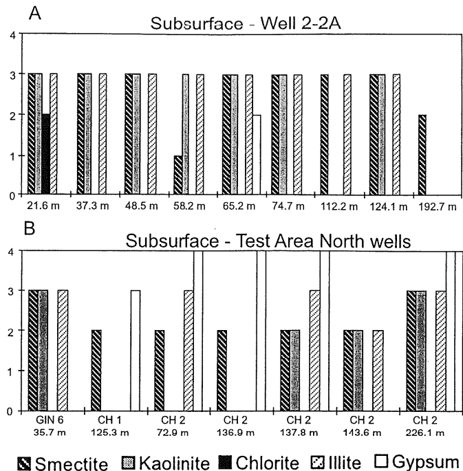
Figure 8. Semiquantitative mineralogy of fine-grained fraction of subsurface deposits determined using X-ray diffraction analyses for samples from well 2-2A, in middle of basin, and from wells at Test Area North, along northeastern margin of basin. Ranking from 0 to 4 indicates relative abundance of mineral: 4 = mineral dominant in sample, 3 = mineral present in sample, 2 = trace amounts of mineral in sample, 1 = mineral possibly present in sample.
