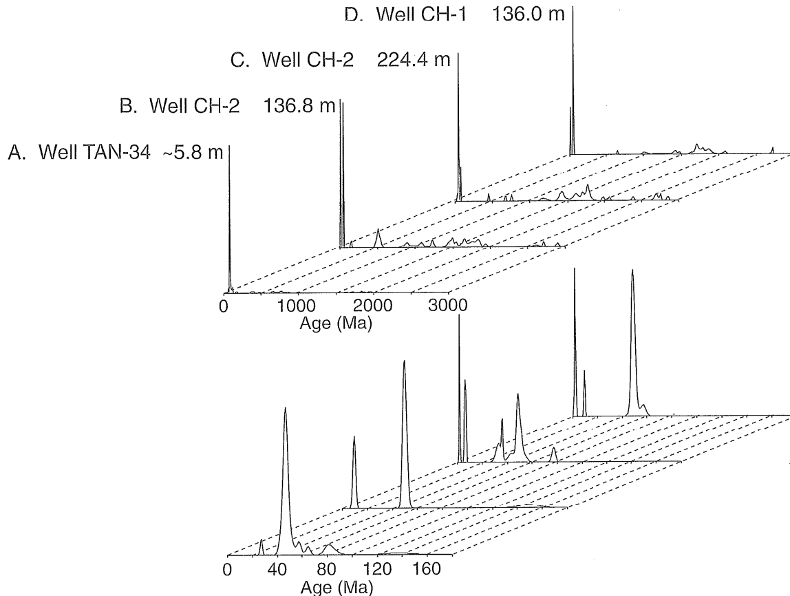
Figure 6. Relative probability plots for detrital-zircon ages determined for subsurface sands from wells at Test Area North, along northeastern margin of Big Lost Trough (Fig. 1). Upper graphs contain results of all analyses (0–3000 Ma zircons); lower graphs are for young (<180 Ma) zircon populations.
