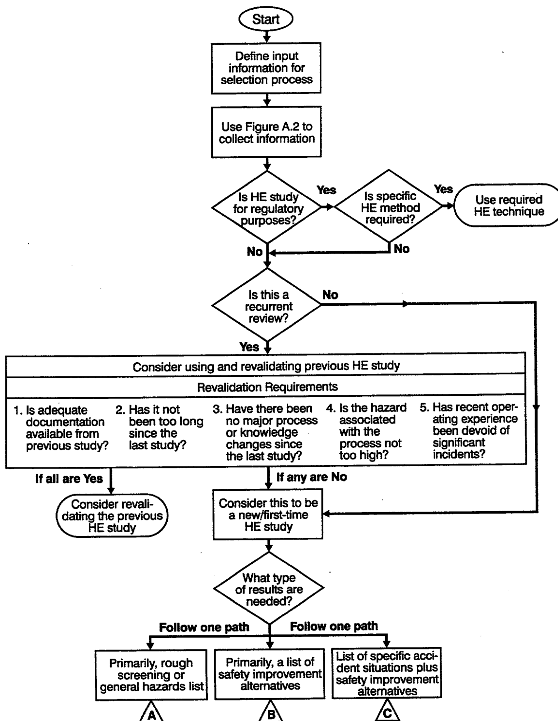
Figure A.1. Example flowchart for selecting an HE technique.
