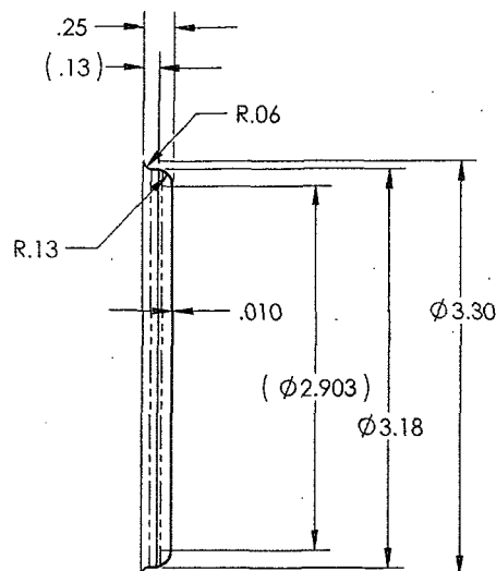
SECTION F-F
