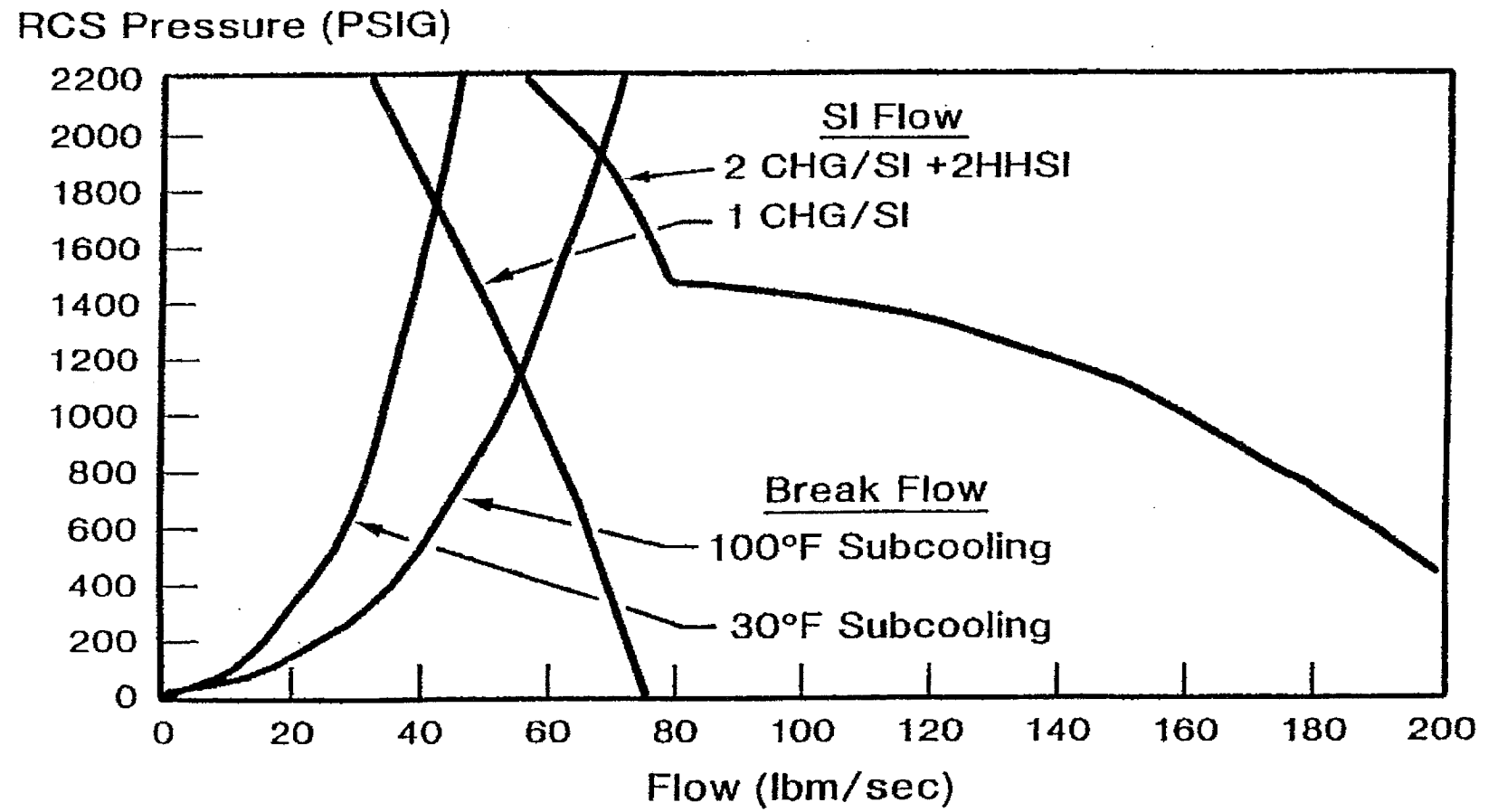
Figure 16. EQUILIBRIUM RCS PRESSURE
