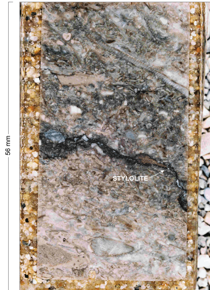
BLN-11 Fossiliferous limestone (packstone); fossils are undeformed
