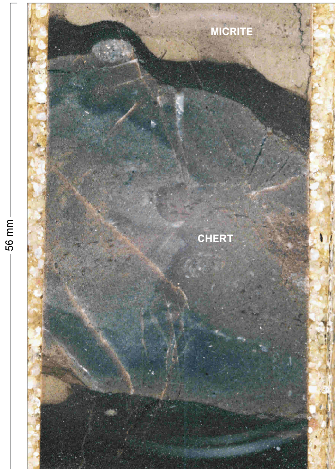
BLN-8 Limestone (micrite) with chert nodule
