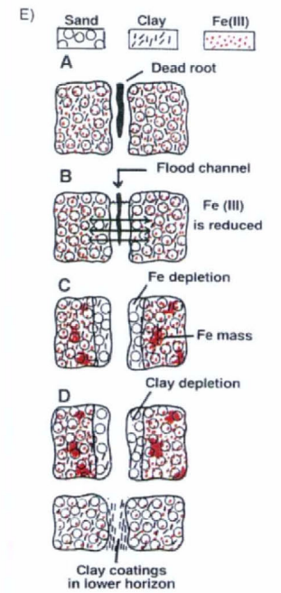
Formation of Fe-Depleted "Bleached" Zones Source: Reference 480
