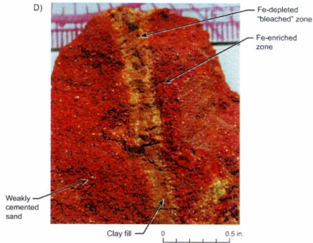
Formation of Fe-Depleted "Bleached" Zones Source: Reference 480
