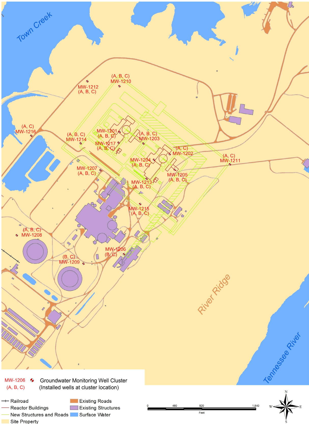
FIGURE 2.4.12-212 (Sheet 1 of 2) Groundwater Monitoring Well Location Map
