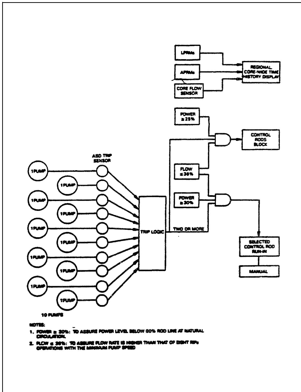
Figure 20.3.7-1 Stability Controls and Protection Logic (Response to Question 100.1)
