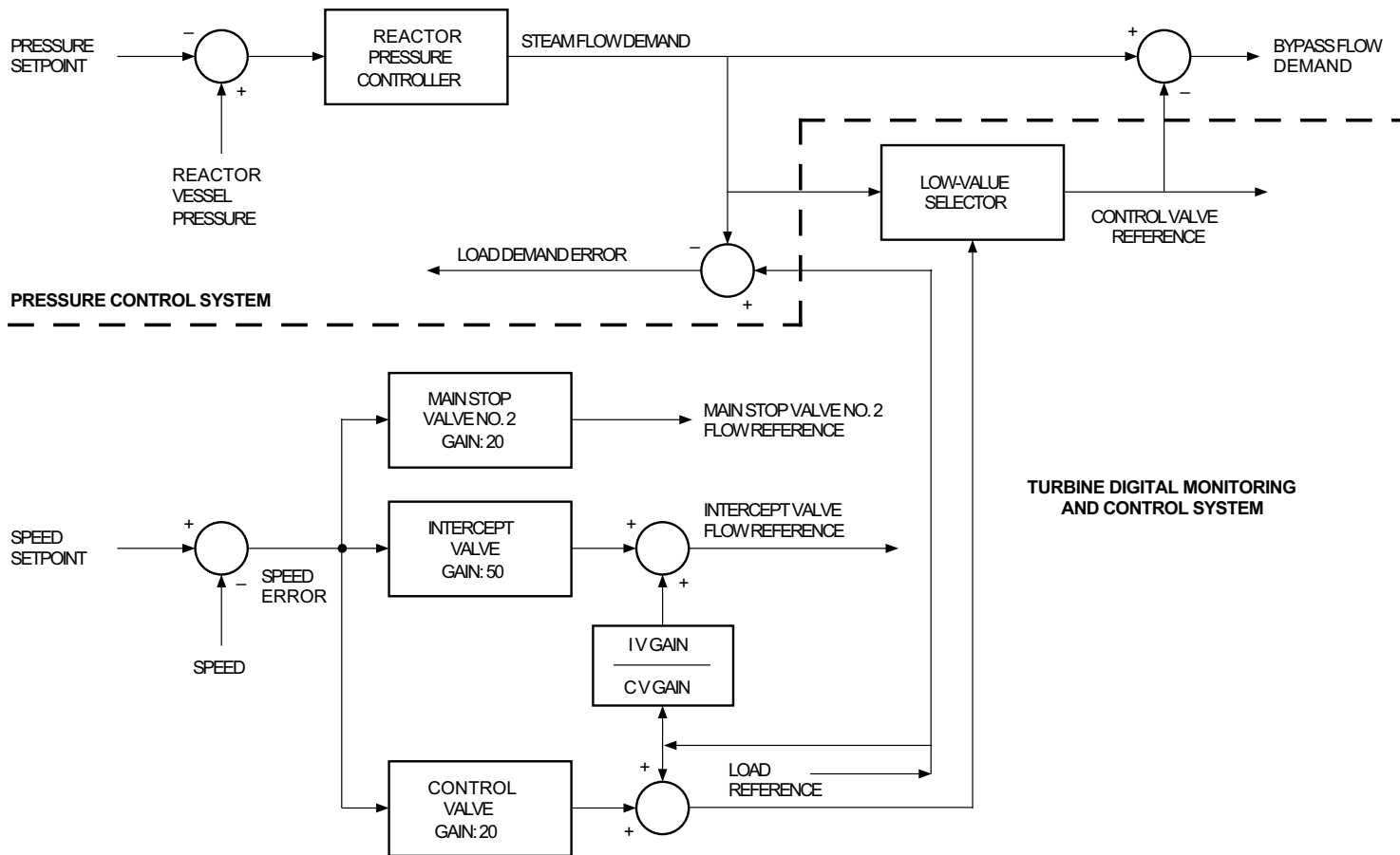
Figure 20.3.10-1 Simplified Functional Control Diagram of Turbine Digital Control and Monitoring System (Typical of One of Three Channels)
