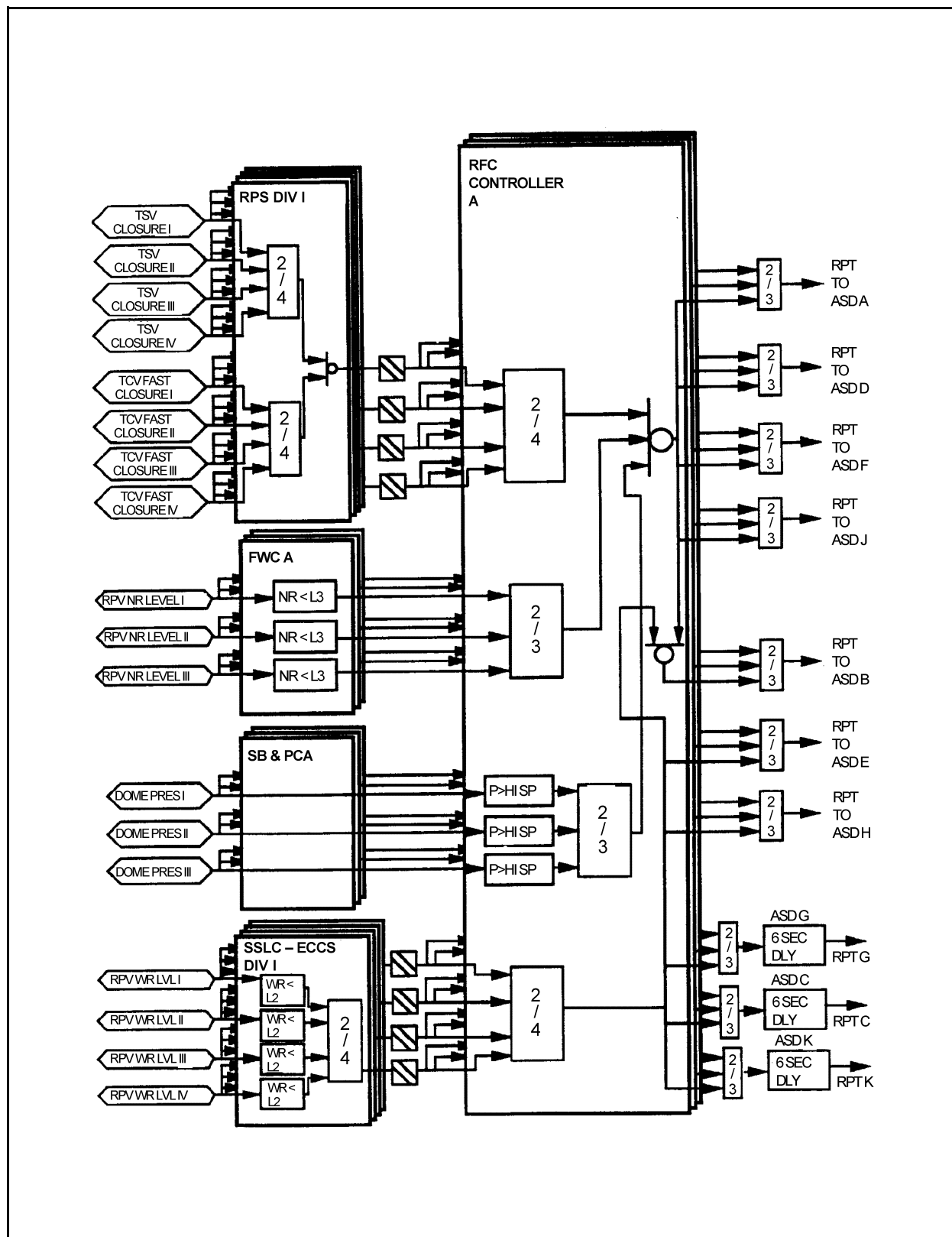
Figure 20.3.8-1 ABWR RPT Logic (Response to Question 420.106)
