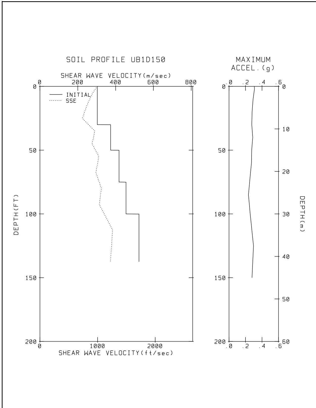
Figure 20.3.3-1 Shake Analysis Results – Soil Profile UB1D150 (Response to Question 220.8)
