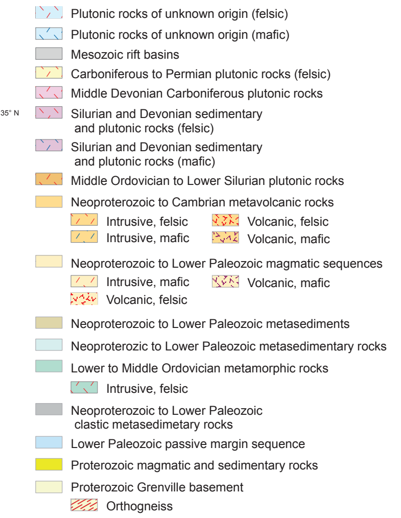
WILLIAM STATES LEE III NUCLEAR STATION UNITS 1 & 2 Tectonic Features and Seismicity Within 50 Miles of the Site FIGURE 2.5.1-210 Rev 2
