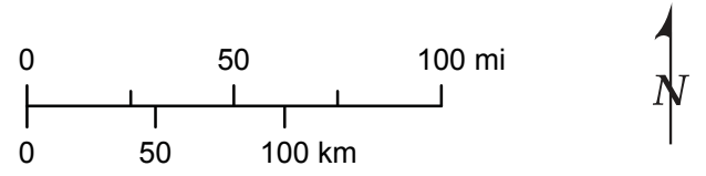
WILLIAM STATES LEE III NUCLEAR STATION UNITS 1 & 2 Site Region Tectonic Features FIGURE 2.5.1-209 Rev 2
