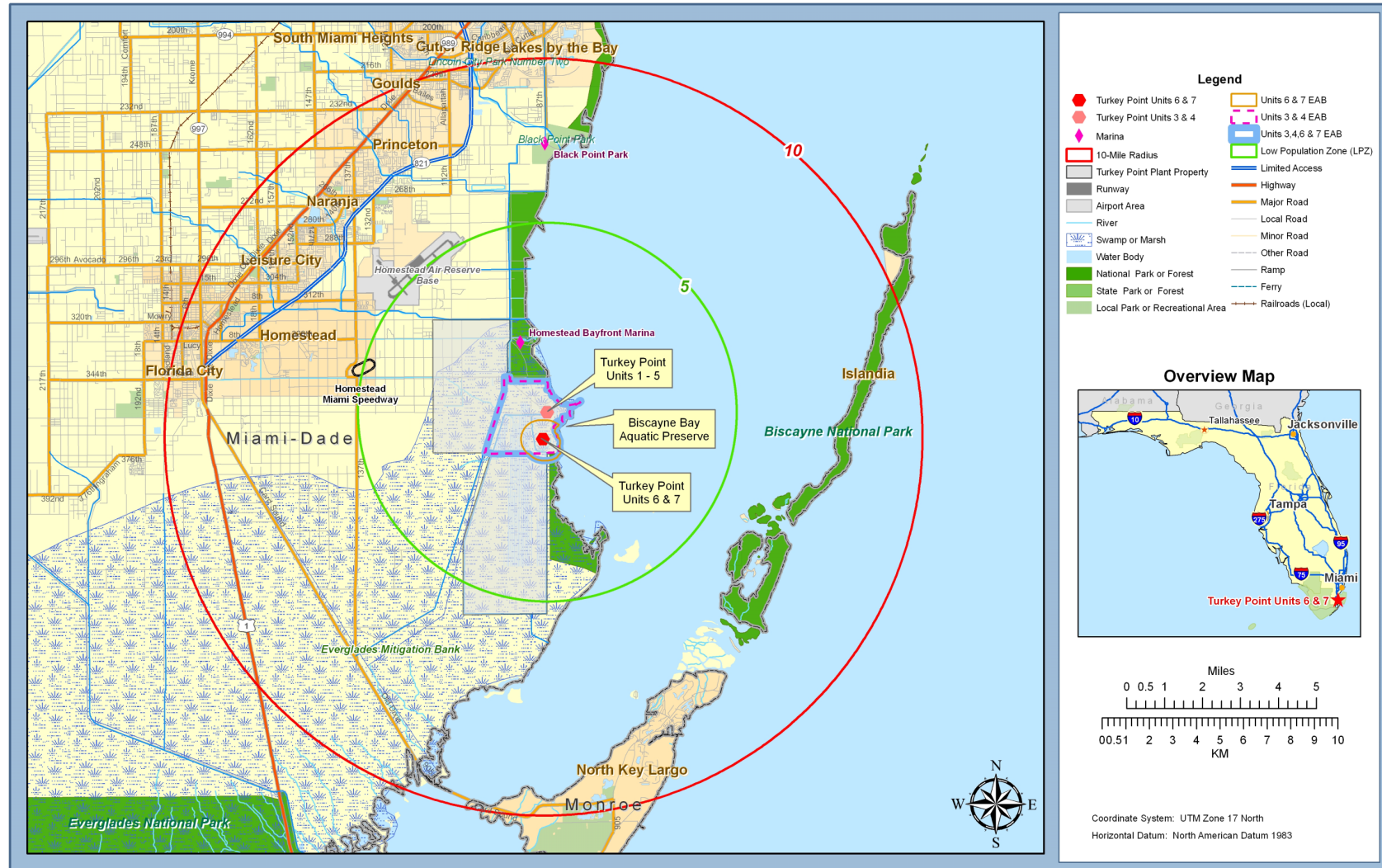
FIGURE 4.1-1 Low Population Zone and Site Boundary Map
