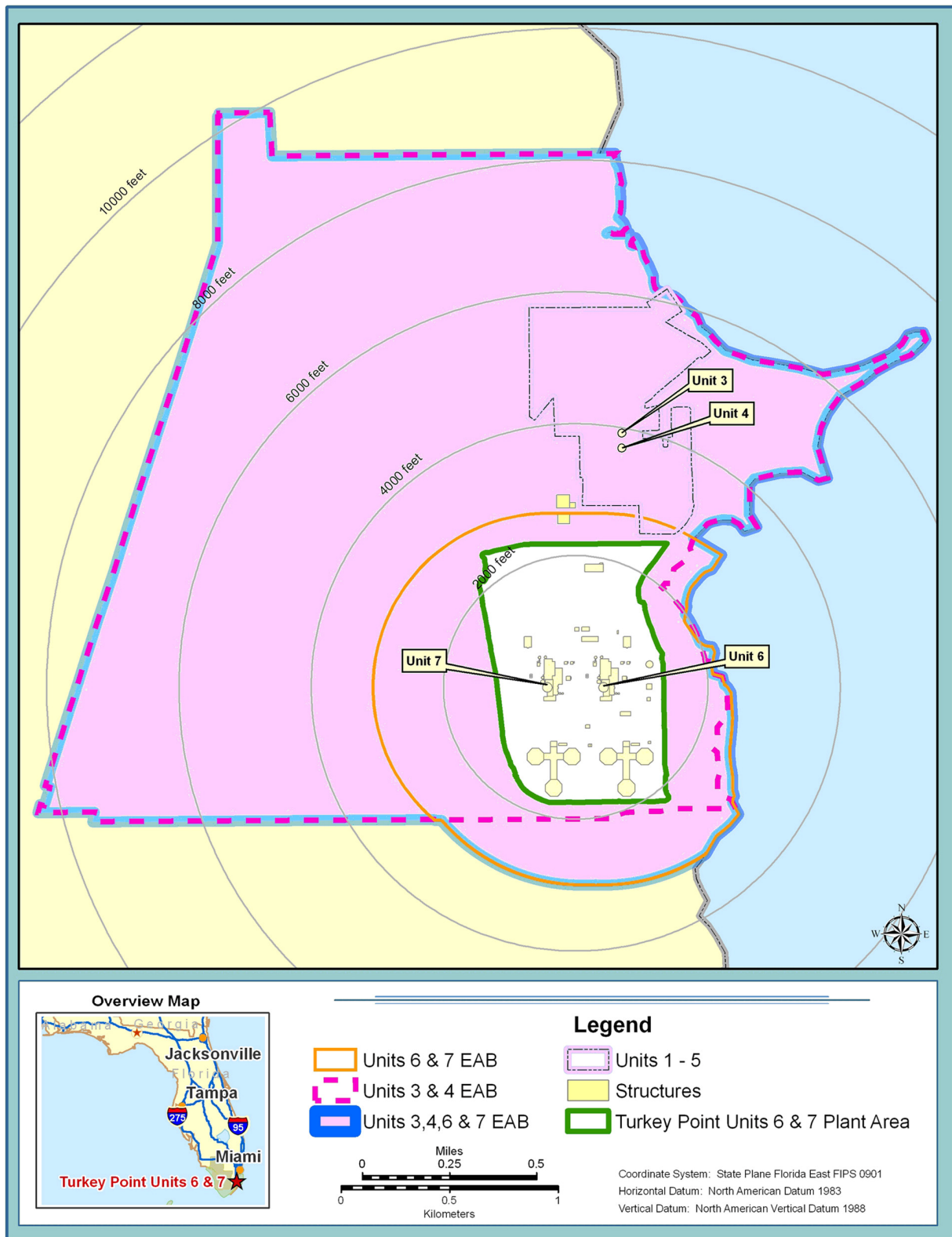
FIGURE 4.1-2 Exclusion Area Boundary
