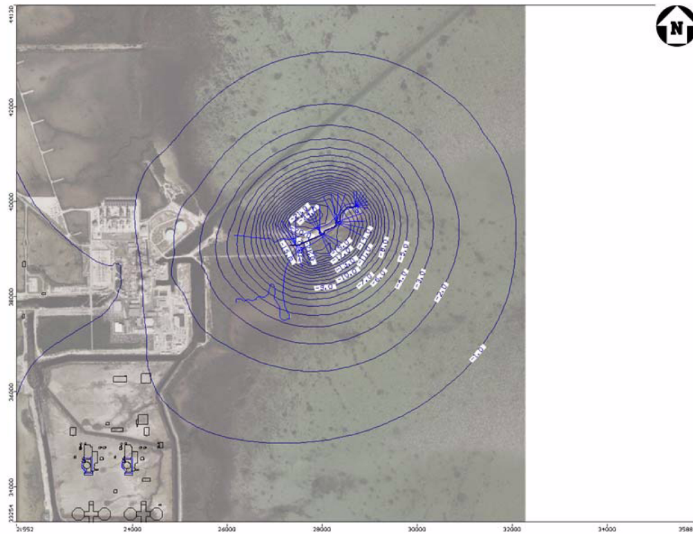
Figure 5.2-1 Groundwater Contours within Key Largo Limestone in Vicinity of Radial Collector Wells
