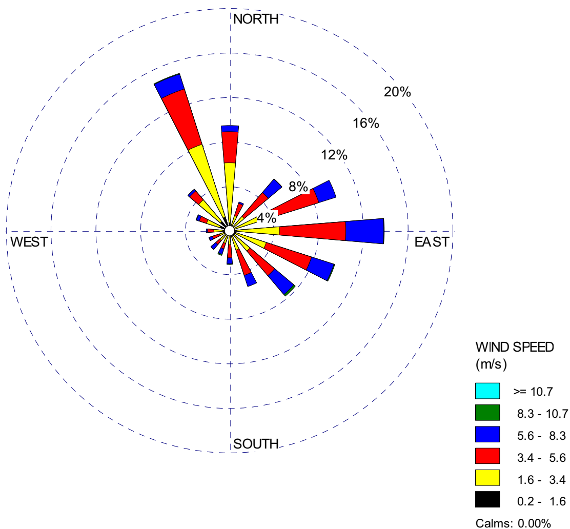
Figure 2.7-3 10-Meter Level 3-Year Composite Wind Rose — Winter (2002, 2005, and 2006)
