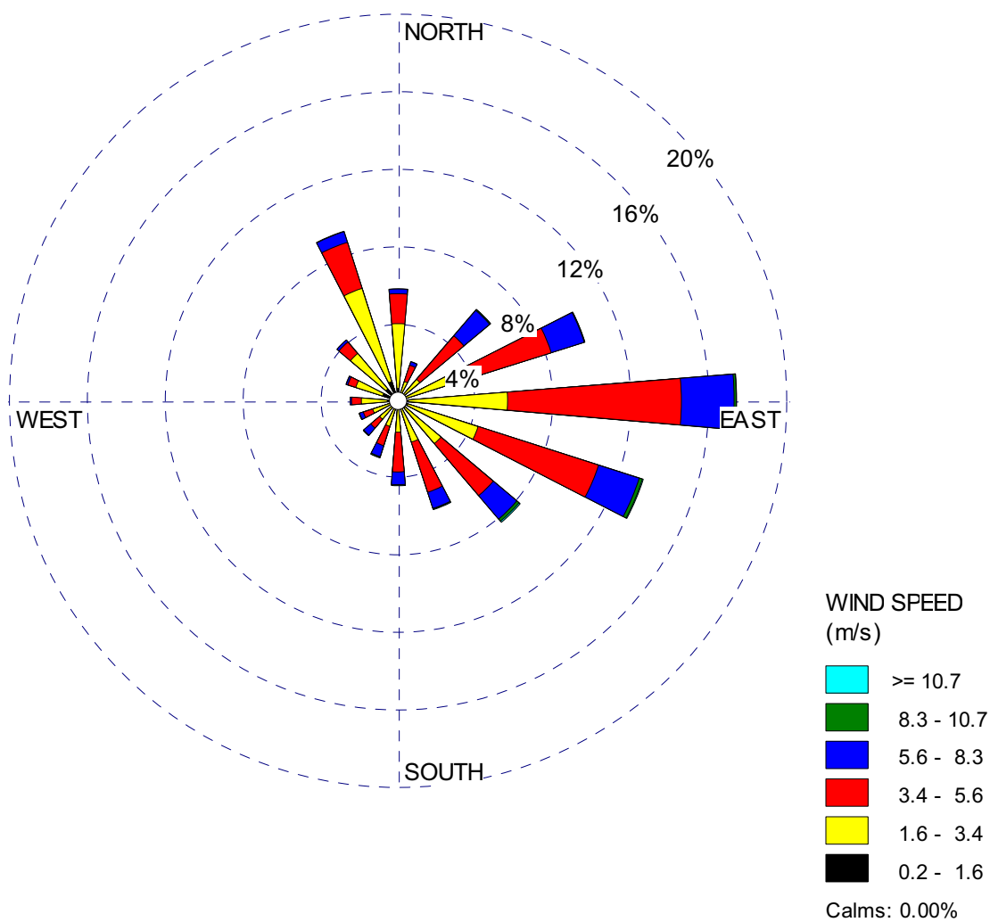
Figure 2.7-2 10-Meter Level 3-Year Composite Wind Rose — Annual (2002, 2005, and 2006)
