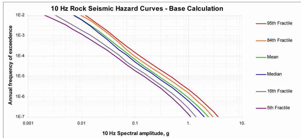
Figure 2.5.2-220 Mean and Fractile Rock 10 Hz Seismic Hazard Curves, Rock
