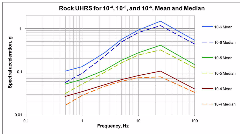
Figure 2.5.2-225 Mean and Median Rock UHRS for 1E-04, 1E-05, and 1E-06
