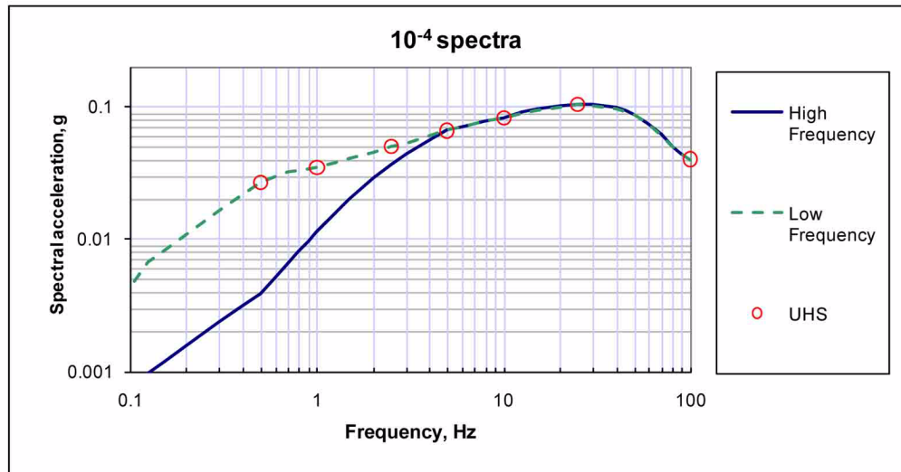
Figure 2.5.2-232 HF and LF Rock Spectra Anchored to Mean UHS Values from Hazard Calculation for 1E-04 Spectra
