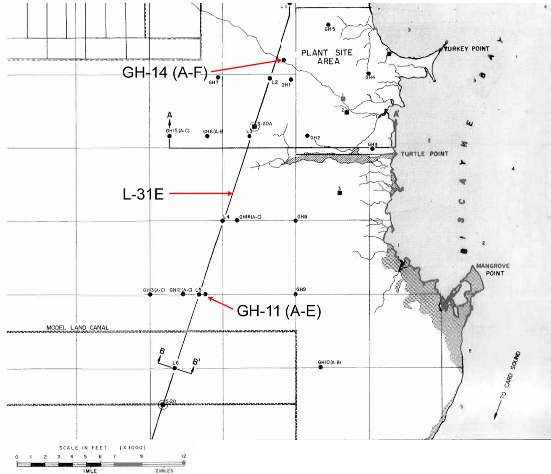
Figure 2CC-201 Cross Section Location
