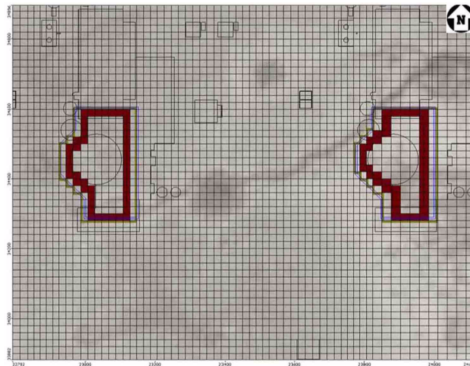
Figure 2CC-224 Location of Units 6 & 7 Cut-Off Walls and Internal Dewatering Wells
