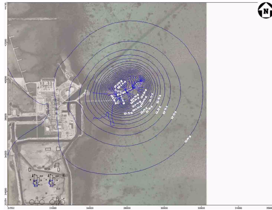
Figure 2CC-234 Groundwater Contours within Key Largo Limestone in Vicinity of Radial Collector Wells
