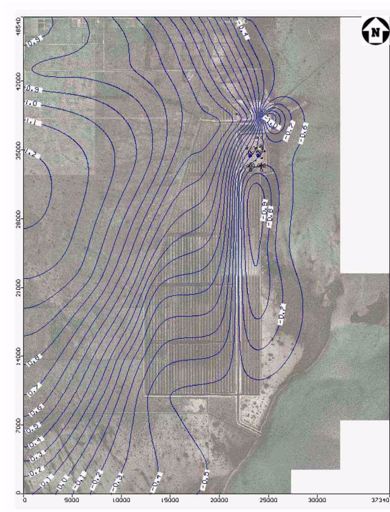
Figure 2CC-219 Simulated Groundwater Contours — Model Layer 6 — Tamiami Formation
