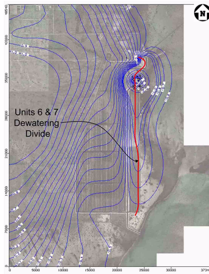
Figure 2CC-230 Groundwater Contours in Fort Thompson Formation for Dewatering of Units 6 & 7 Excavations
