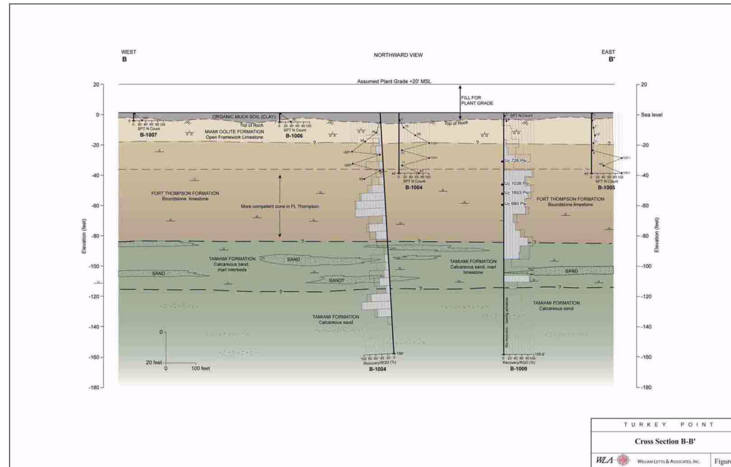
Figure 2CC-206 Stratigraphic Cross Section B-B'
