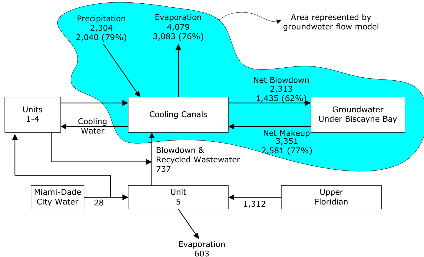
Figure 2CC-220 Cooling Canals Water Balance — Comparison with Groundwater Model
