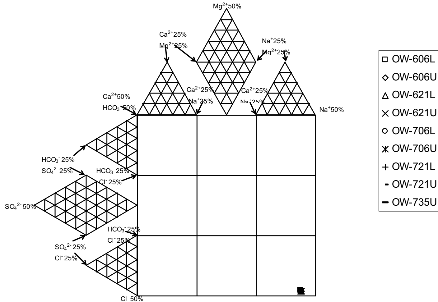
Figure 2CC-208 Expanded Durov Plot of Units 6 & 7 Observation Wells
