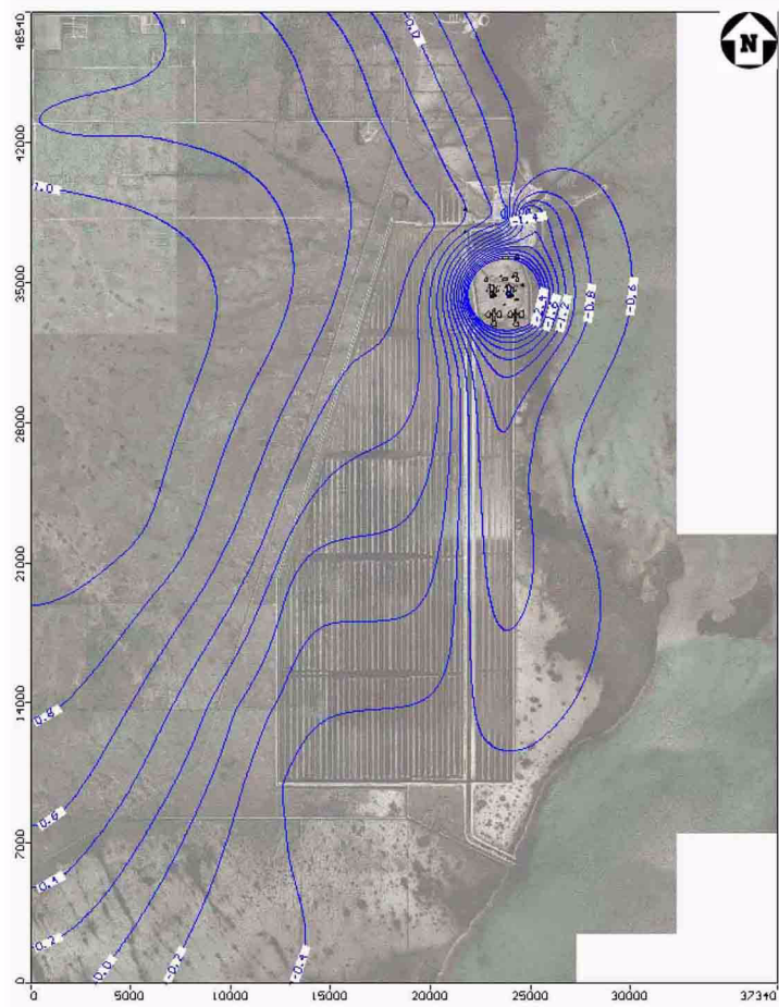
Figure 2CC-229 Construction Dewatering: Simulated Groundwater Contours — Fort Thompson Formation (Upper Portion)
