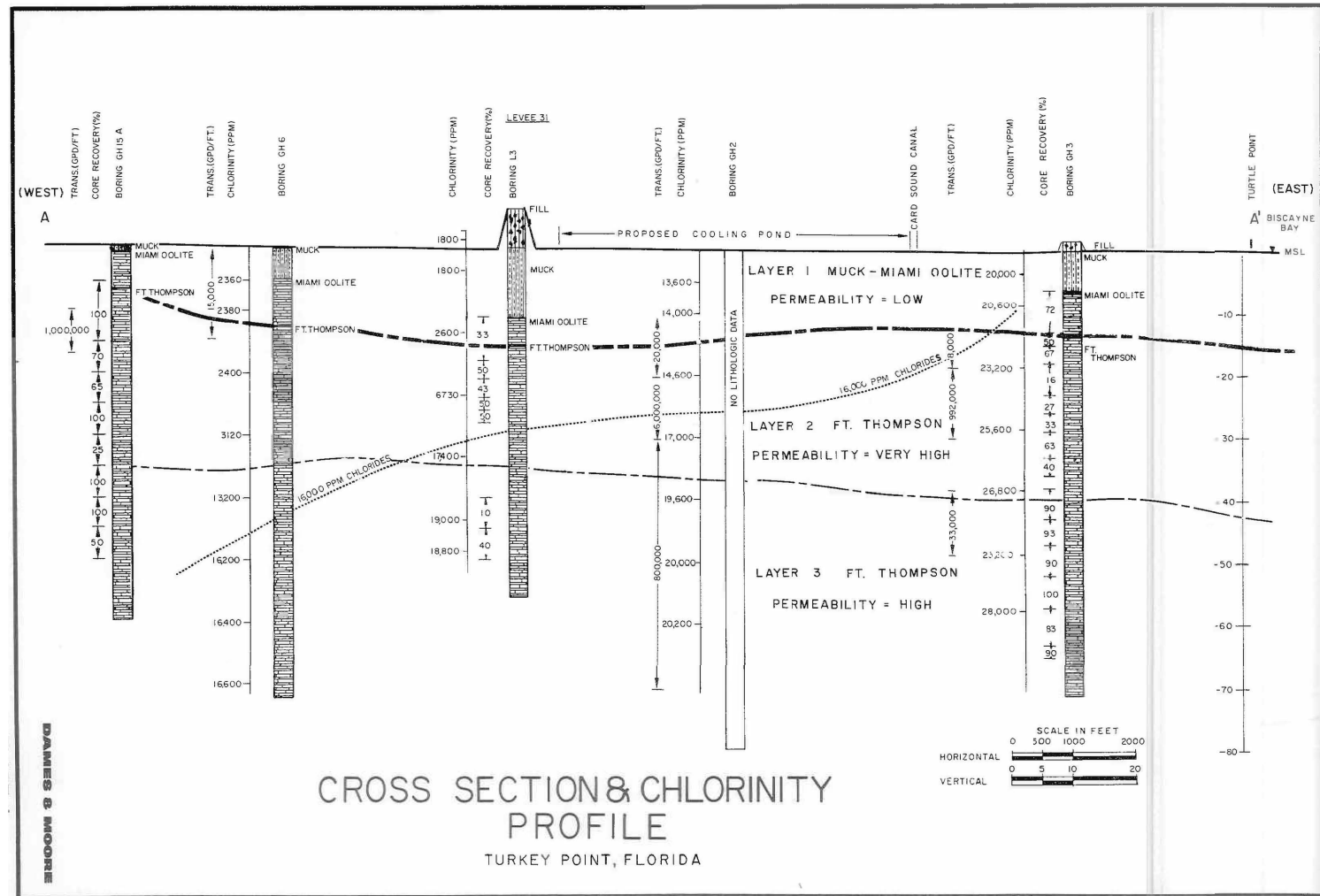
Figure 2CC-202 Hydrostratigraphic Cross Section A-A'
