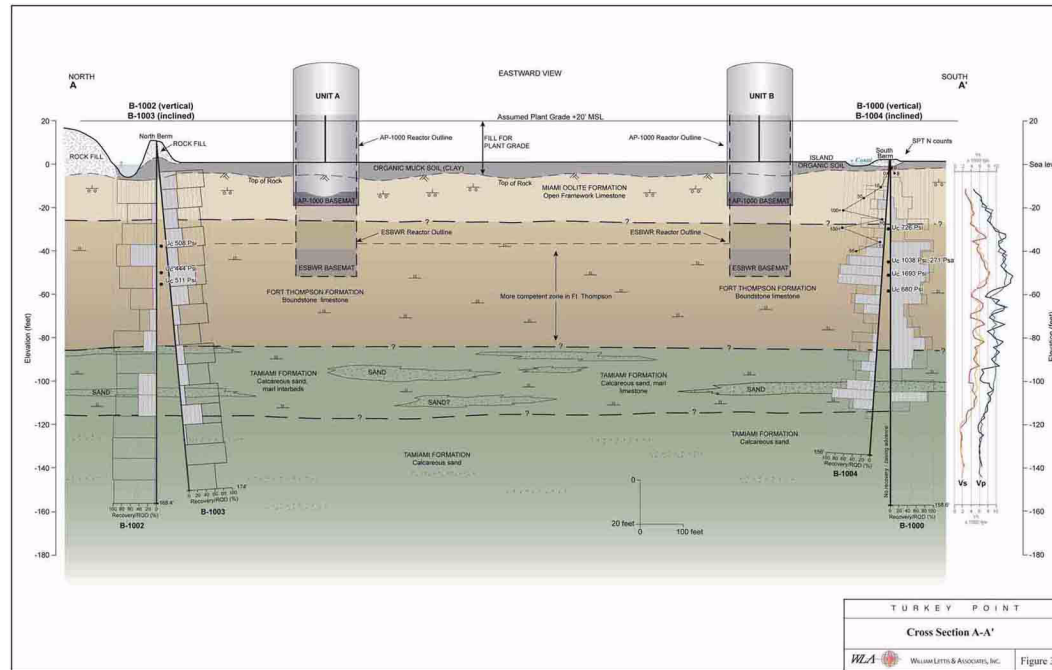
Figure 2CC-205 Stratigraphic Cross Section A-A'
