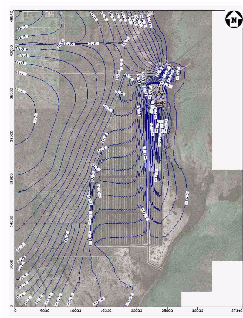
Figure 2CC-215 Simulated Groundwater Contours — Model Layer 2 — Miami Limestone
