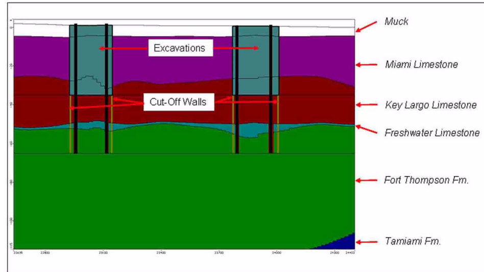
Figure 2CC-225 Cross Section of Units 6 & 7 Excavations in Numerical Model
