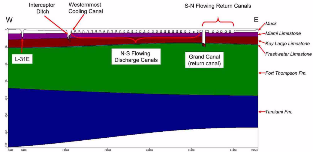
Figure 2CC-211 West-East Model Cross Section Towards Southern End of Cooling Water Canals
