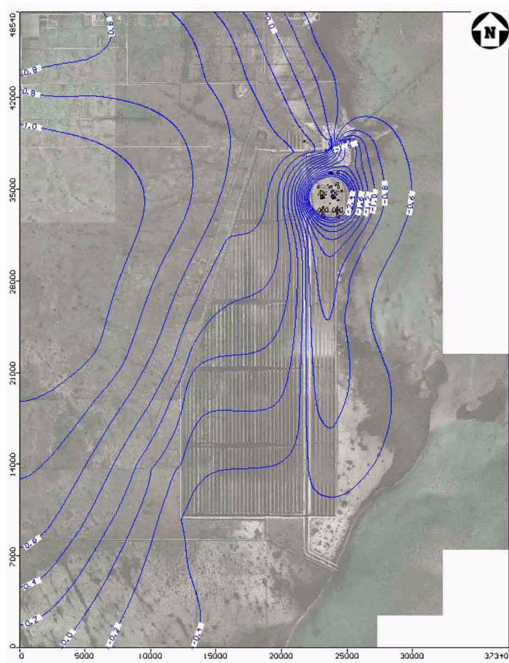
Contours — Freshwater Limestone
