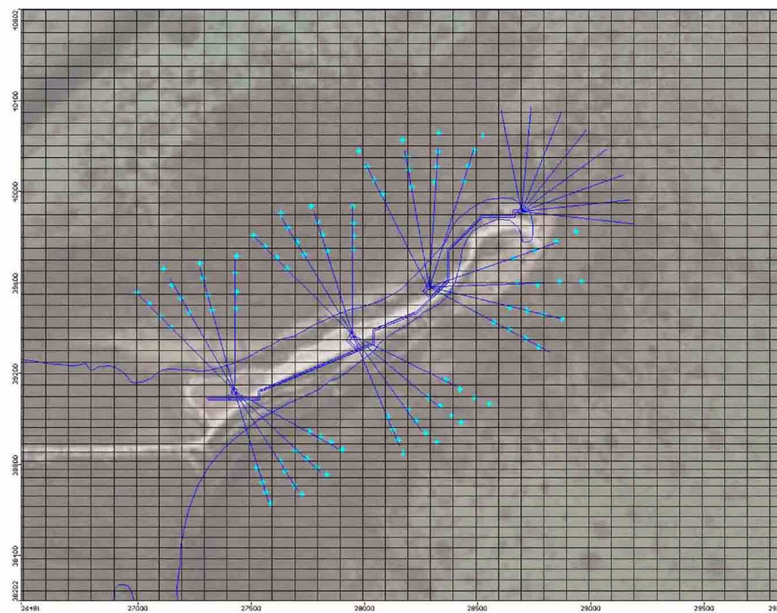
Figure 2CC-232 Location of Radial Collector Wells and Laterals, with Finite-Difference Grid and Pumping Well Locations Overlaid
