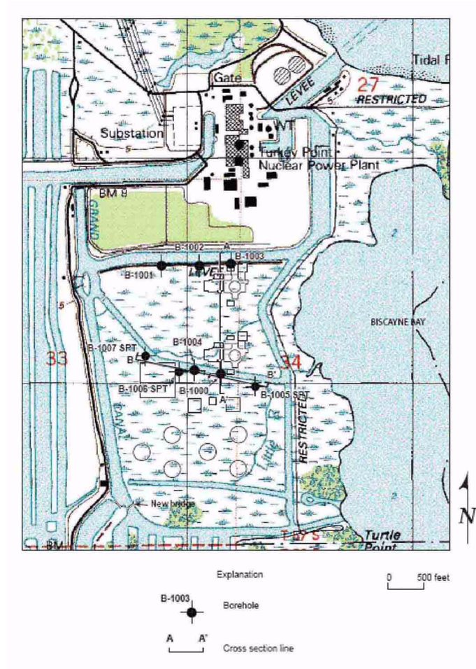
Figure 2CC-204 Boring and Stratigraphic Cross Section Locations
