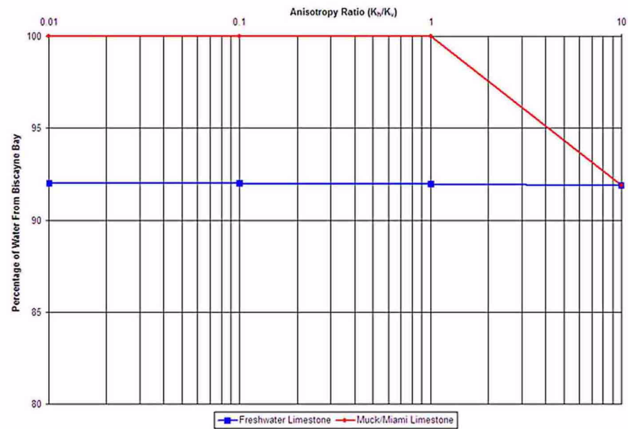
Figure 2CC-236 Radial Collector Wells Sensitivity Analysis
