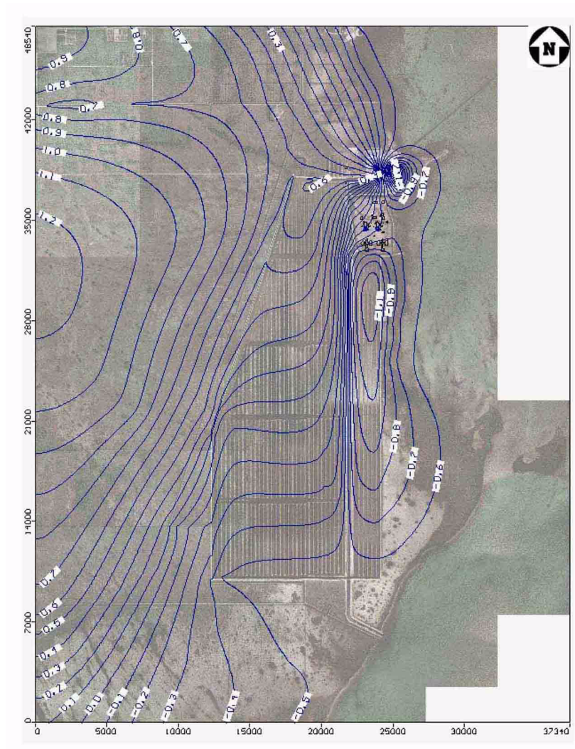
Figure 2CC-216 Simulated Groundwater Contours — Model Layer 3 — Key Largo Limestone
