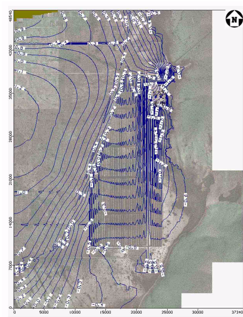
Figure 2CC-214 Simulated Groundwater Contours — Model Layer 1 — Muck
