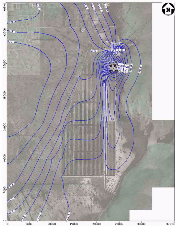
Figure 2CC-227 Construction Dewatering: Simulated Groundwater Contours — Key Largo Limestone (Lower Portion)
