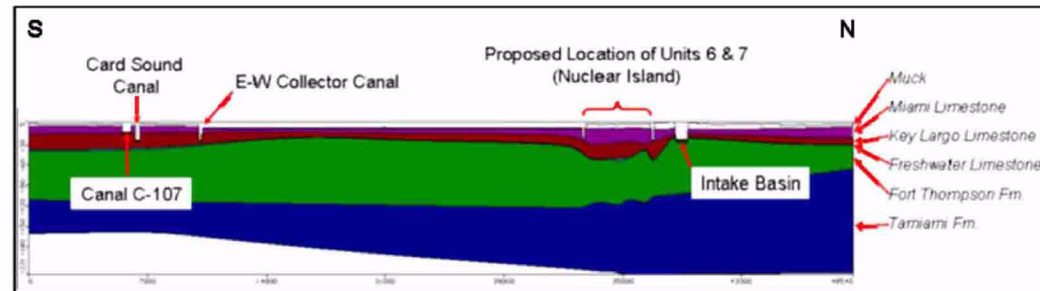
Figure 2CC-212 South-North Model Cross Section Along Return Canal of Cooling Water Canals
