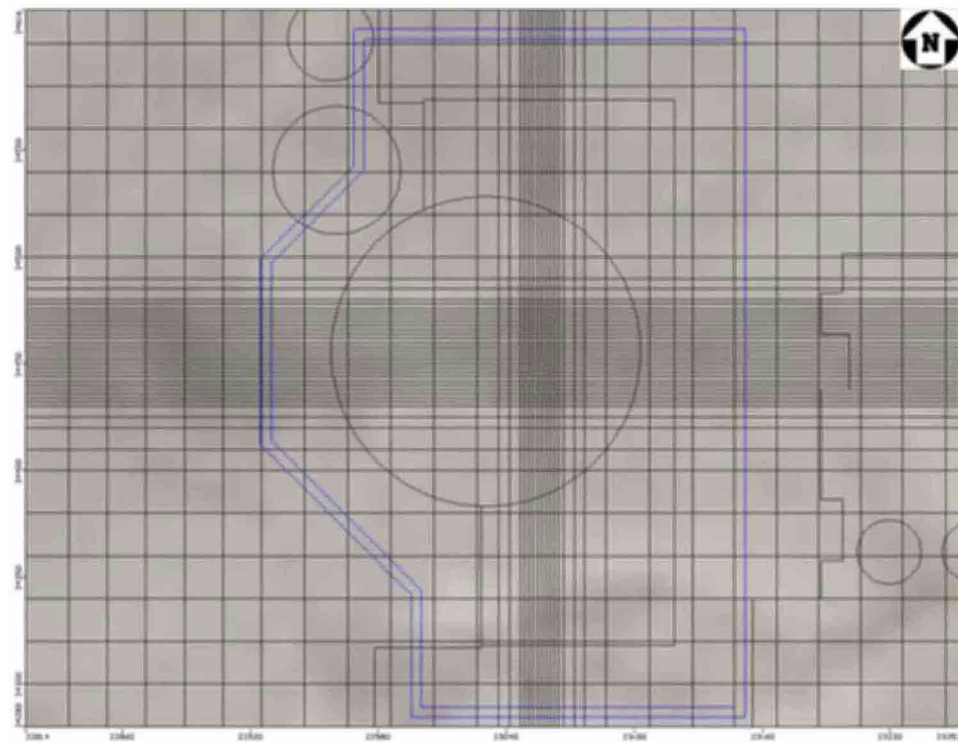
Figure 2CC-222 Grid Refinement in Vicinity of Unit 7 Reactor Footprint
