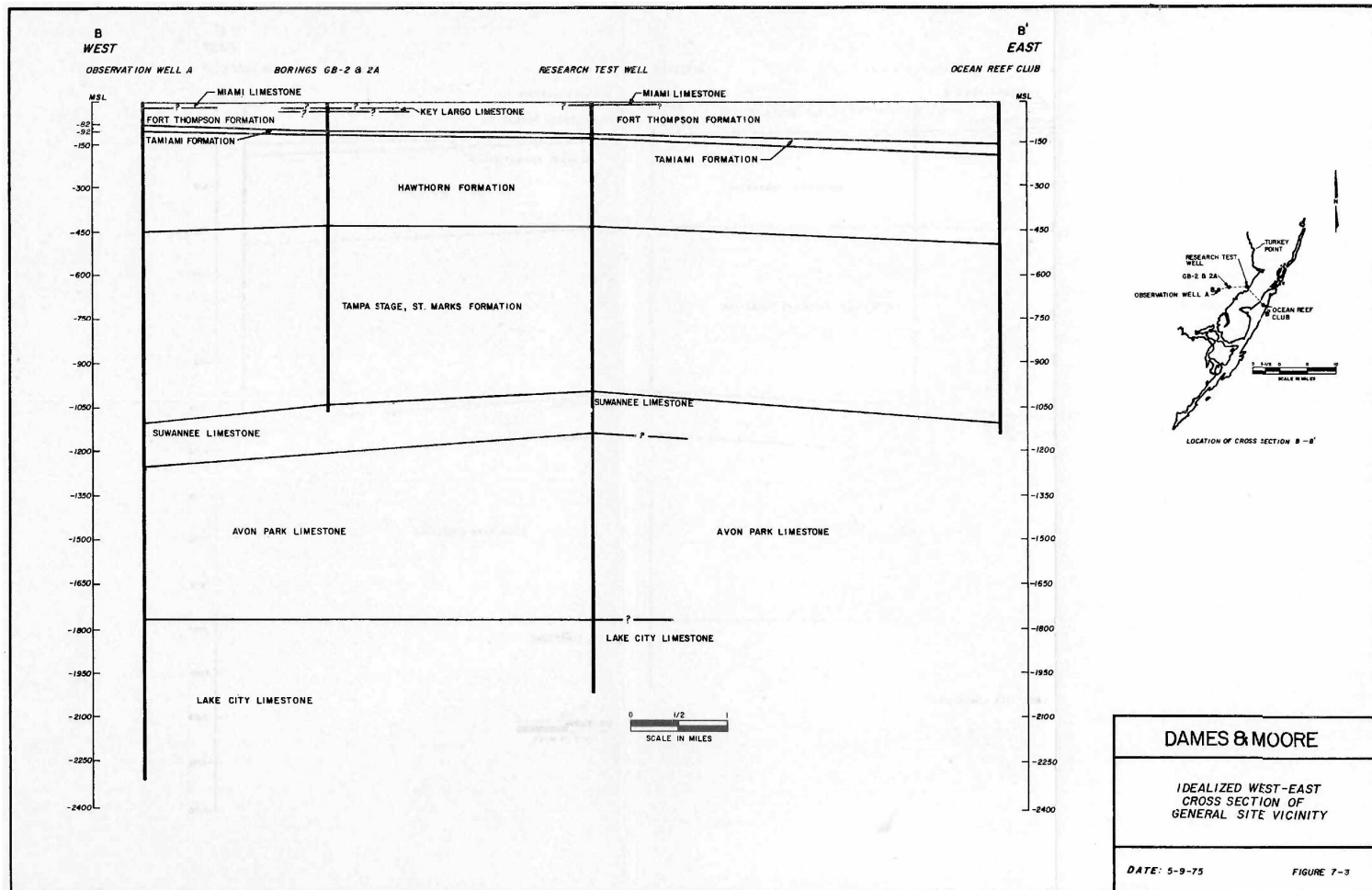
Figure 2CC-203 West-East Cross Section of Site Vicinity
