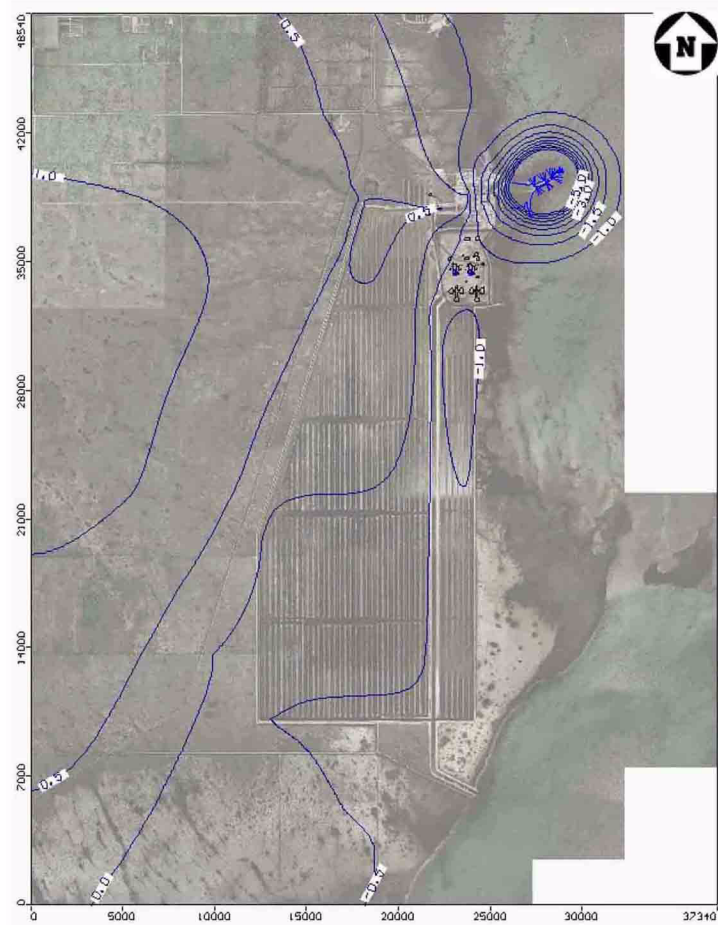
Figure 2CC-233 Groundwater Contours within Key Largo Limestone During Radial Collector Well Simulations
