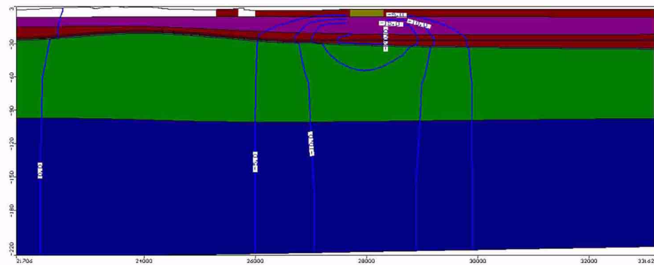
Figure 2CC-235 Results of Radial Collector Well Simulation
