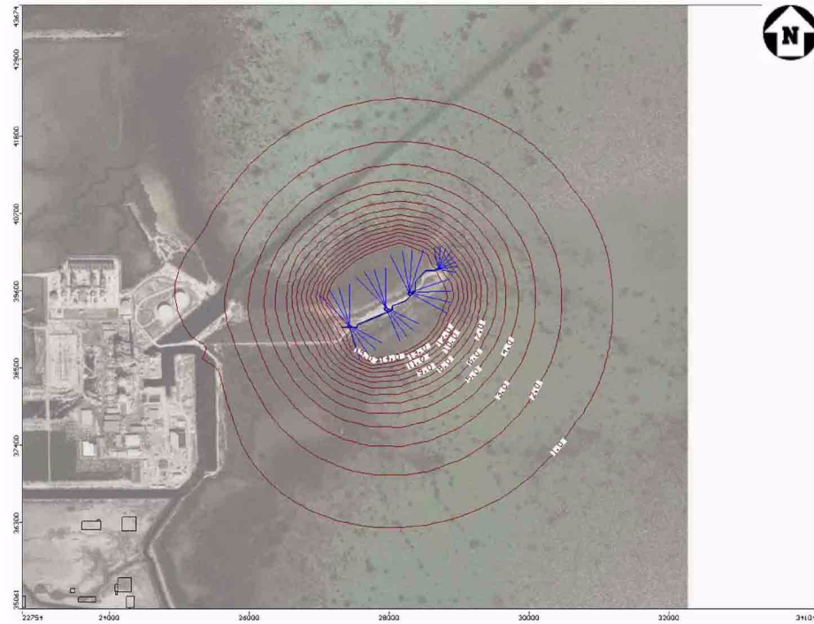
Figure 2CC-239 Drawdown within the Pumped Layer (Key Largo Limestone)
