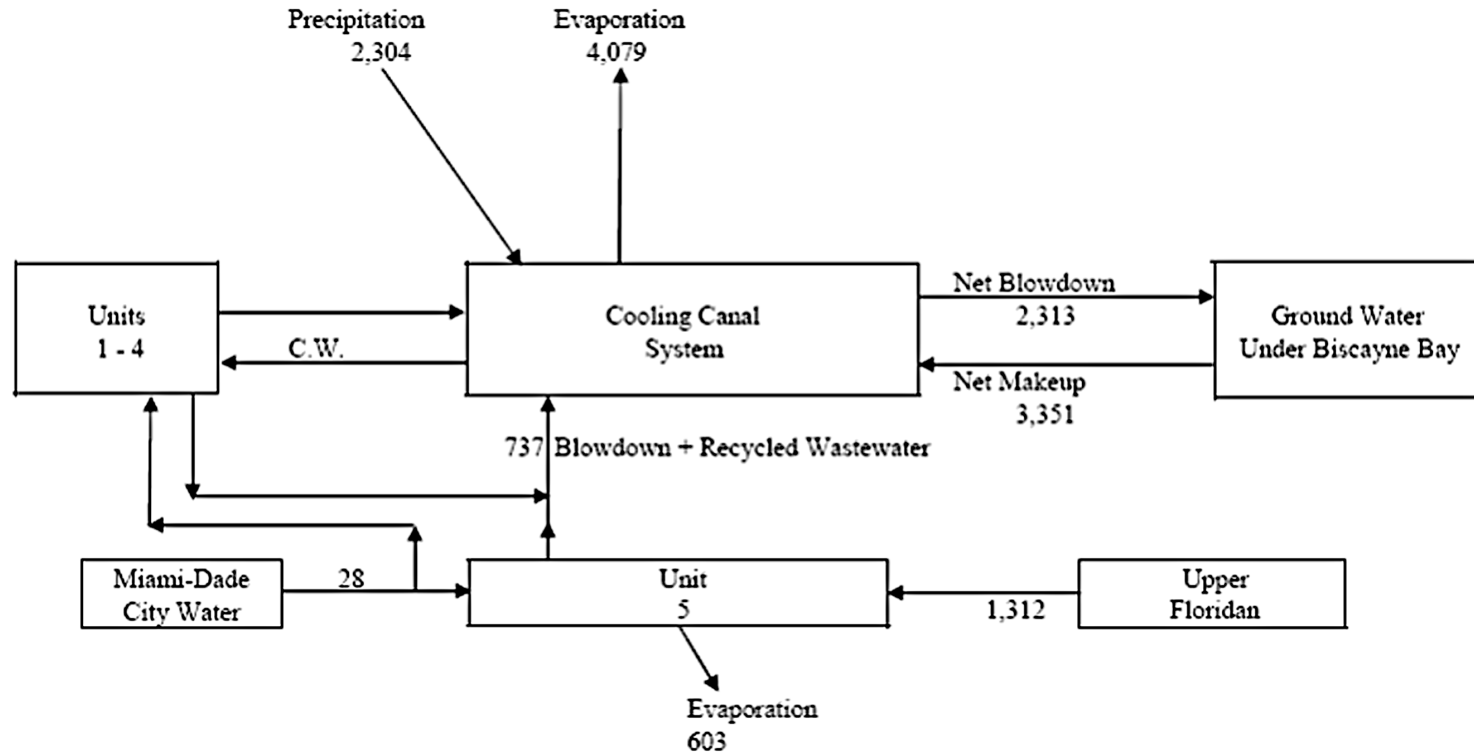
Figure 2CC-213 Cooling Canals Water Balance
