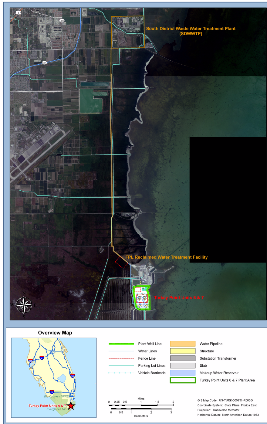
PTN COL 2.4-3 Figure 2.4.11-201 Location of Reclaimed Water Source and Pipeline Route
