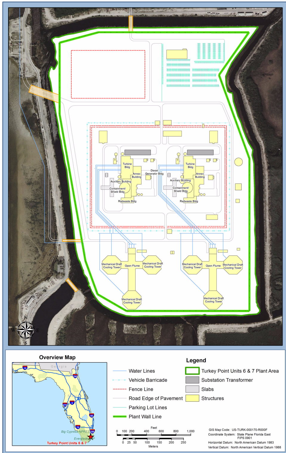
Figure 2.4.1-204 General Arrangement of Units 6 & 7
